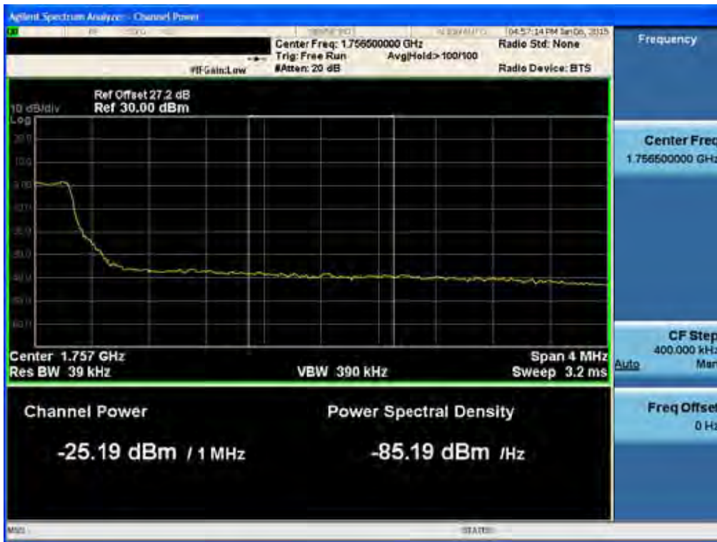
BAND 4. Upper Extended Band Edge Plot (5M BW Ch.20375 QPSK_RB25) -3
