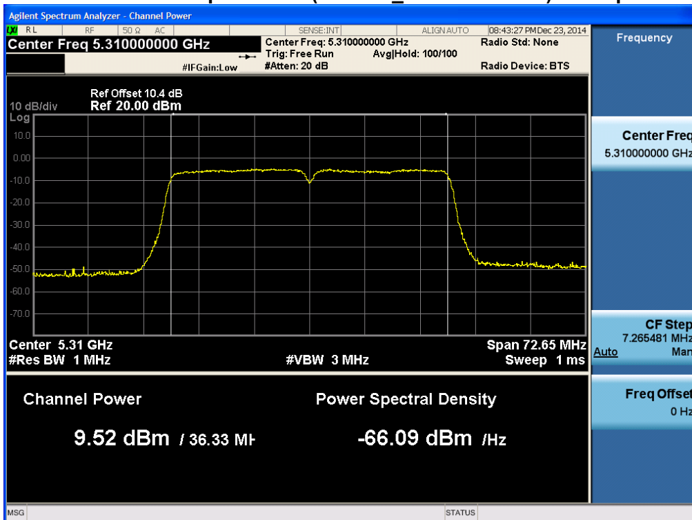
Conducted Output Power (802.11n_40M BW-CH 62) 54 Mbps
