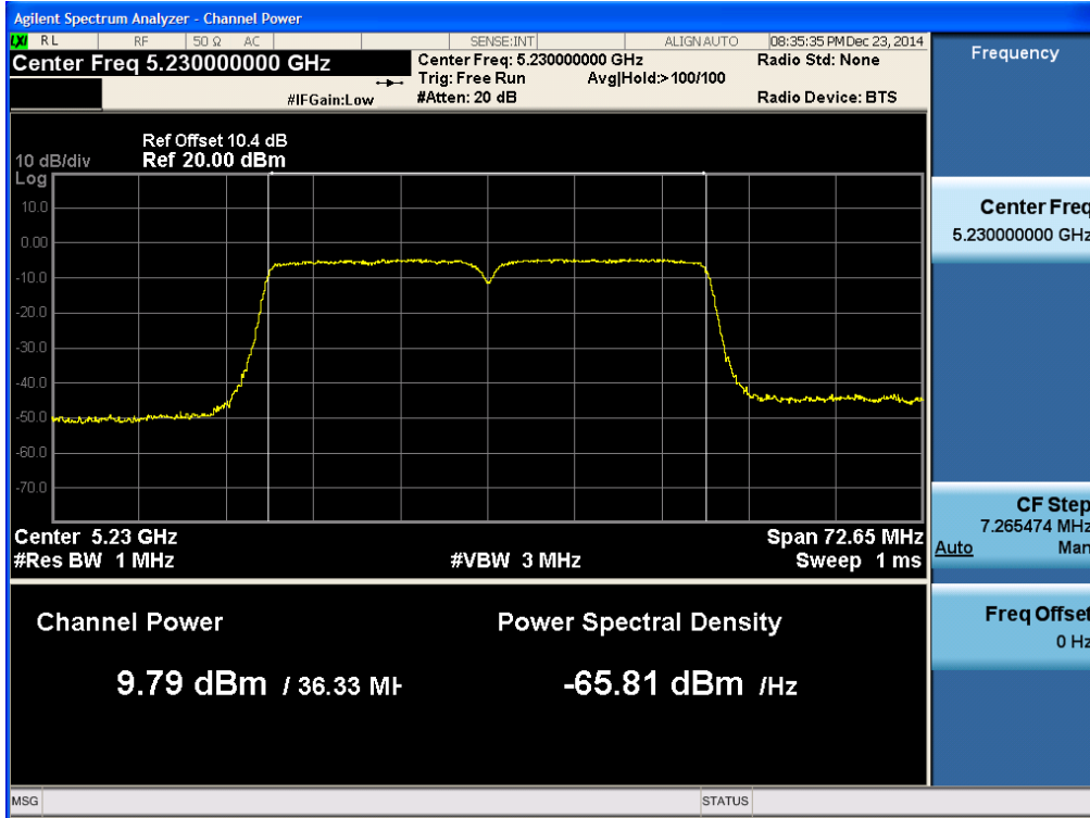
Conducted Output Power (802.11n_40M BW-CH 46) 81 Mbps
