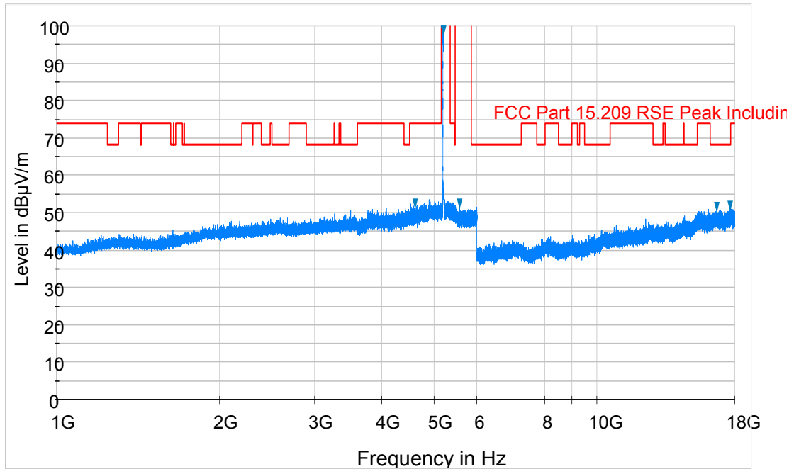
Plot 6-76. Radiated Spurious Plot above 1GHz (802.11a – U1 Ch. 40, Ant. Pol. H)
