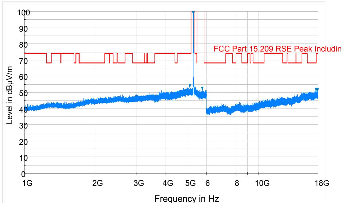
Plot 6-79. Radiated Spurious Plot above 1GHz (802.11a – U2A Ch. 56, Ant. Pol. V)
