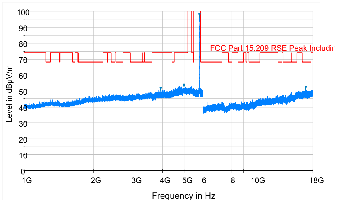
Plot 6-83. Radiated Spurious Plot above 1GHz (802.11a – U3 Ch. 157, Ant. Pol. V)
