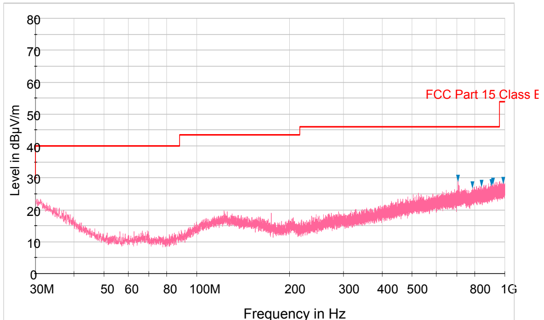
Plot 6-108. Radiated Spurious Plot below 1GHz (802.11a – U3 Ch. 157, Ant. Pol. V)
