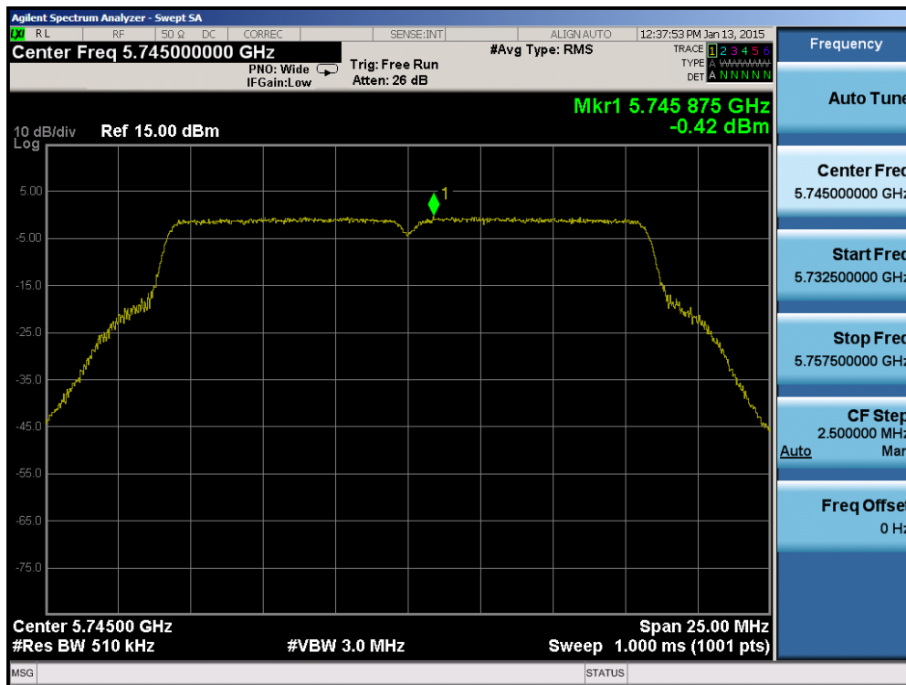
Plot 6-67. Power Spectral Density Plot (802.11a (UNII Band 3) – Ch. 149)
