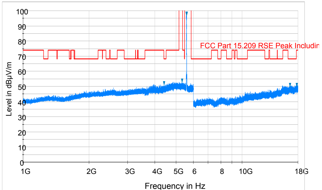
Plot 6-81. Radiated Spurious Plot above 1GHz (802.11a – U2C Ch. 116, Ant. Pol. V)
