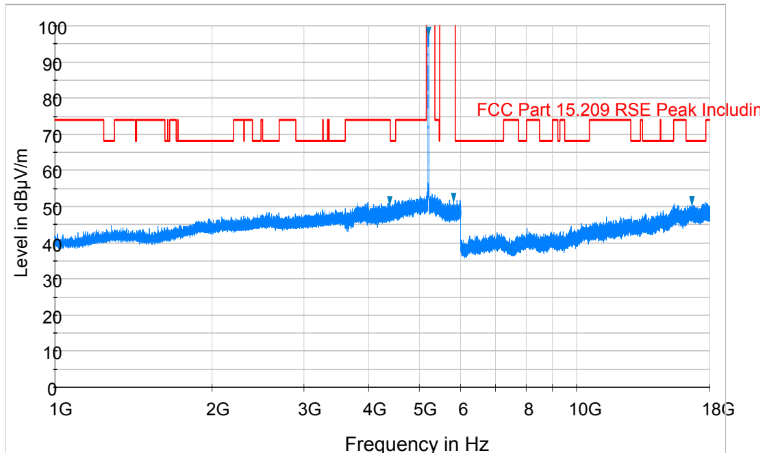
Plot 6-77. Radiated Spurious Plot above 1GHz (802.11a – U1 Ch. 40, Ant. Pol. V)
