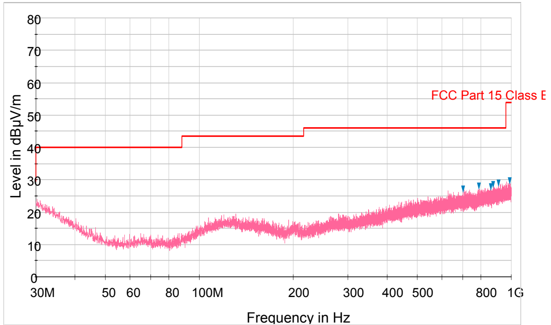
Plot 6-107. Radiated Spurious Plot below 1GHz (802.11a – U3 Ch. 157, Ant. Pol. H)
