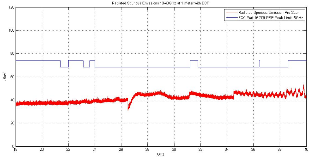
Plot 6-84. Radiated Spurious Plot above 18GHz (802.11a – Ant. Pol. H)
