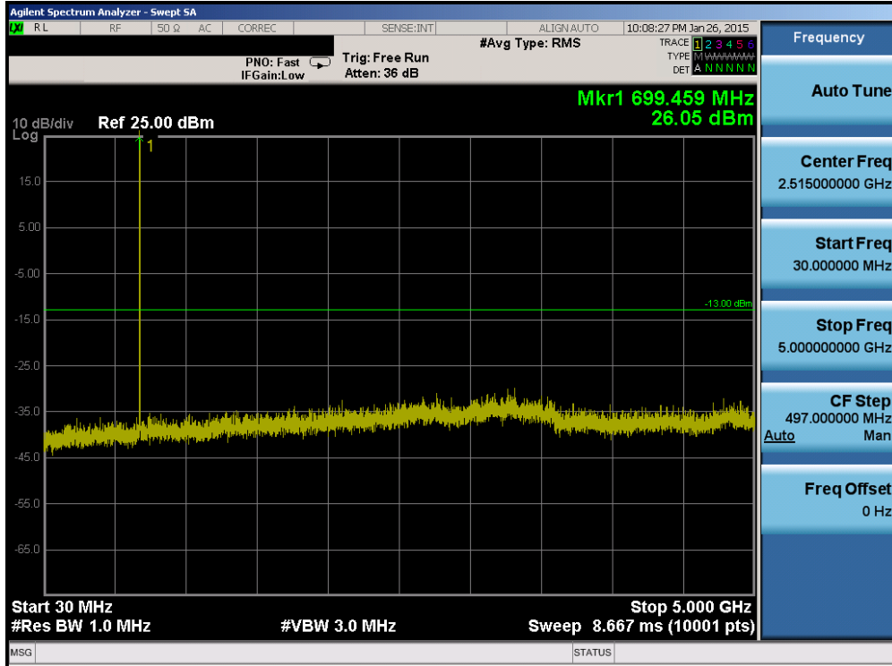
Plot 6-49. Conducted Spurious Plot (Band 12 – 3.0MHz QPSK – RB Size 1, RB Offset 0 – Low Channel)
