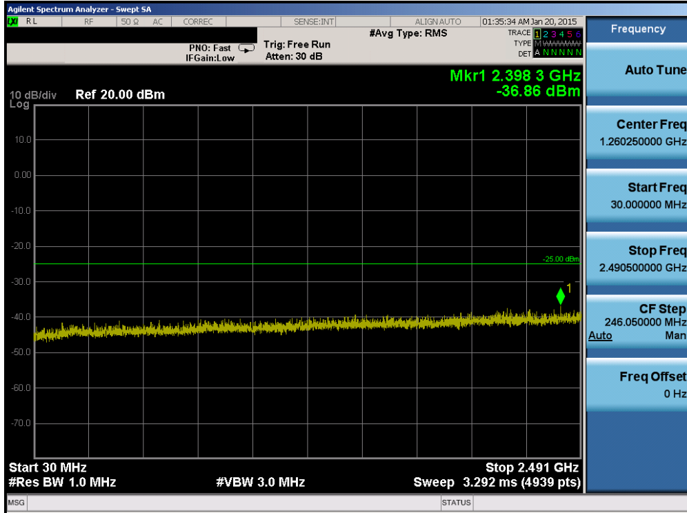
Plot 6-71. Conducted Spurious Plot (Band 7 – 10.0MHz QPSK – RB Size 1, RB Offset 0– Low Channel)
