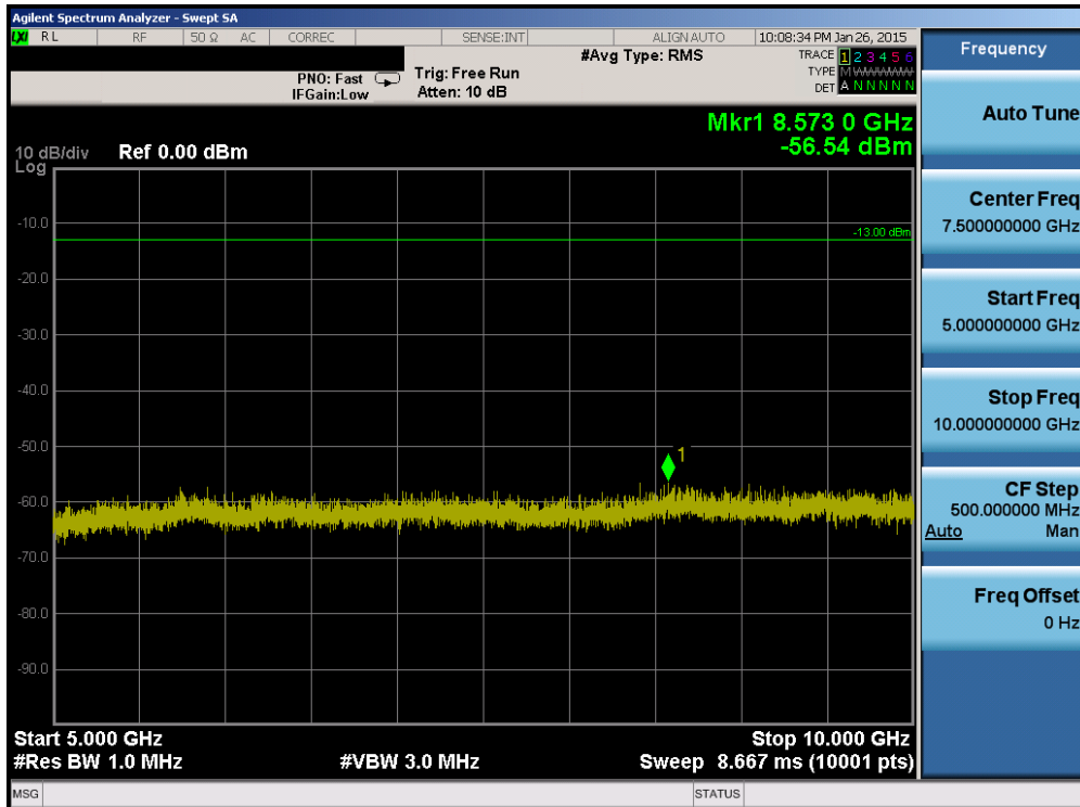
Plot 6-50. Conducted Spurious Plot (Band 12 – 3.0MHz QPSK – RB Size 1, RB Offset 0 – Low Channel)
