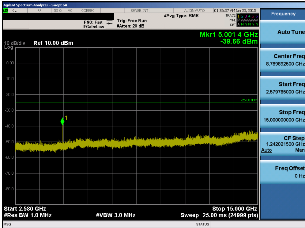
Plot 6-72. Conducted Spurious Plot (Band 7 – 10.0MHz QPSK – RB Size 1, RB Offset 0 – Low Channel)
