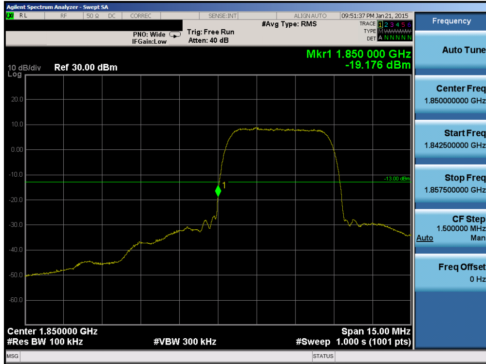
Plot 6-43. Band Edge Plot (PCS WCDMA Mode – Ch. 9262)
