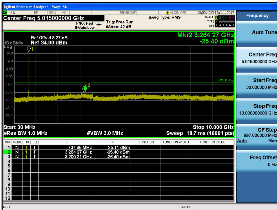
LTE Band 17 / 10MHz / 64QAM - RB Size/Offset (25/0) – High Channel
