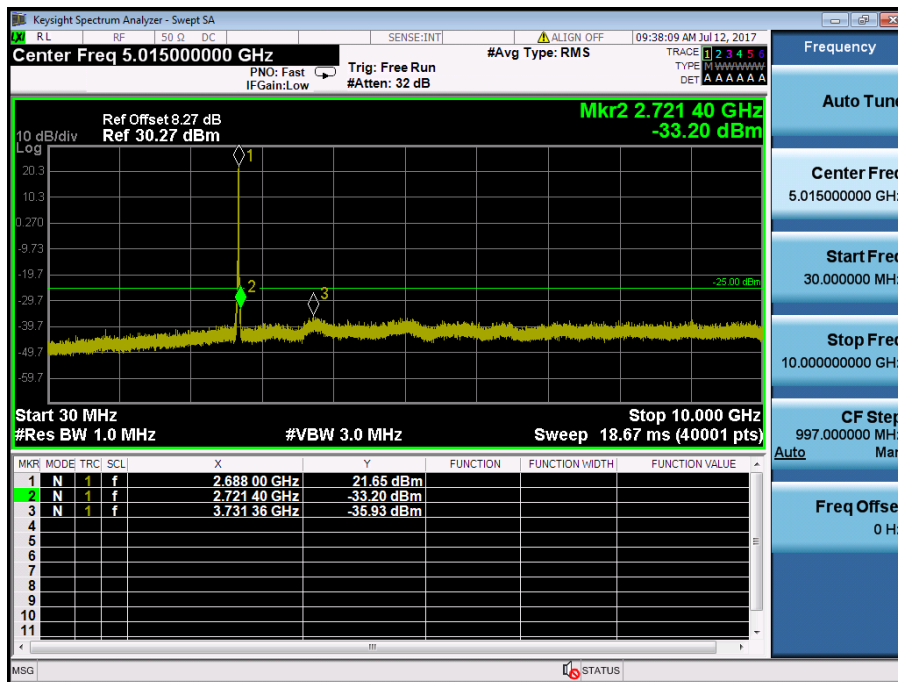
LTE Band 41 / 10MHz / QPSK - RB Size/Offset (25/0) – High Channel
