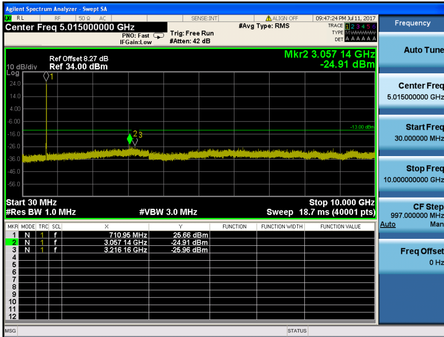
LTE Band 17 / 10MHz / 64QAM - RB Size/Offset (25/12) – Low Channel
