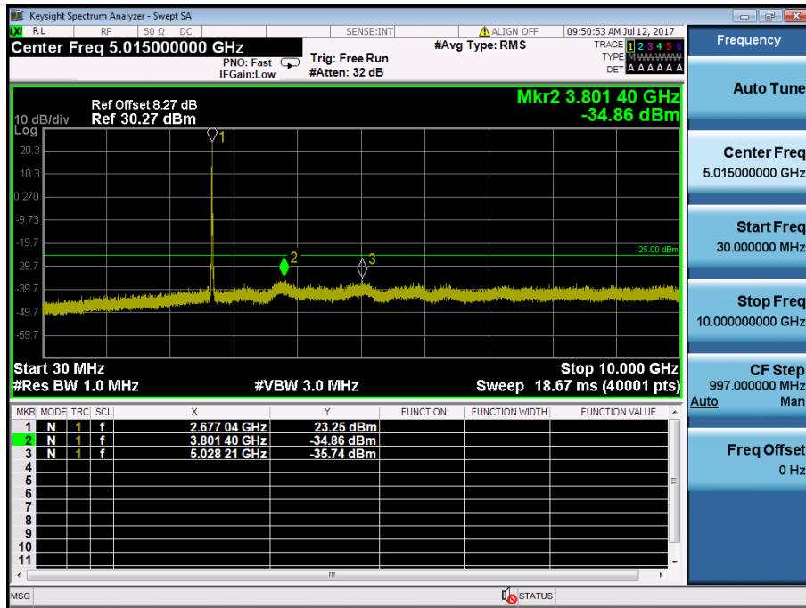
LTE Band 41 / 15MHz / QPSK - RB Size/Offset (36/0) – High Channel
