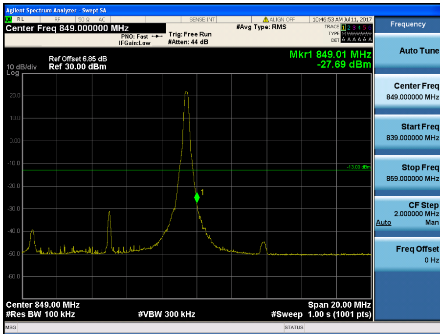
LTE Band 5 / 10MHz / 64QAM - RB Size/Offset (1/49)
