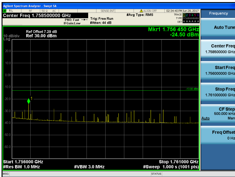
LTE Band 4 / 5MHz / 64QAM - RB Size/Offset (1/12)
