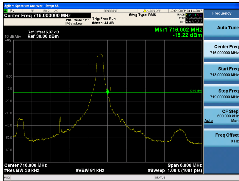
LTE Band 12 / 3MHz / QPSK - RB Size/Offset (1/14)
