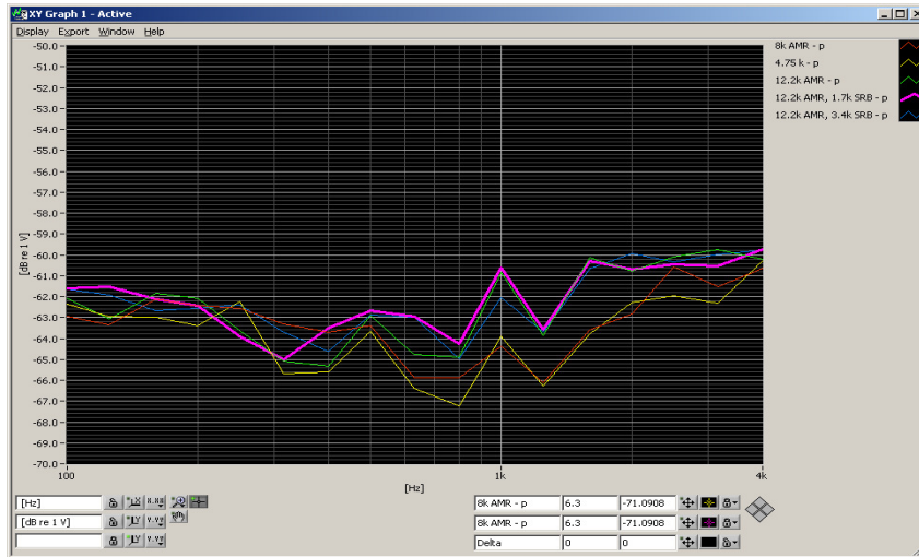
Figure 5-1 UMTS Audio Band Magnetic Noise
