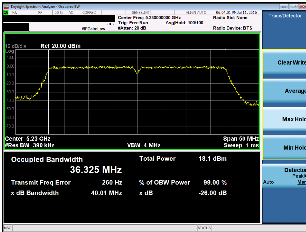
Plot 7-37. 26dB Bandwidth Plot (40MHz BW 802.11n (UNII Band 1) – Ch. 46)
