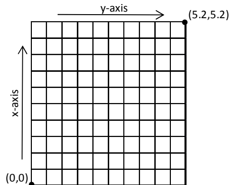
Figure 4-12 Measurement Grid
