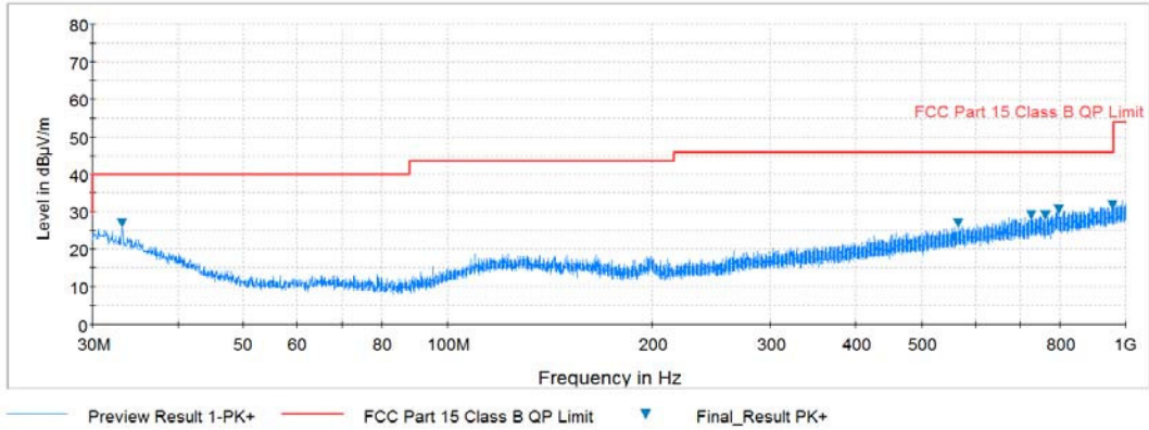
Plot 7-29. Radiated Spurious Plot below 1GHz (Pol. H)
