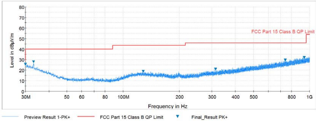
Plot 7-31. Radiated Spurious Plot below 1GHz (Pol. H)
