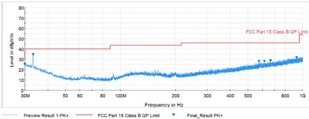
Plot 7-32. Radiated Spurious Plot below 1GHz (Pol. V)
