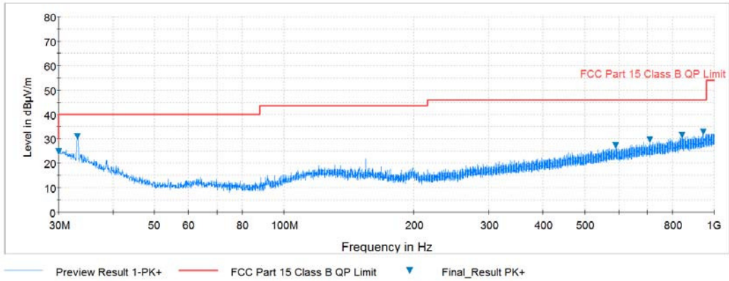
Plot 7-30. Radiated Spurious Plot below 1GHz (Pol. V)
