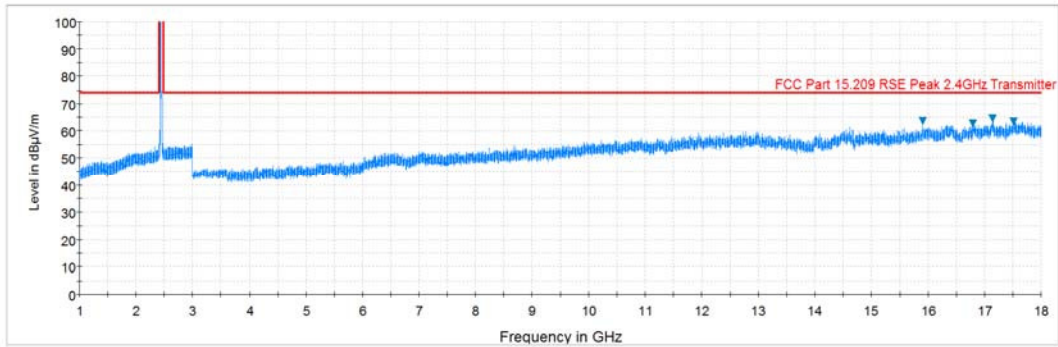
Plot 7-11. Radiated Spurious Plot above 1GHz (802.11b – Ch. 6, Ant. Pol. H)
