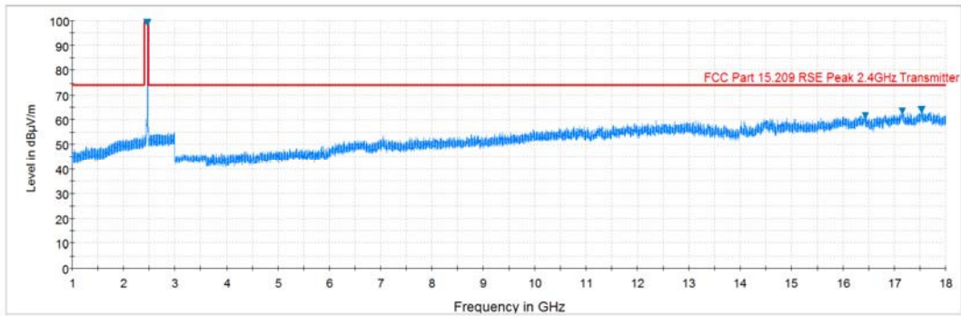
Plot 7-2. Radiated Spurious Plot above 1GHz (802.11b – Ch. 1, Ant. Pol. V)
