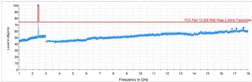
Plot 7-10. Radiated Spurious Plot above 1GHz (802.11b – Ch. 1, Ant. Pol. V)
