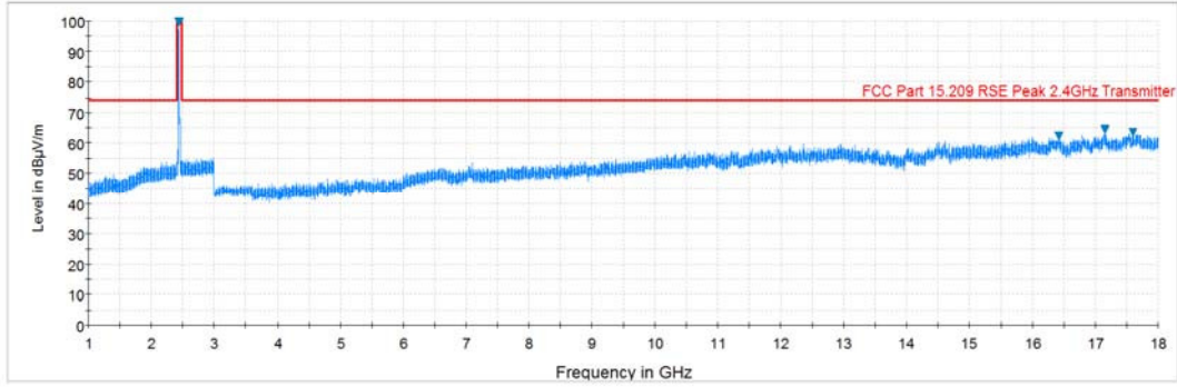
Plot 7-12. Radiated Spurious Plot above 1GHz (802.11b – Ch. 6, Ant. Pol. V)
