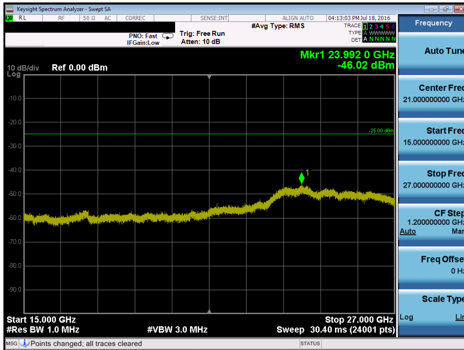
Plot 7-100. Conducted Spurious Plot (Band 7 – 5.0MHz QPSK – RB Size 1, RB Offset 0 – Low Channel)
