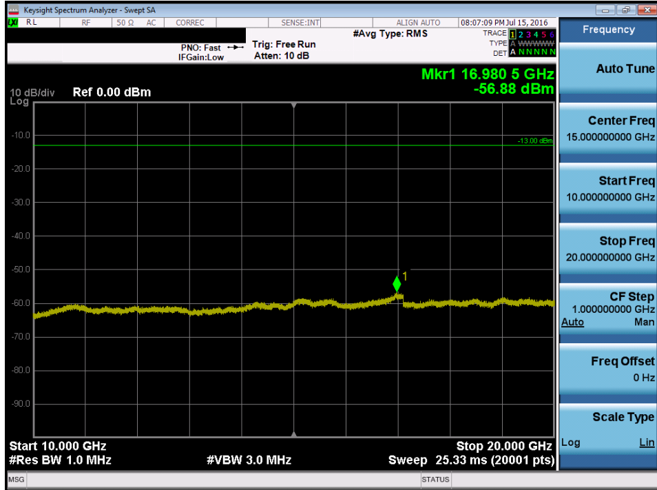
Plot 7-79. Conducted Spurious Plot (Band 4/66 – 10.0MHz QPSK – RB Size 1, RB Offset 0 – High Channel)
