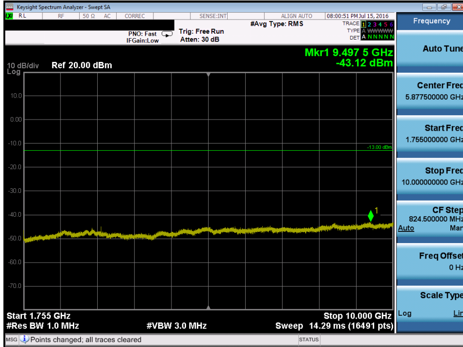
Plot 7-75. Conducted Spurious Plot (Band 4/66 – 10.0MHz QPSK – RB Size 1, RB Offset 0 – Mid Channel)
