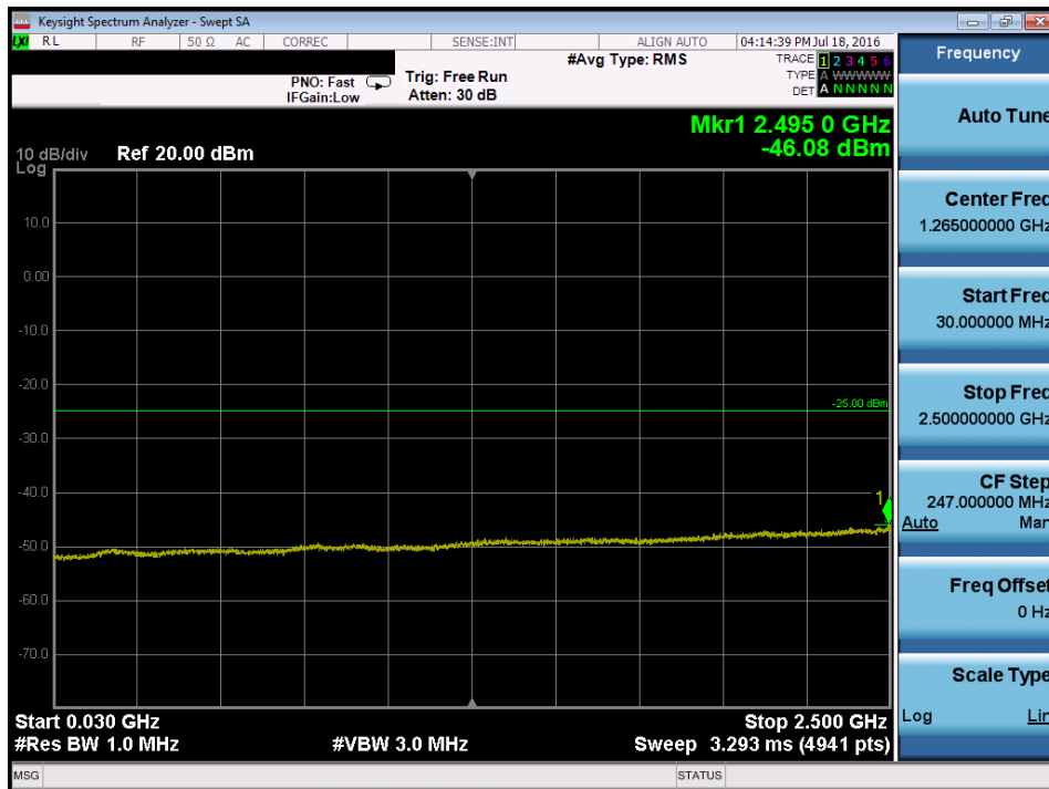
Plot 7-104. Conducted Spurious Plot (Band 7 – 5.0MHz QPSK – RB Size 1, RB Offset 0 – High Channel)
