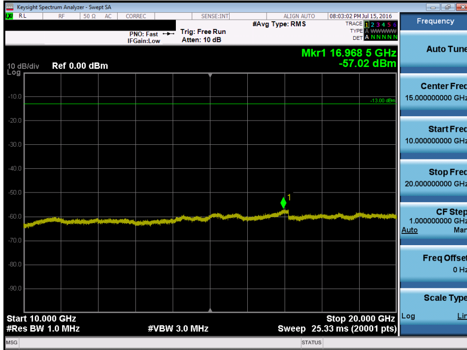
Plot 7-73. Conducted Spurious Plot (Band 4/66 – 10.0MHz QPSK – RB Size 1, RB Offset 0 – Low Channel)
