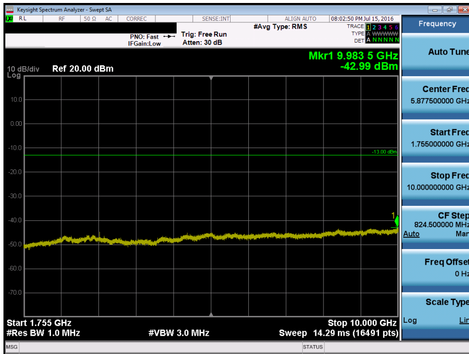
Plot 7-72. Conducted Spurious Plot (Band 4/66 – 10.0MHz QPSK – RB Size 1, RB Offset 0 – Low Channel)
