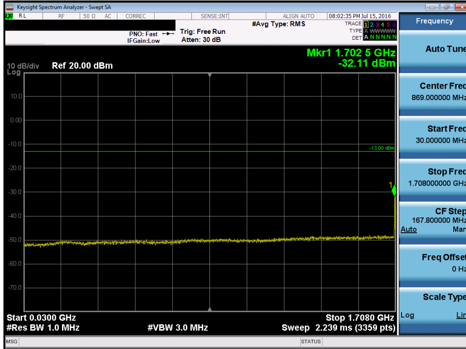
Plot 7-71. Conducted Spurious Plot (Band 4/66 – 10.0MHz QPSK – RB Size 1, RB Offset 0– Low Channel)
