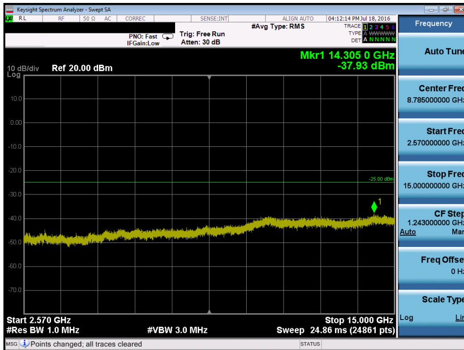
Plot 7-102. Conducted Spurious Plot (Band 7 – 5.0MHz QPSK – RB Size 1, RB Offset 0 – Mid Channel)
