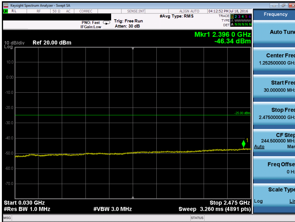
Plot 7-98. Conducted Spurious Plot (Band 7 – 5.0MHz QPSK – RB Size 1, RB Offset 0 – Low Channel)
