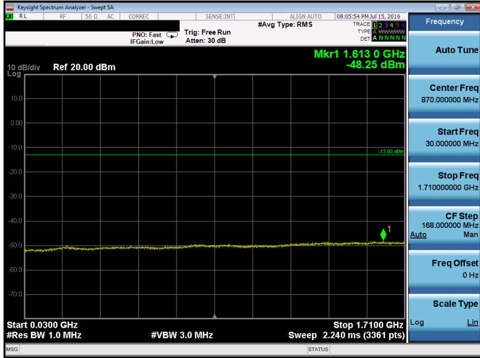
Plot 7-77. Conducted Spurious Plot (Band 4/66 – 10.0MHz QPSK – RB Size 1, RB Offset 0 – High Channel)
