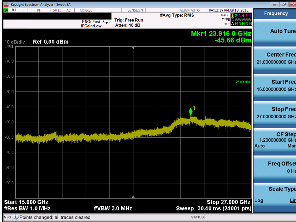
Plot 7-103. Conducted Spurious Plot (Band 7 – 5.0MHz QPSK – RB Size 1, RB Offset 0 – Mid Channel)
