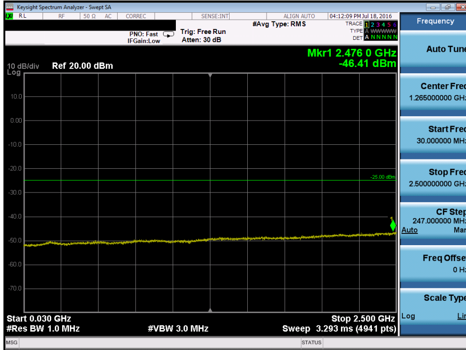
Plot 7-101. Conducted Spurious Plot (Band 7 – 5.0MHz QPSK – RB Size 1, RB Offset 0 – Mid Channel)
