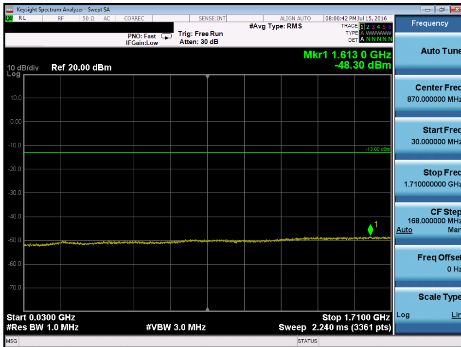
Plot 7-74. Conducted Spurious Plot (Band 4/66 – 10.0MHz QPSK – RB Size 1, RB Offset 0 – Mid Channel)
