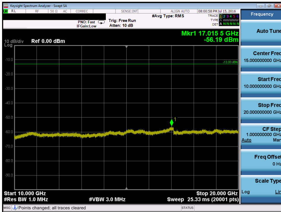
Plot 7-76. Conducted Spurious Plot (Band 4/66 – 10.0MHz QPSK – RB Size 1, RB Offset 0 – Mid Channel)
