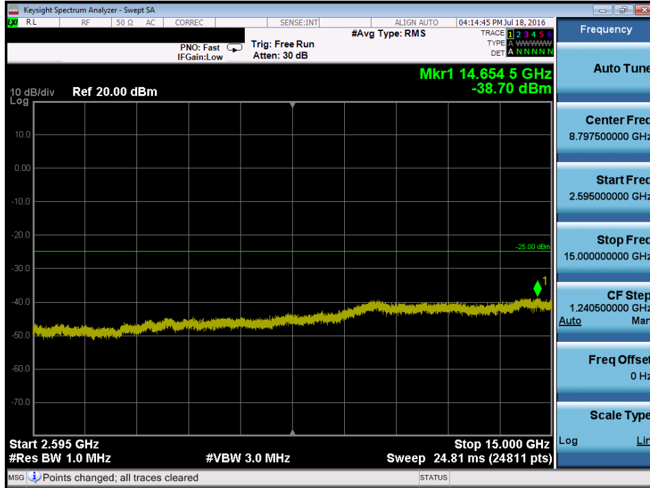
Plot 7-105. Conducted Spurious Plot (Band 7 – 5.0MHz QPSK – RB Size 1, RB Offset 0 – High Channel)
