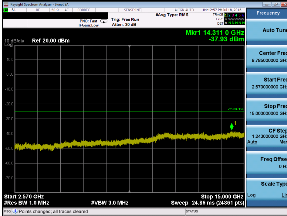
Plot 7-99. Conducted Spurious Plot (Band 7 – 5.0MHz QPSK – RB Size 1, RB Offset 0 – Low Channel)
