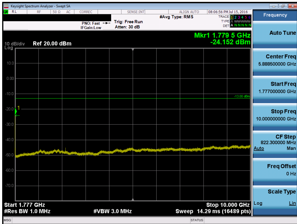
Plot 7-78. Conducted Spurious Plot (Band 4/66 – 10.0MHz QPSK – RB Size 1, RB Offset 0 – High Channel)
