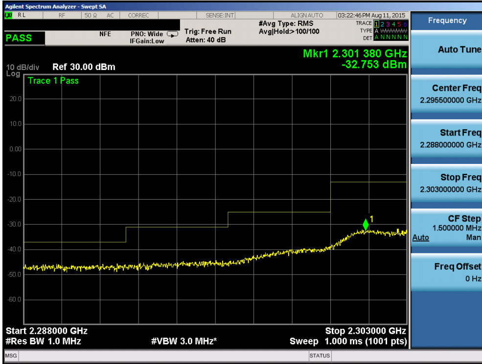
Plot 6-158. Lower Extended Band Edge Plot (Band 30 – 5.0MHz QPSK – RB Size 25)
