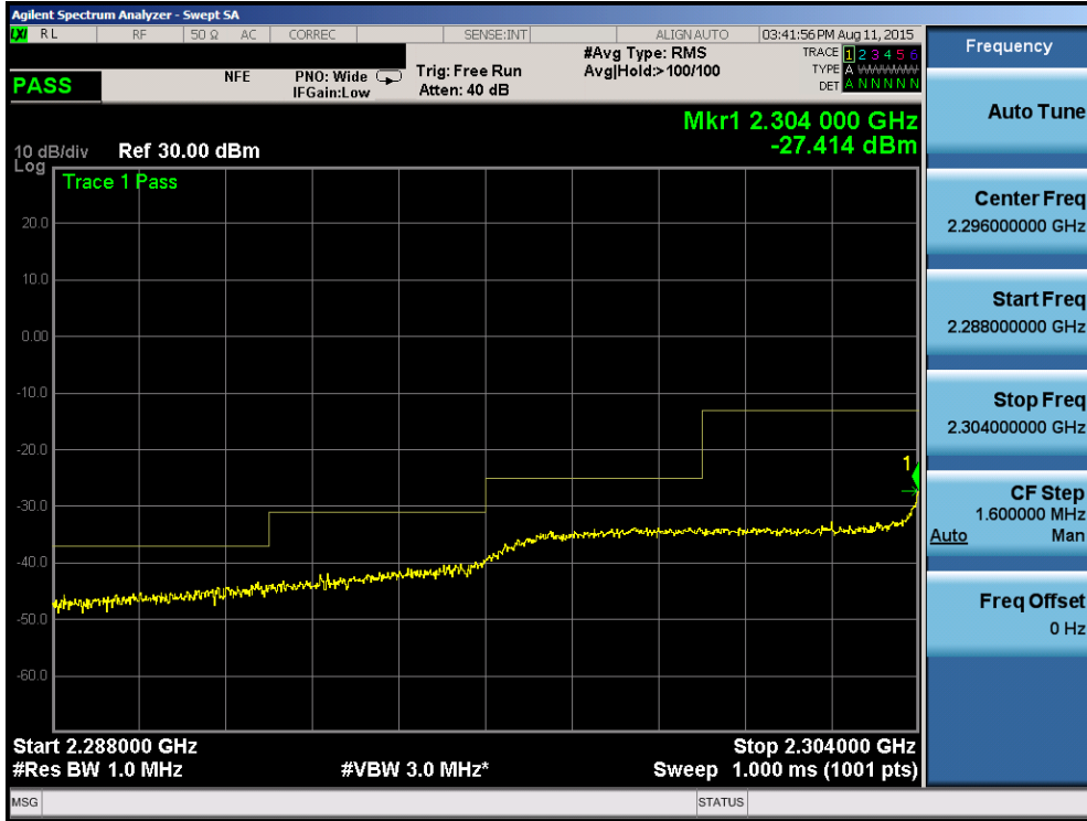
Plot 6-162. Lower Extended Band Edge Plot (Band 30 – 10.0MHz QPSK – RB Size 50)
