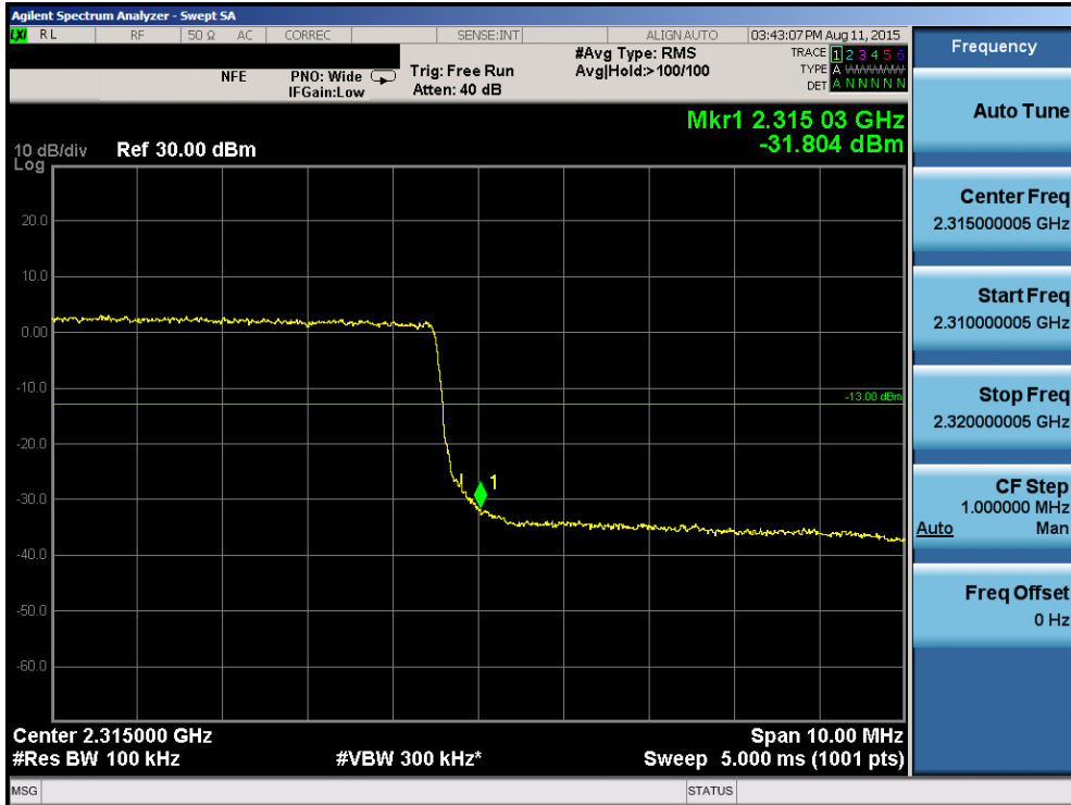
Plot 6-163. Upper Band Edge Plot (Band 30 – 10.0MHz QPSK – RB Size 50)
