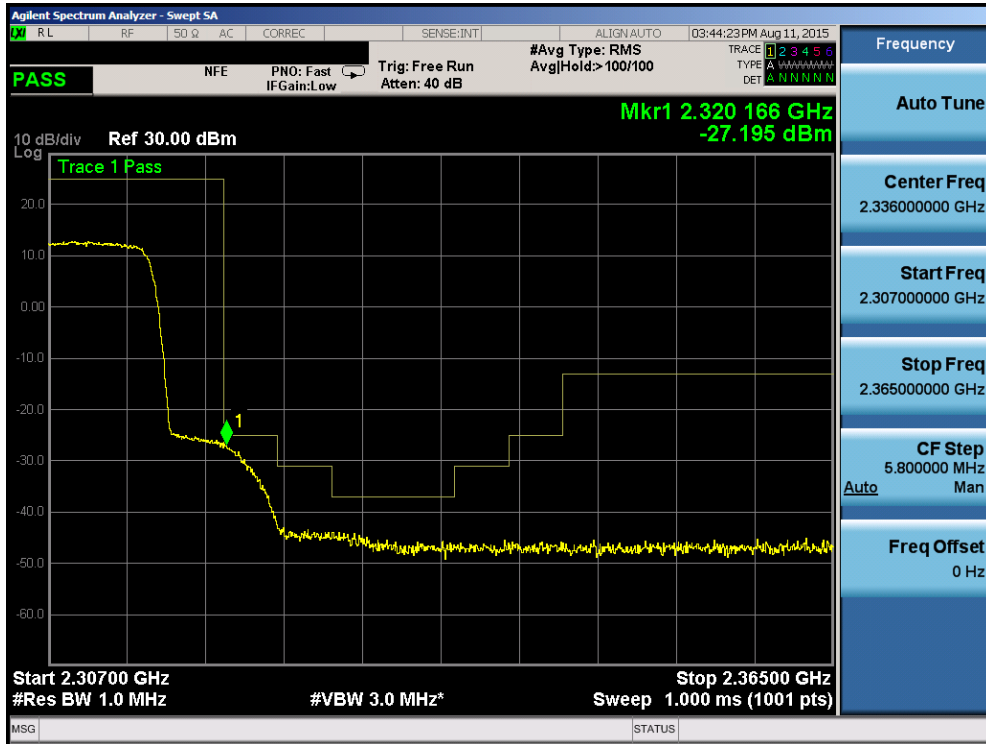
Plot 6-164. Upper Extended Band Edge Plot (Band 30 – 10.0MHz QPSK – RB Size 50)
