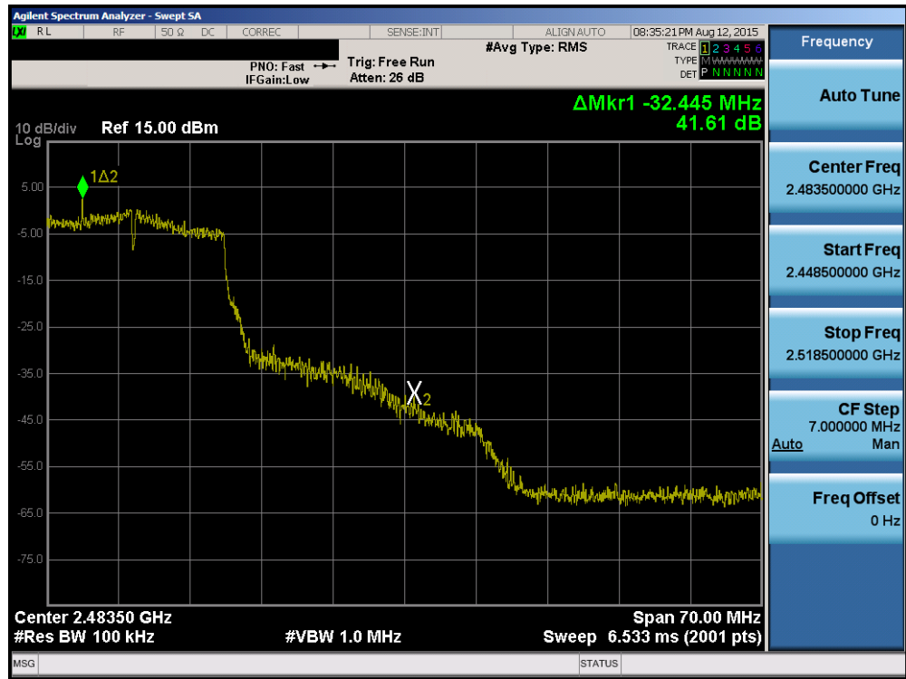
Plot 6-30. Band Edge Plot (802.11n (2.4GHz) - Ch.10)
