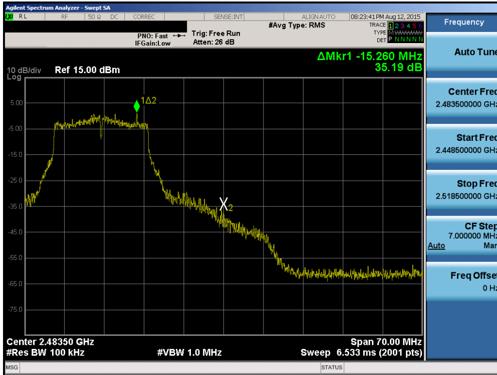
Plot 6-25. Band Edge Plot (802.11g – Ch. 11)
