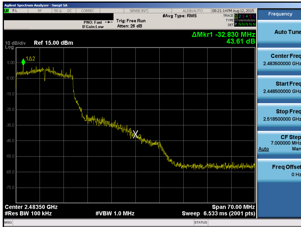
Plot 6-26. Band Edge Plot (802.11g - Ch. 10)
