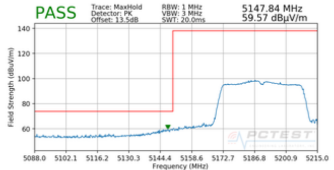
Plot 7-91. Radiated Lower Band Edge Plot (Peak – UNII Band 1)
