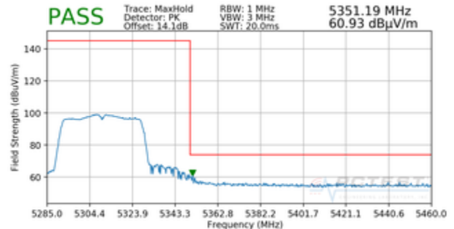
Plot 7-93. Radiated Upper Band Edge Plot (Peak – UNII Band 2A)
