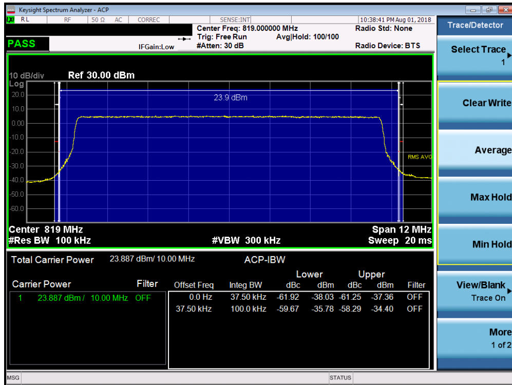
Plot 7-20. Channel Edge Plot (LTE Band 26, 10MHz QPSK – RB Size 50)
