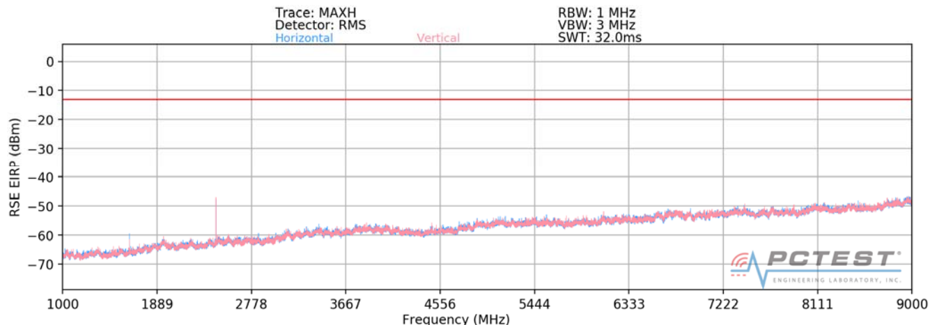
Plot 7-23. Radiated Spurious Plot above 1GHz (LTE Band 26)
