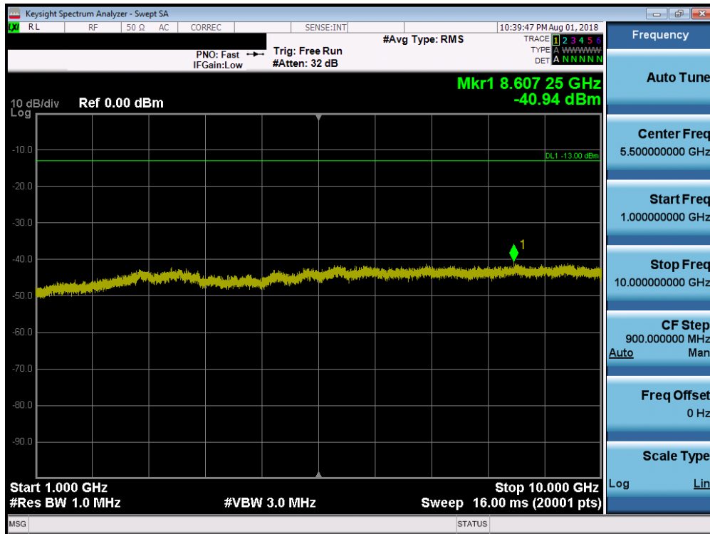
Plot 7-13. Conducted Spurious Plot (LTE Band 26, 15.0MHz QPSK – RB Size 1, RB Offset 0)
