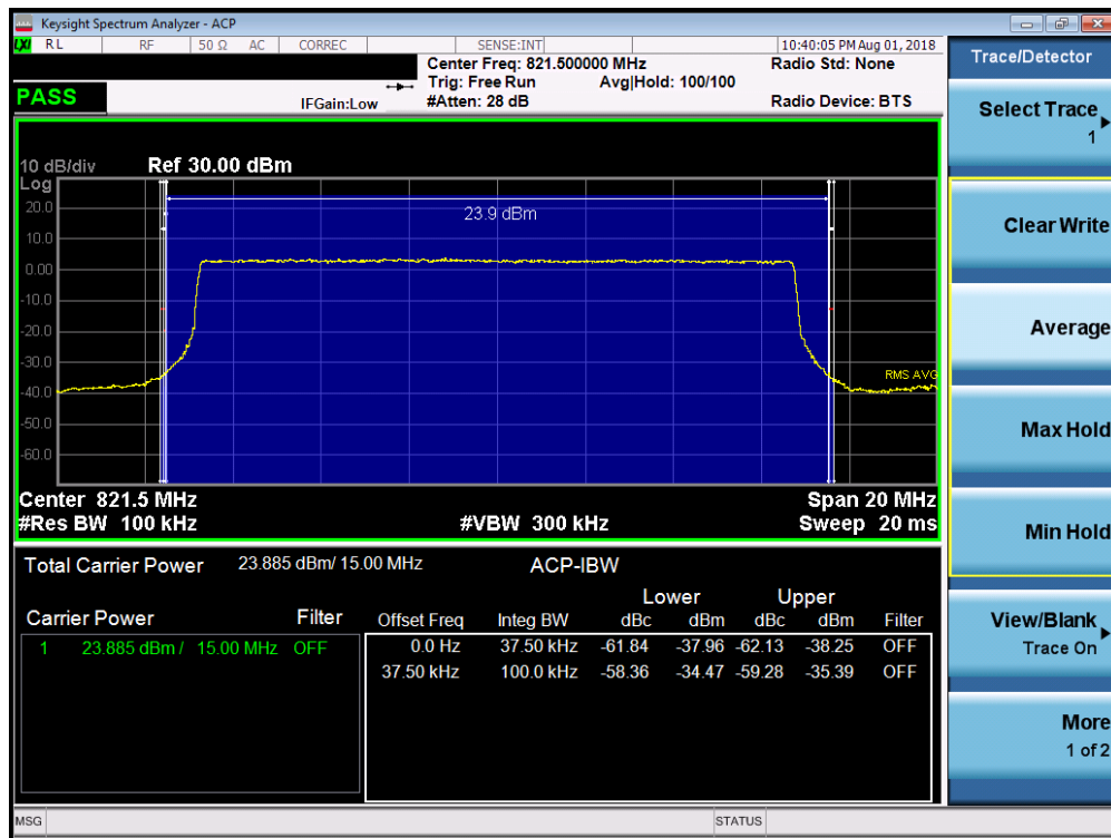
Plot 7-21. Channel Edge Plot (LTE Band 26, 15MHz QPSK – RB Size 75)
