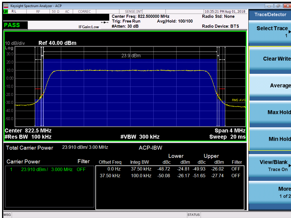
Plot 7-17. Channel Edge Plot (LTE Band 26, 3MHz QPSK – RB Size 15 – High Channel)
