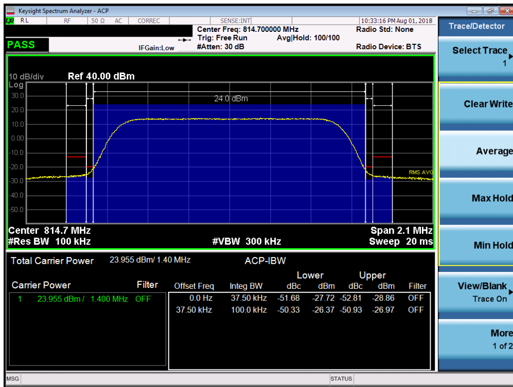
Plot 7-14. Channel Edge Plot (LTE Band 26, 1.4MHz QPSK – RB Size 6– Low Channel)
