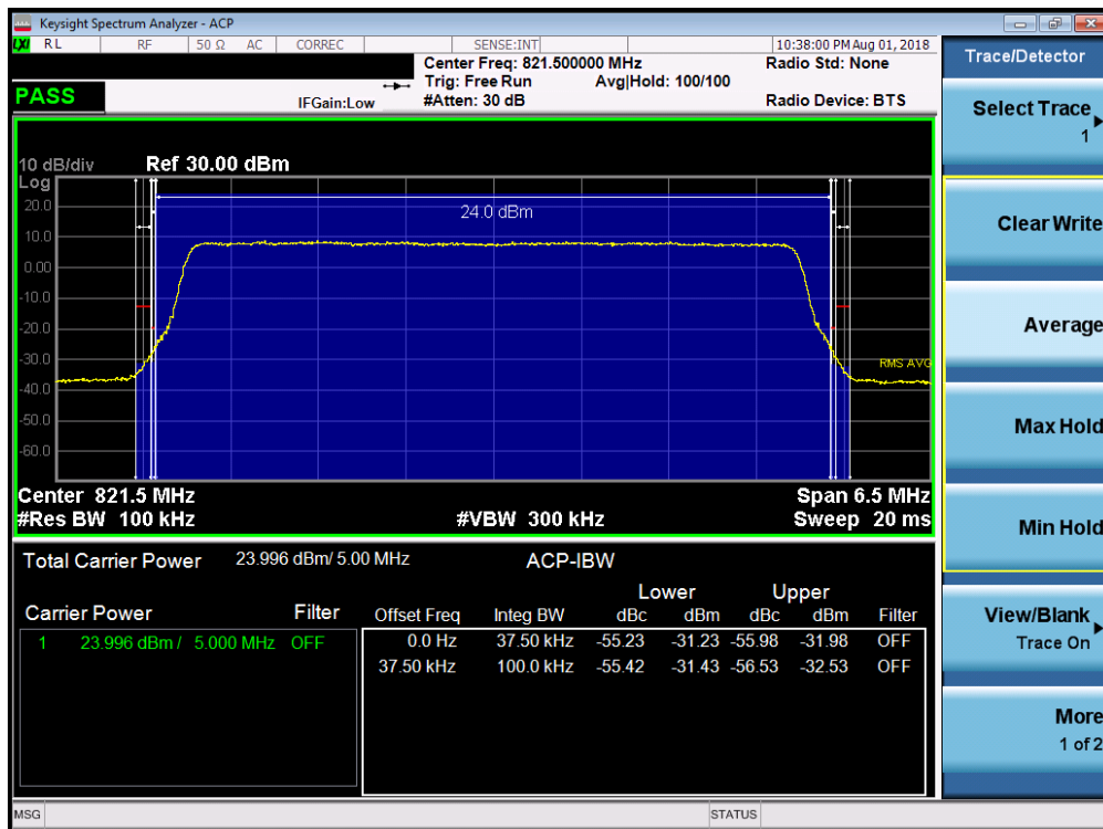
Plot 7-19. Channel Edge Plot (LTE Band 26, 5MHz QPSK – RB Size 25 – High Channel)
