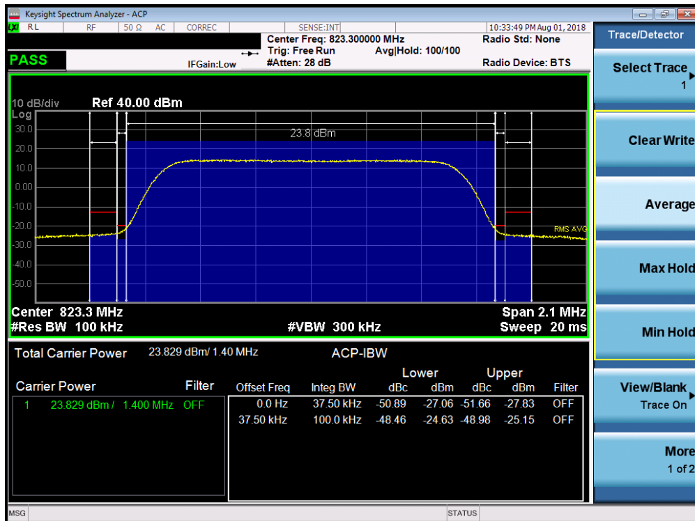
Plot 7-15. Channel Edge Plot (LTE Band 26, 1.4MHz QPSK – RB Size 6 – High Channel)
