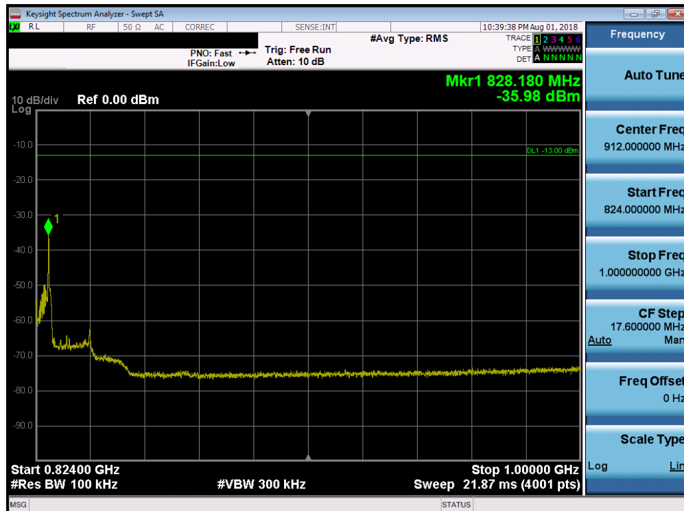
Plot 7-12. Conducted Spurious Plot (LTE Band 26, 15.0MHz QPSK – RB Size 1, RB Offset 0)
