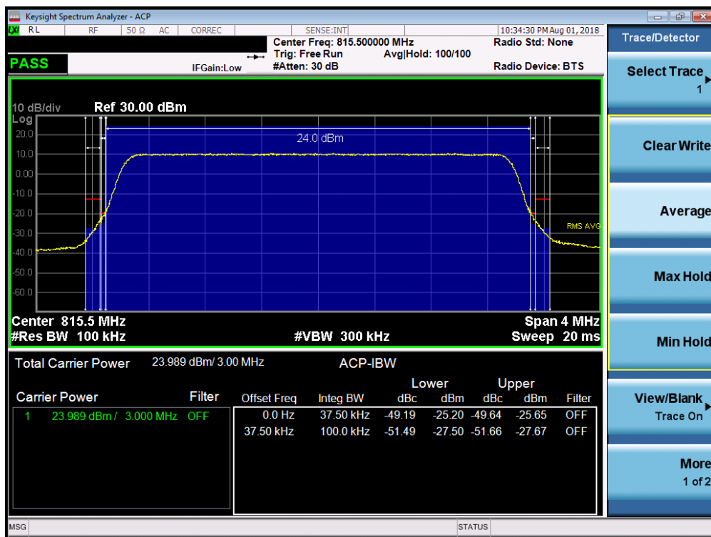
Plot 7-16. Channel Edge Plot (LTE Band 26, 3MHz QPSK – RB Size 15– Low Channel)
