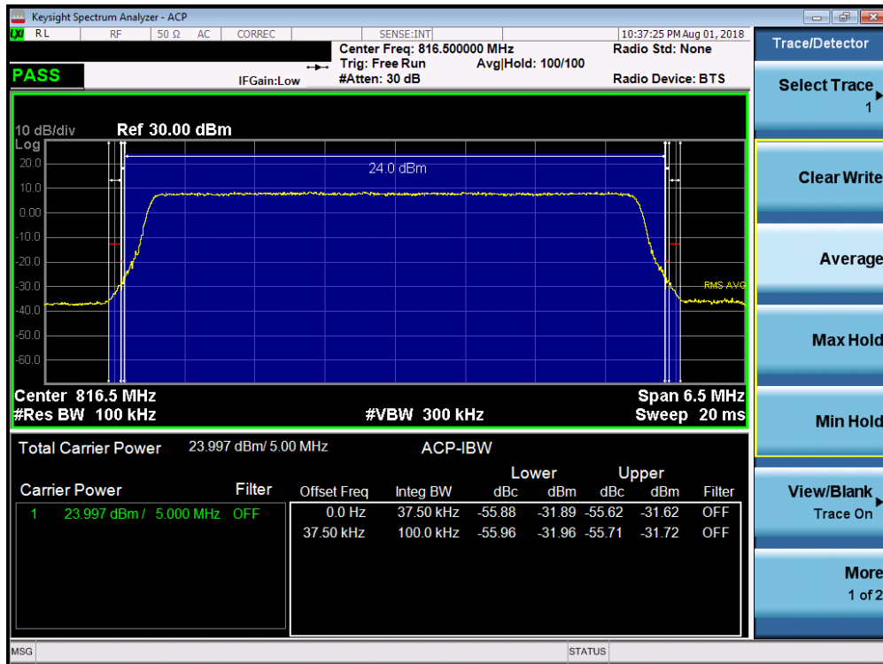
Plot 7-18. Channel Edge Plot (LTE Band 26, 5MHz QPSK – RB Size 25– Low Channel)
