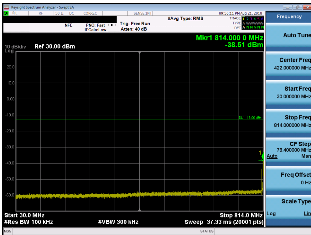
Plot 7-11. Conducted Spurious Plot (LTE Band 26, 15.0MHz QPSK – RB Size 1, RB Offset 0)
