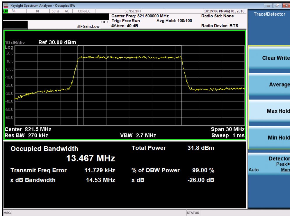
Plot 7-10. Occupied Bandwidth Plot (LTE Band 26, 15MHz 16-QAM – RB Size 75)
