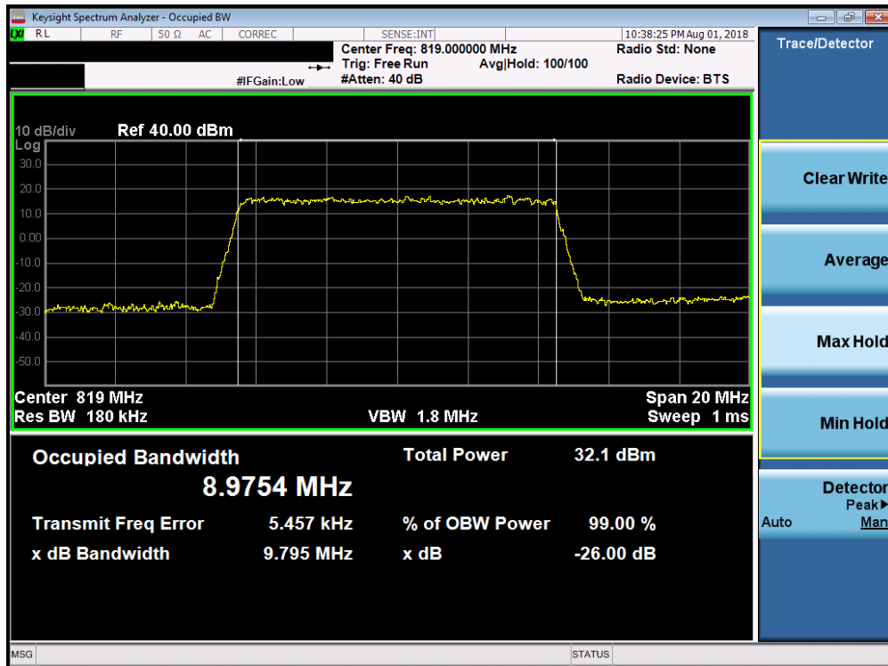
Plot 7-8. Occupied Bandwidth Plot (LTE Band 26, 10MHz 16-QAM – RB Size 50)
