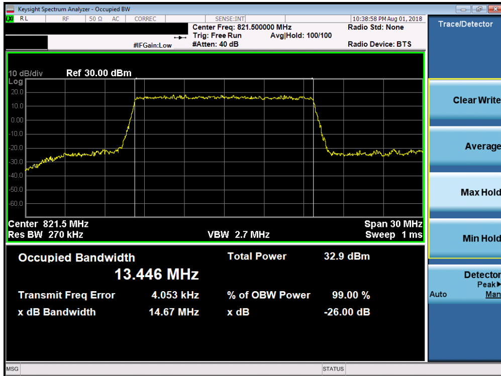
Plot 7-9. Occupied Bandwidth Plot (LTE Band 26, 15MHz QPSK – RB Size 75)
