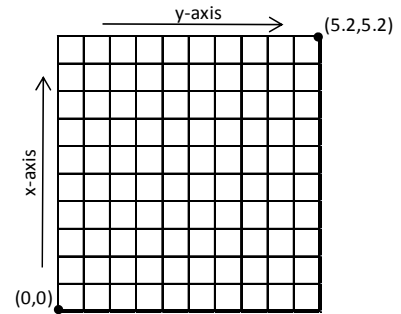
Figure 4-12 Measurement Grid
