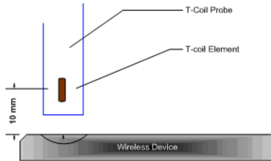
Figure 4-11 Measurement Distance
