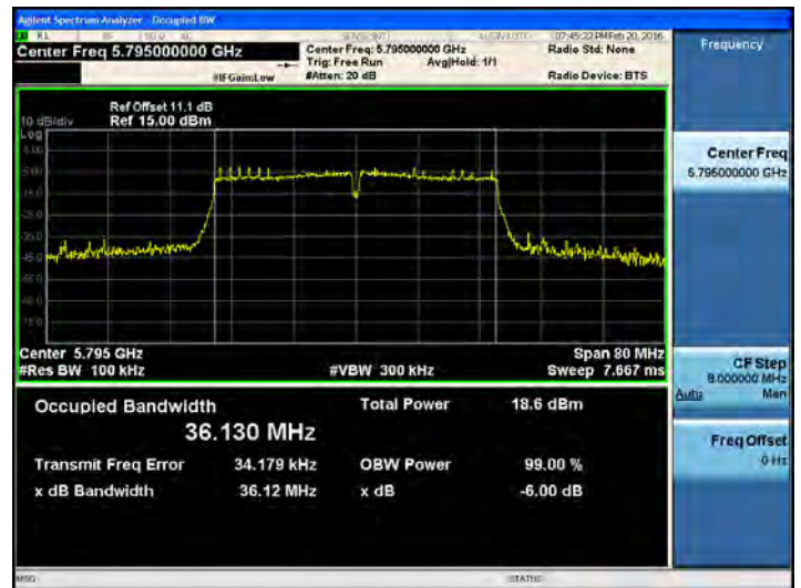
802.11ac_40 MHz BW UNII 3 BAND 6dB Bandwidth(CH.159)
