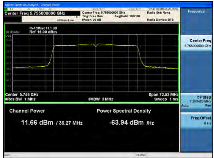
802.11ac_40 MHz BW UNII 3 BAND Average Power (5755 ~ 5795 MHz) CH 151 MCS1
