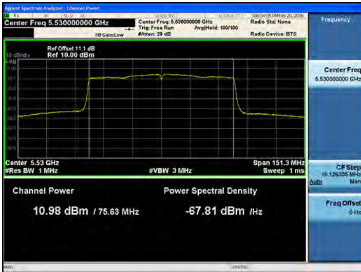
802.11ac_80 MHz BW UNII 2C BAND Average Power (5530 ~ 5690 MHz) CH 106MCS2
