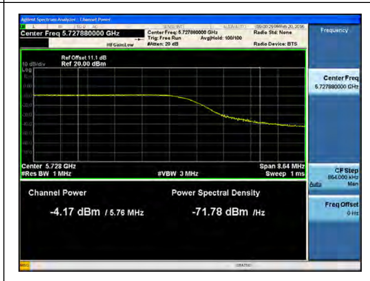
802.11ac_80MHz BW UNII 3 Band Average Power CH.138
