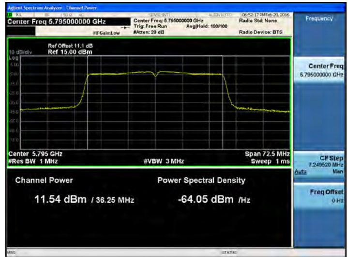
802.11n_40 MHz BW UNII 3 BAND Average Power (5755 MHz ~5795 MHz) CH 159MCS2
