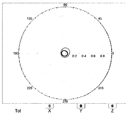
f=2500 MHz,R22,90°
