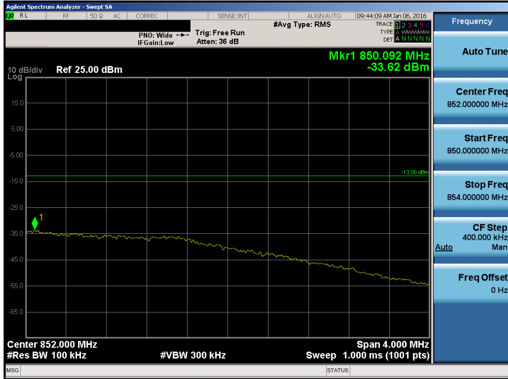
Plot 7-130. Upper Extended Band Edge Plot (Band 5 – Band 5 – 3.0MHz QPSK – RB Size 15)
