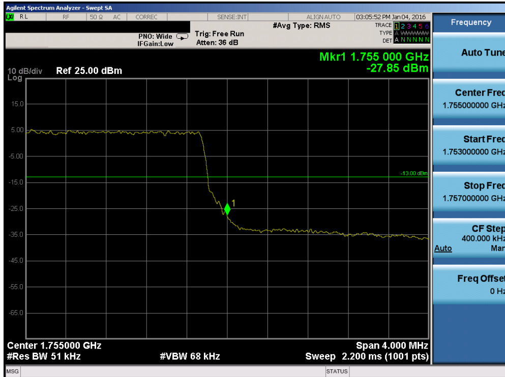
Plot 7-147. Upper Band Edge Plot (Band 4 – 5.0MHz QPSK – RB Size 25)
