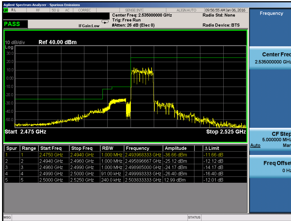
Plot 7-193. Lower ACP Plot (Band 7 – 5.0MHz QPSK – RB Size 25)
