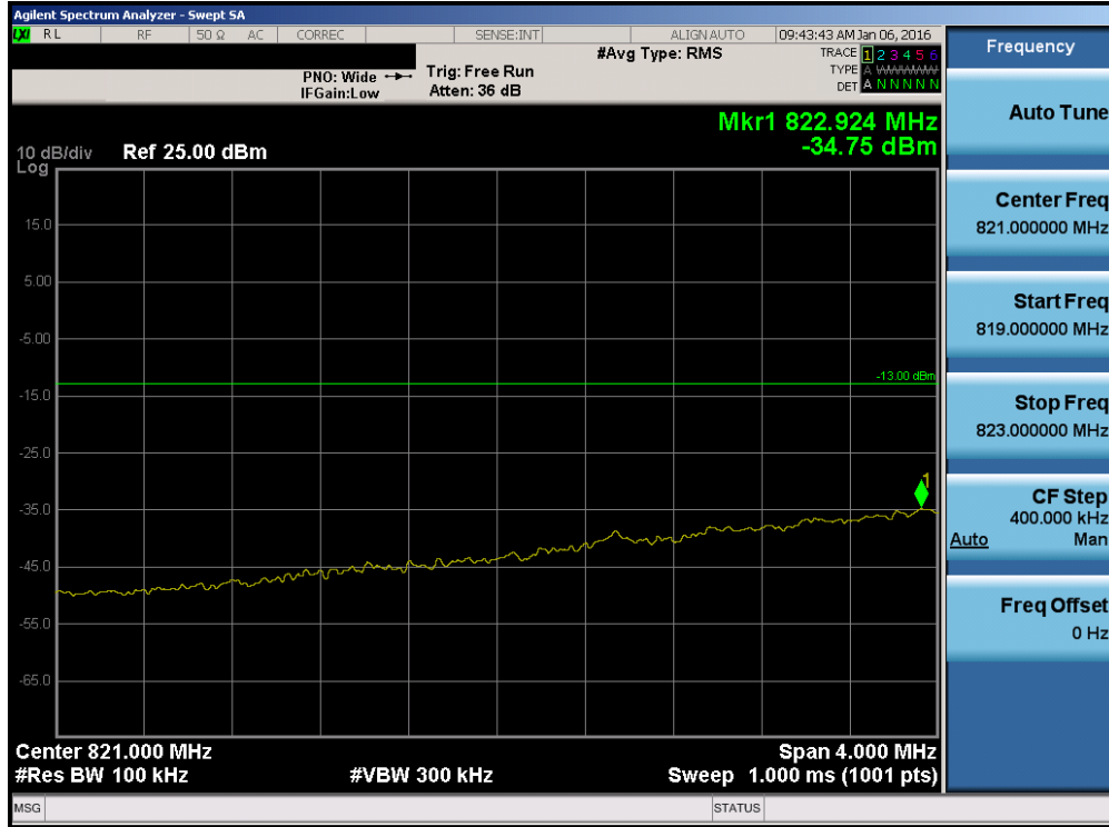
Plot 7-128. Lower Extended Band Edge Plot (Band 5 – 3.0MHz QPSK – RB Size 15)
