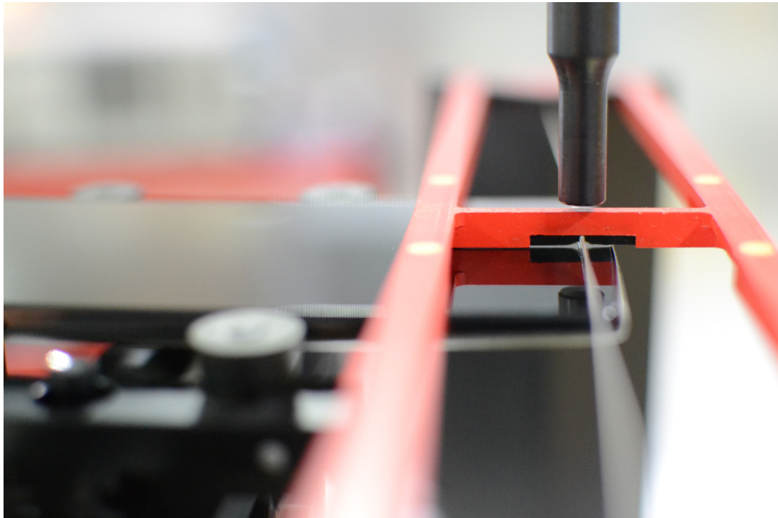
Figure 17-4 HAC Phantom Plane Alignment, Standard Cover
