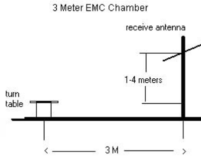
Figure 6-1. Test Instrument & Measurement Setup
