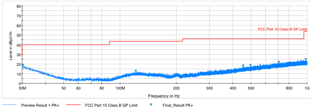
Plot 6-7. Radiated Spurious Plot below 1GHz (Pol. H)
