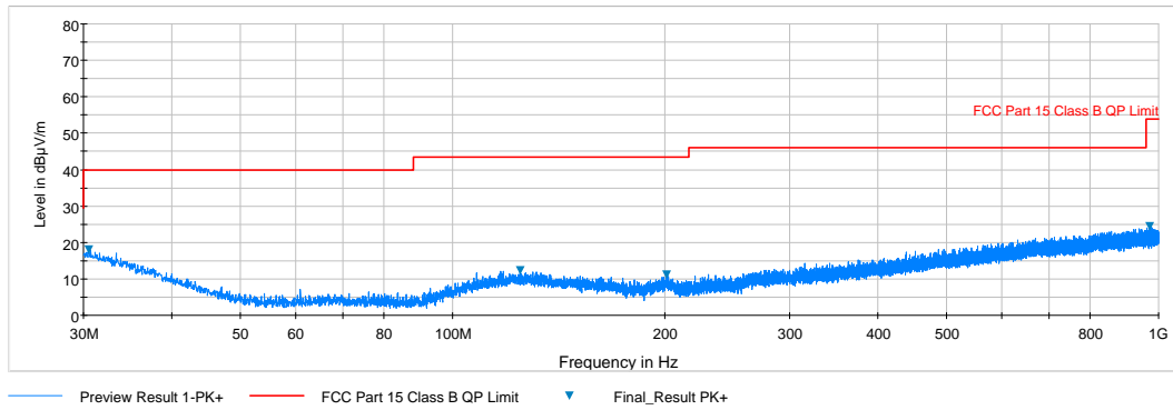
Plot 6-8. Radiated Spurious Plot below 1GHz (Pol. V)
