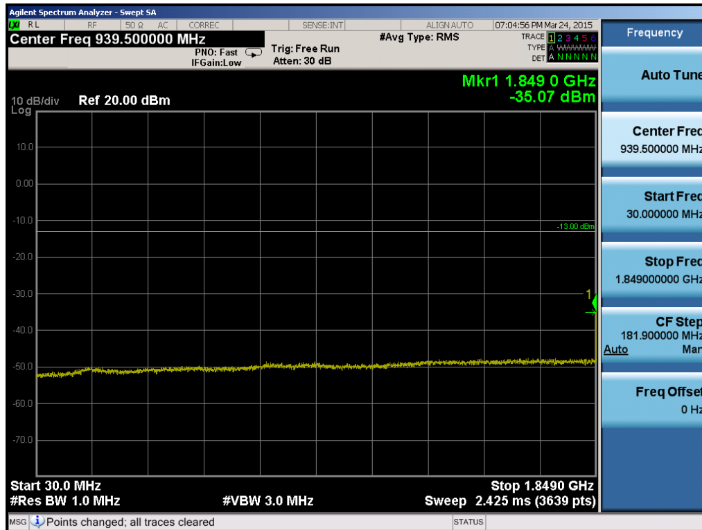
Plot 6-76. Conducted Spurious Plot (Band 2 – 1.4MHz QPSK – RB Size 1, RB Offset 0 – Low Channel)
