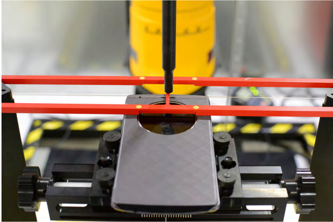
Figure 17-3 Ear Reference Point HAC Phantom Alignment (Wireless Charging Cover - Closed)
