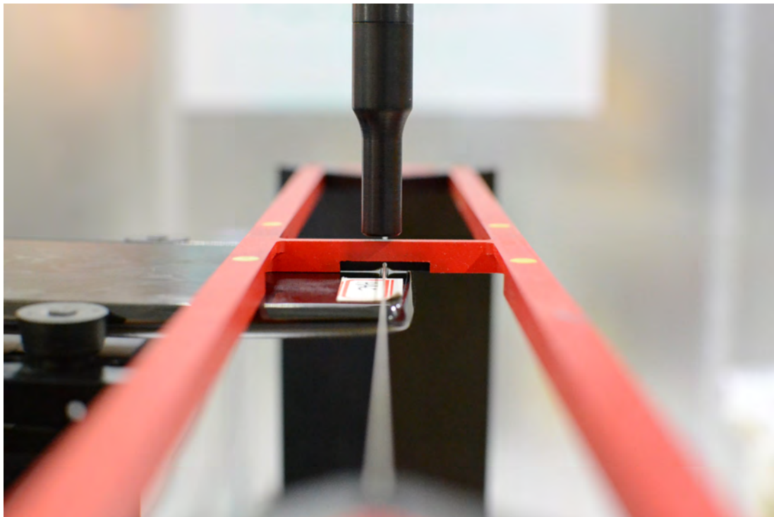
Figure 17-4 HAC Phantom Plane Alignment (Standard Battery Cover)
