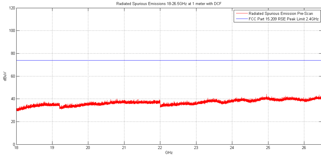
Plot 6-8. Radiated Spurious Plot above 18GHz (Pol. V)
