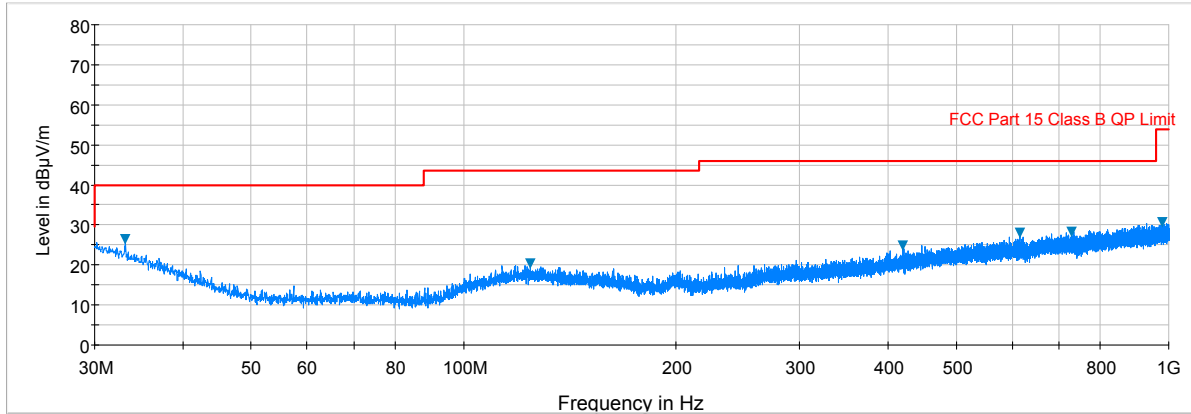
Plot 6-23. Radiated Spurious Plot below 1GHz (802.11a – U3 Ch. 157, Ant. Pol. H)
