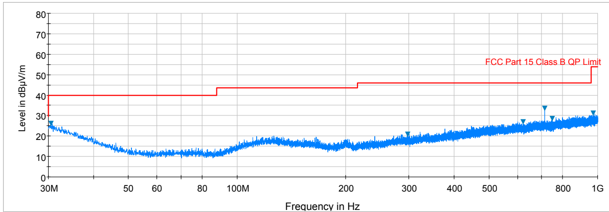
Plot 6-24. Radiated Spurious Plot below 1GHz (802.11a – U3 Ch. 157, Ant. Pol. V)
