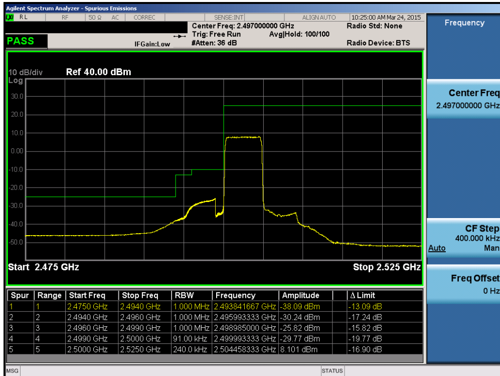
Plot 6-195. Lower ACP Plot (Band 7 – 5.0MHz QPSK – RB Size 25)
