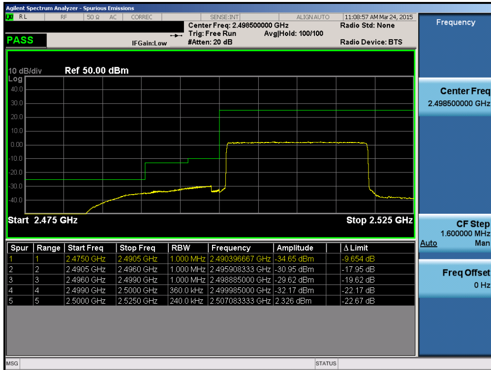
Plot 6-201. Lower ACP Plot (Band 7 – 20.0MHz QPSK – RB Size 100)
