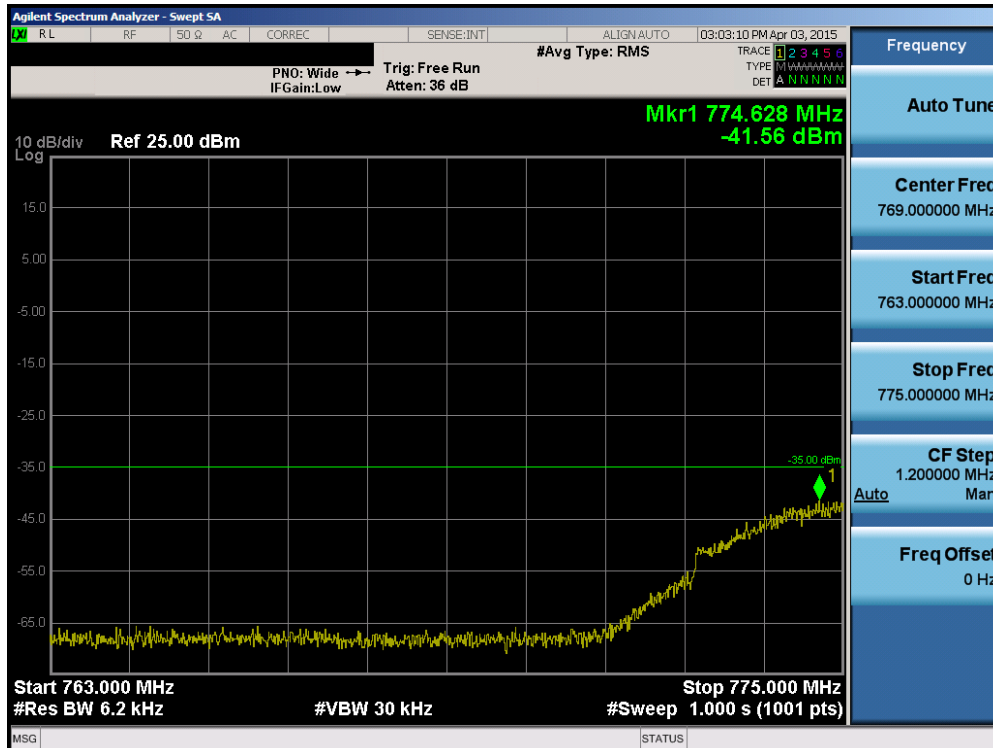
Plot 6-123. Lower Emission Mask Edge Plot (Band 13 – 5.0MHz QPSK – RB Size 25)
