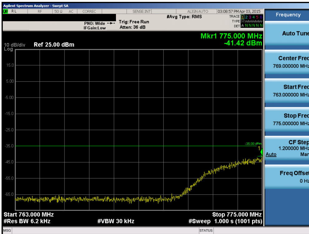
Plot 6-129. Lower Emission Mask Edge Plot (Band 13 – 10.0MHz QPSK – RB Size 50)
