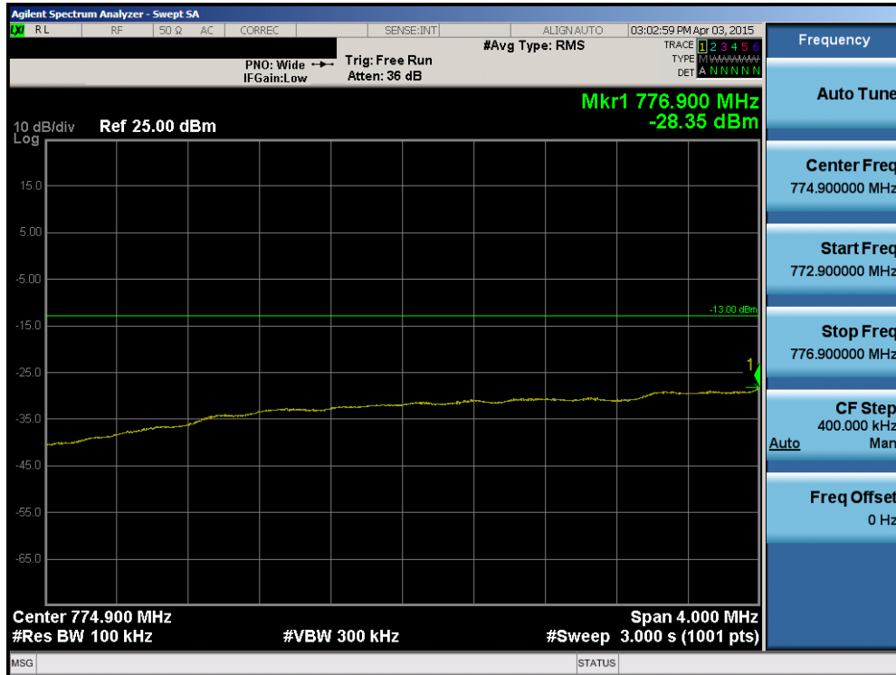
Plot 6-122. Lower Extended Band Edge Plot (Band 13 – 5.0MHz QPSK – RB Size 25)
