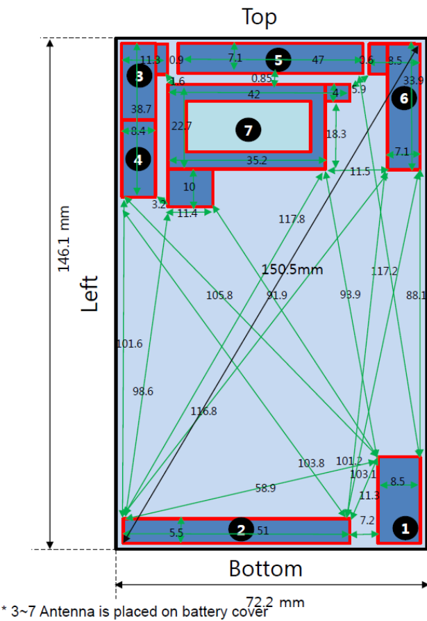
H791 Antenna Distance(Front View)
