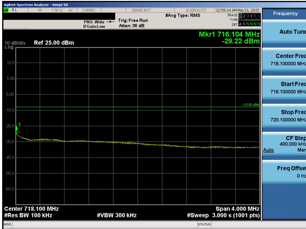
Plot 6-132. Upper Extended Band Edge Plot (Band 12 – 5.0MHz QPSK – RB Size 25)
