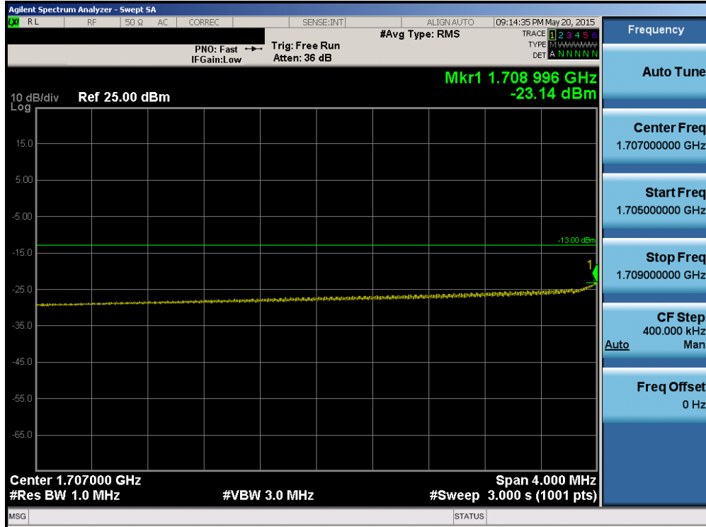
Plot 6-162. Lower Extended Band Edge Plot (Band 4 – 10.0MHz QPSK – RB Size 50)
