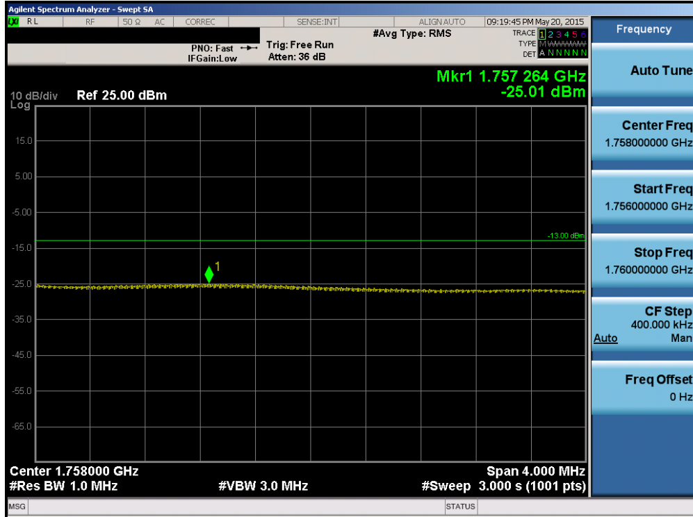
Plot 6-168. Upper Extended Band Edge Plot (Band 4 – 15.0MHz QPSK – RB Size 75)
