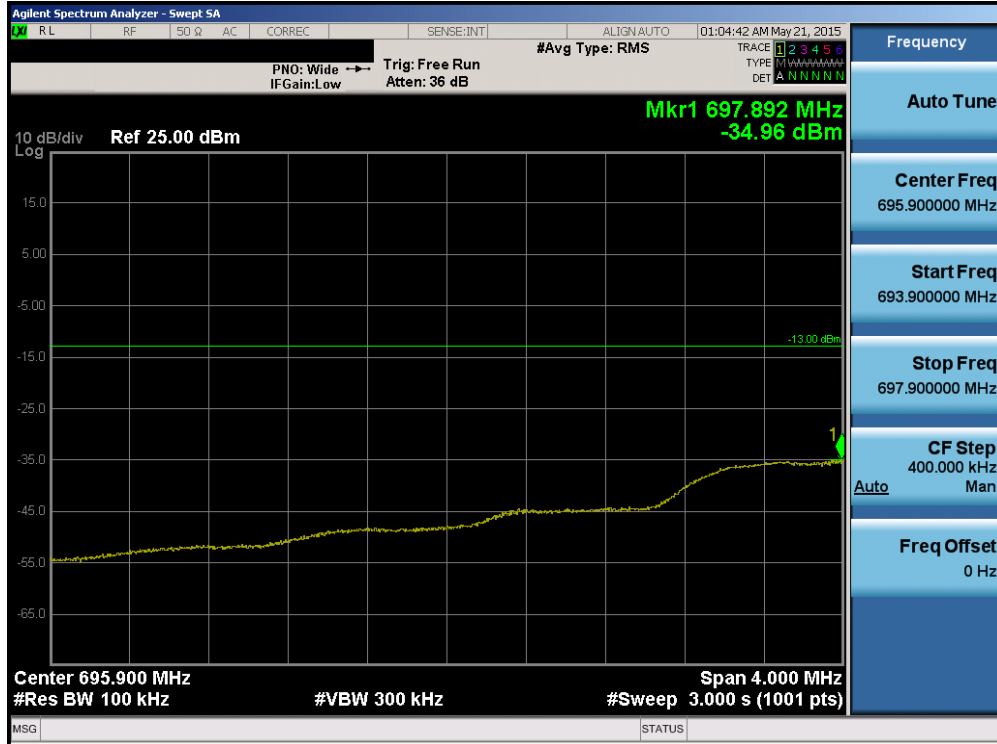
Plot 6-122. Lower Extended Band Edge Plot (Band 12 – 1.4MHz QPSK – RB Size 6)
