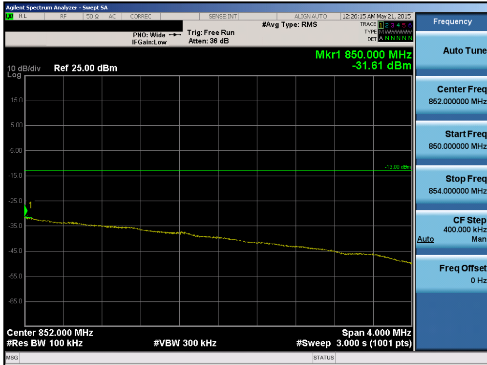
Plot 6-146. Upper Extended Band Edge Plot (Band 5 – 5.0MHz QPSK – RB Size 25)
