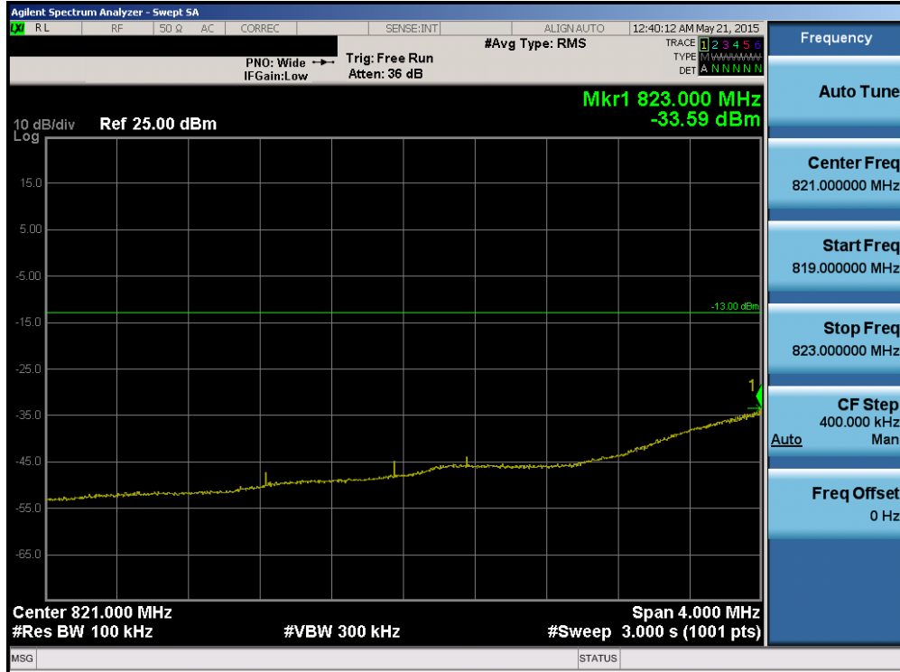
Plot 6-136. Lower Extended Band Edge Plot (Band 5 – 1.4MHz QPSK – RB Size 6)
