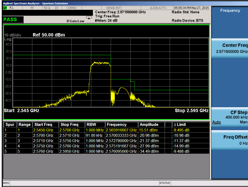
Plot 6-198. Upper ACP Plot (Band 7 – 5.0MHz QPSK – RB Size 25)
