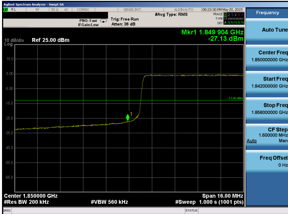
Plot 6-193. Lower Band Edge Plot (Band 2 – 20.0MHz QPSK – RB Size 100)
