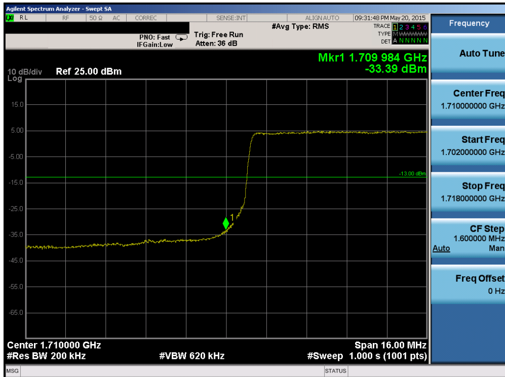
Plot 6-169. Lower Band Edge Plot (Band 4 – 20.0MHz QPSK – RB Size 100)
