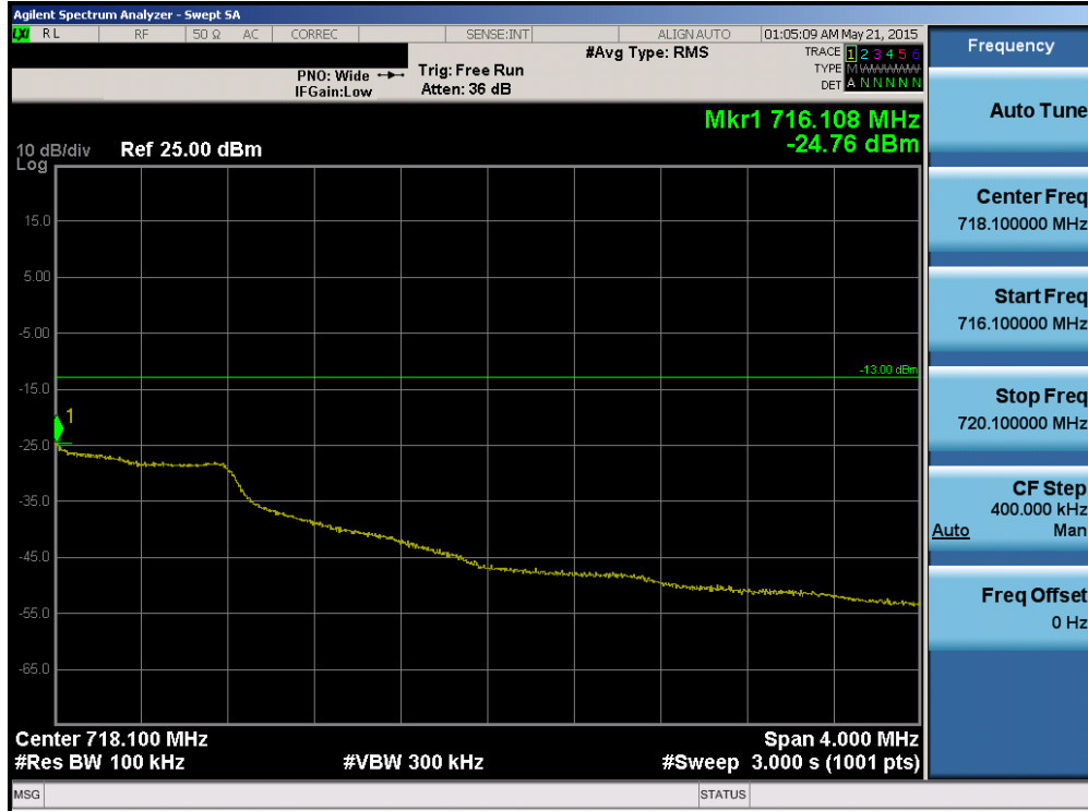
Plot 6-124. Upper Extended Band Edge Plot (Band 12 – 1.4MHz QPSK – RB Size 6)
