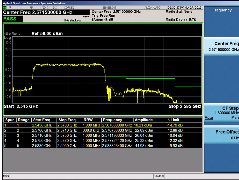
Plot 6-204. Upper ACP Plot (Band 7 – 20.0MHz QPSK – RB Size 100)
