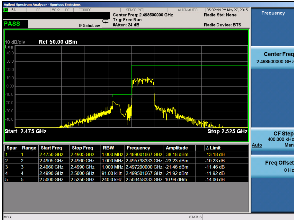
Plot 6-197. Lower ACP Plot (Band 7 – 5.0MHz QPSK – RB Size 25)
