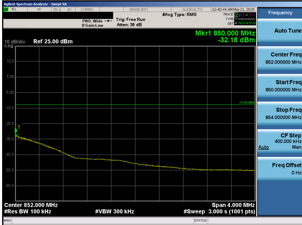
Plot 6-138. Upper Extended Band Edge Plot (Band 5 – 1.4MHz QPSK – RB Size 6)
