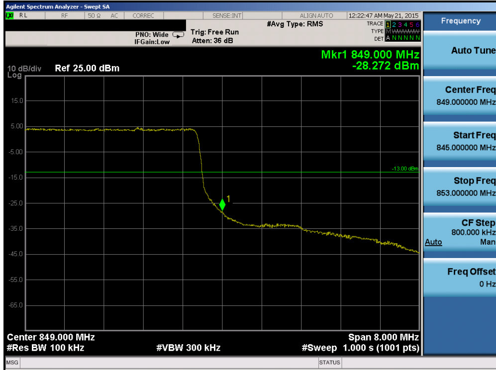
Plot 6-148. Upper Band Edge Plot (Band 5 – 10.0MHz QPSK – RB Size 50)
