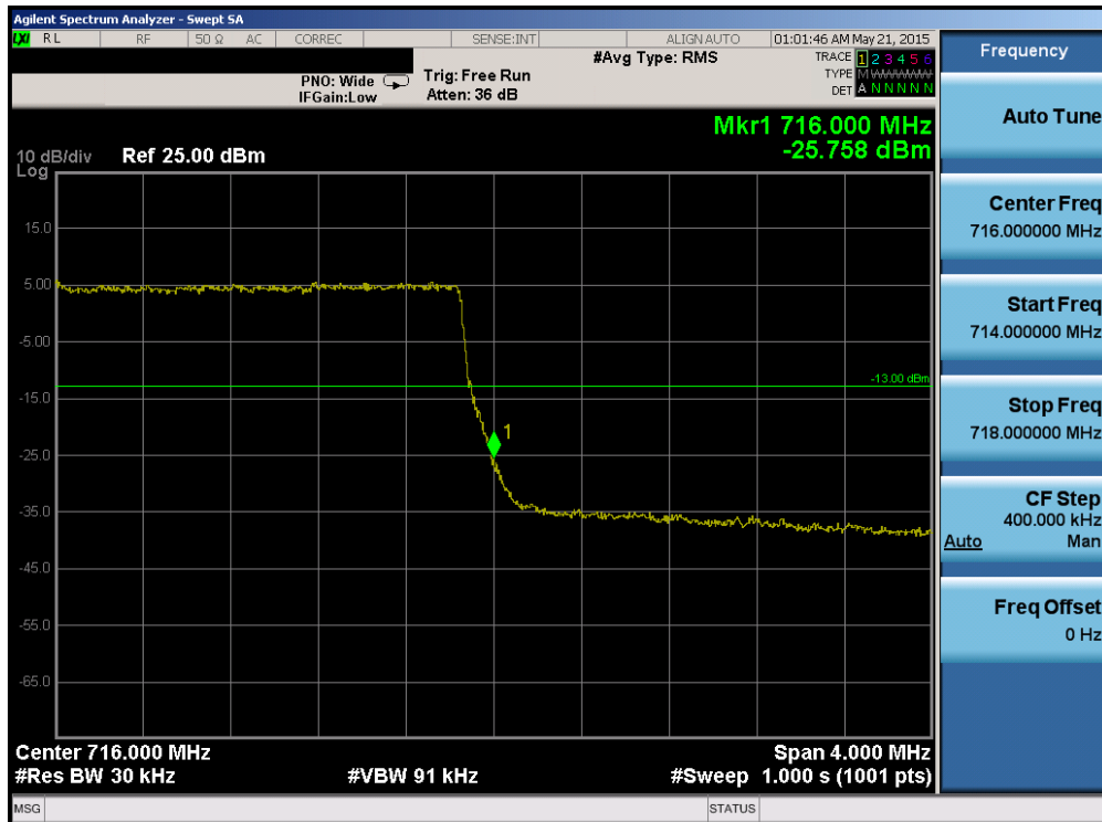
Plot 6-127. Upper Band Edge Plot (Band 12 – 3.0MHz QPSK – RB Size 15)
