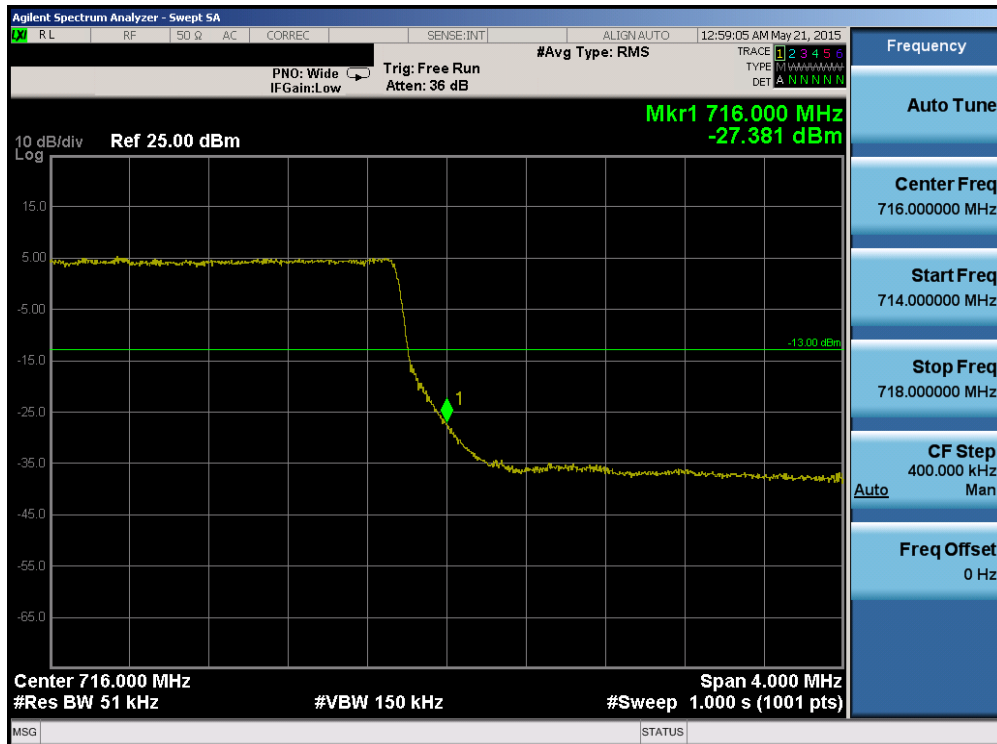
Plot 6-131. Upper Band Edge Plot (Band 12 – 5.0MHz QPSK – RB Size 25)
