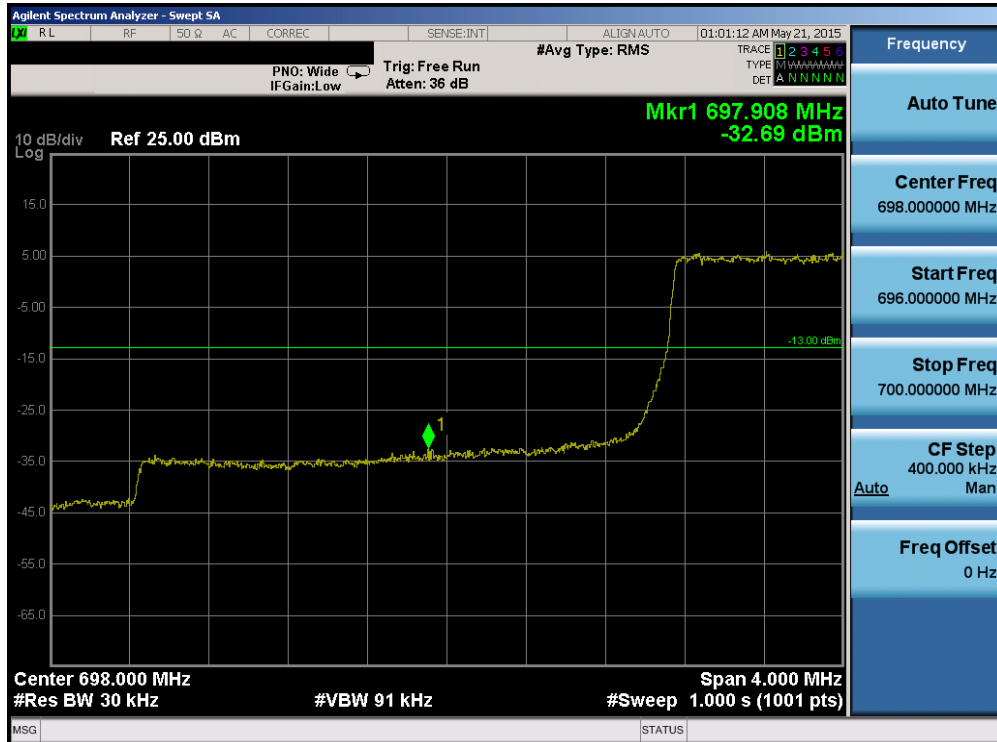
Plot 6-125. Lower Band Edge Plot (Band 12 – 3.0MHz QPSK – RB Size 15)
