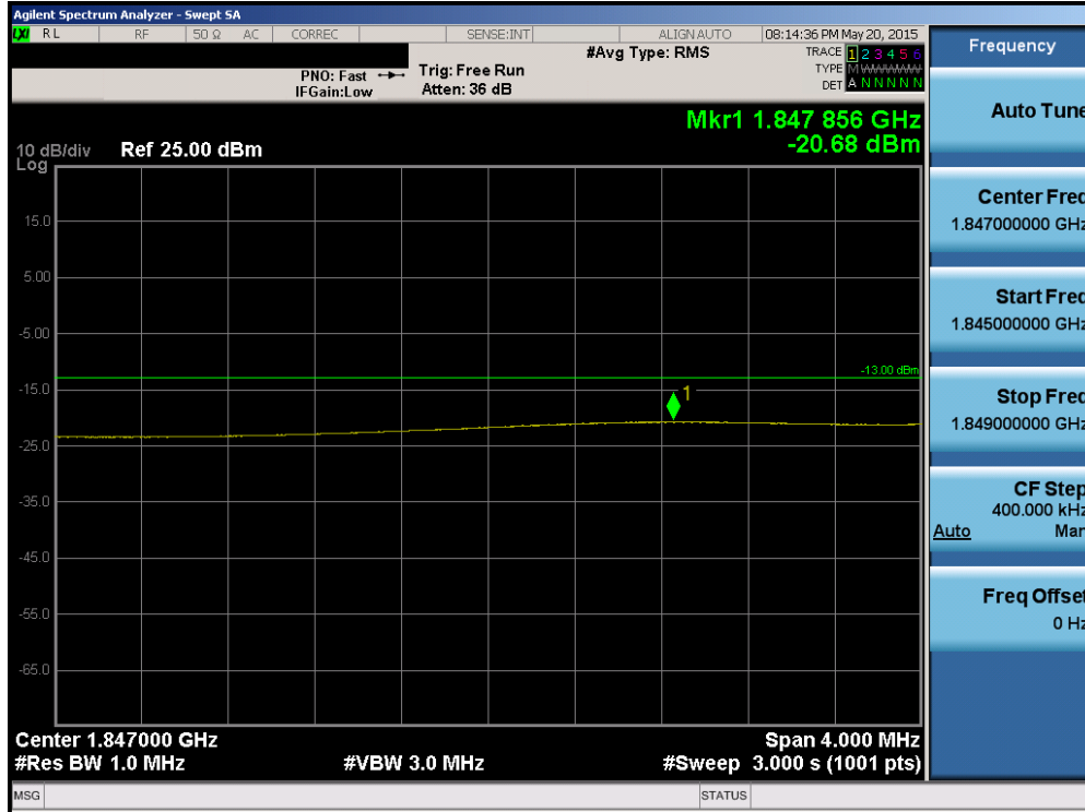
Plot 6-190. Lower Extended Band Edge Plot (Band 2 – 15.0MHz QPSK – RB Size 75)
