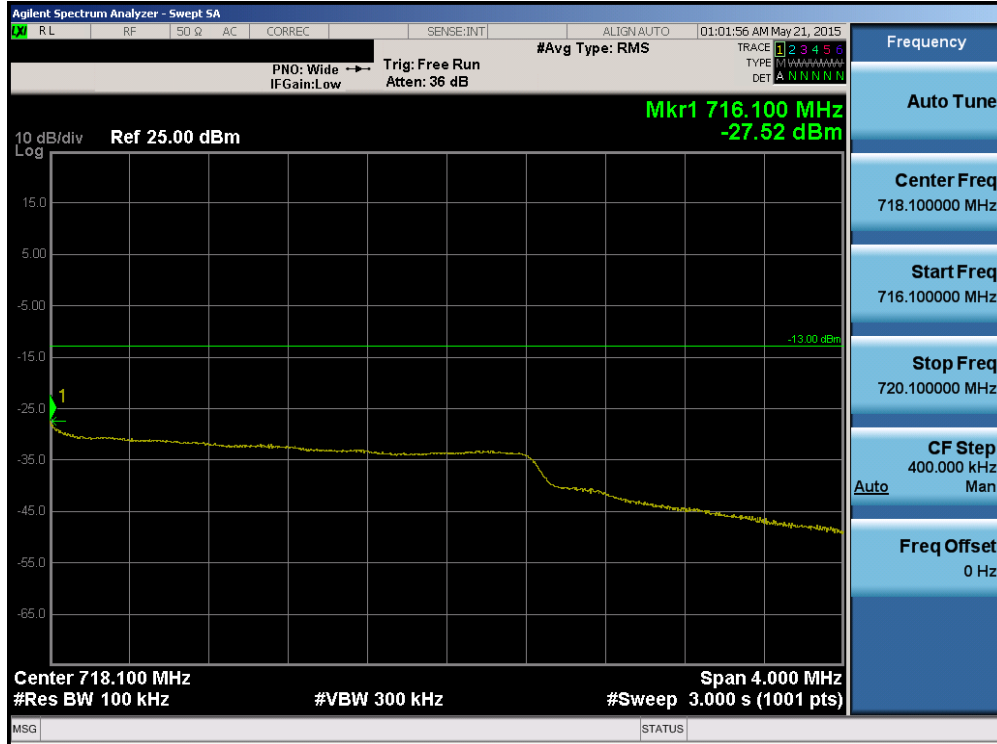
Plot 6-128. Upper Extended Band Edge Plot (Band 12 – 3.0MHz QPSK – RB Size 15)
