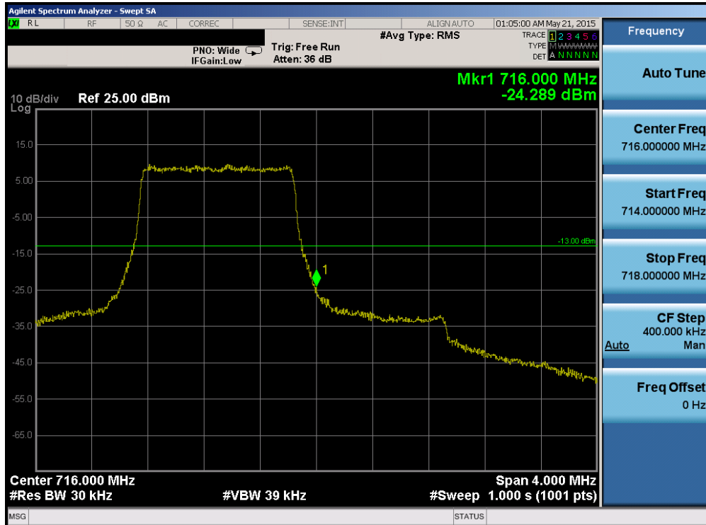
Plot 6-123. Upper Band Edge Plot (Band 12 – 1.4MHz QPSK – RB Size 6)
