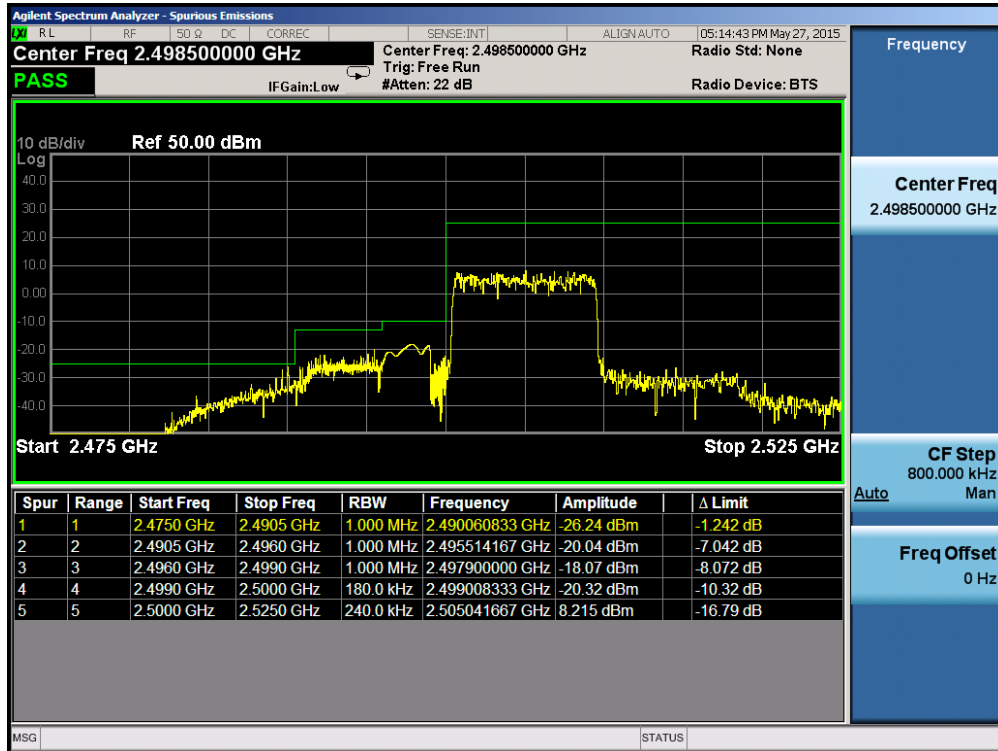
Plot 6-199. Lower ACP Plot (Band 7 – 10.0MHz QPSK – RB Size 50)
