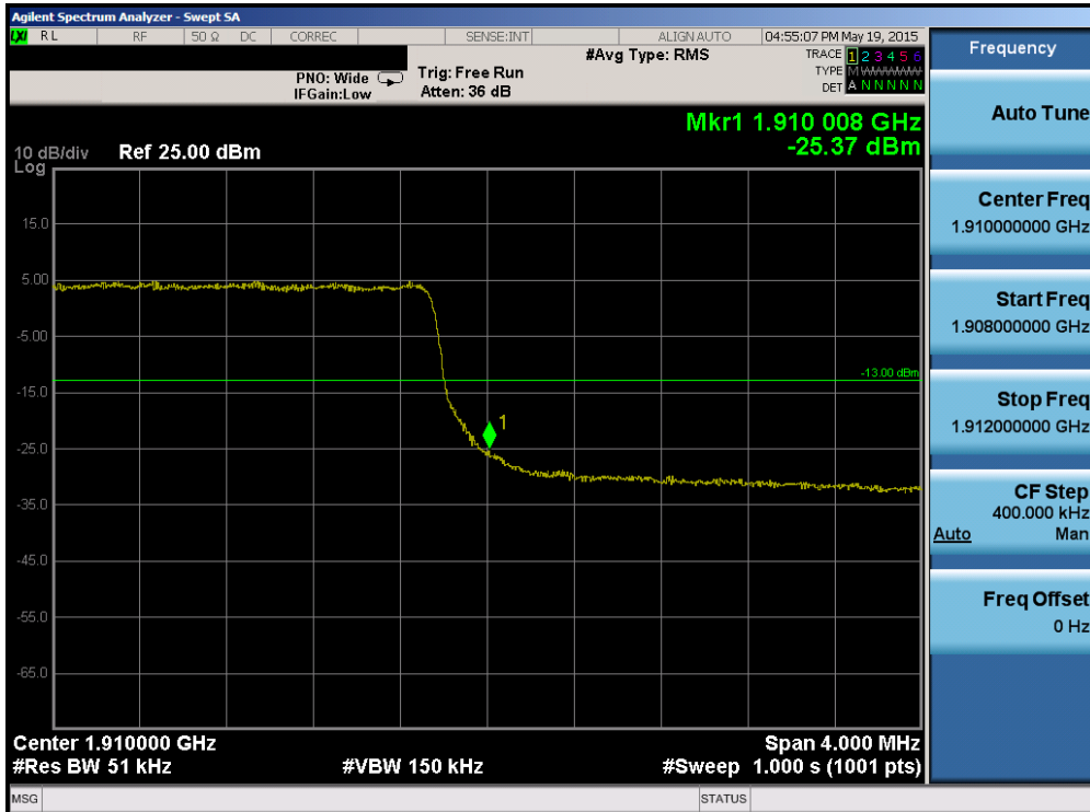
Plot 6-183. Upper Band Edge Plot (Band 2 – 5.0MHz QPSK – RB Size 25)
