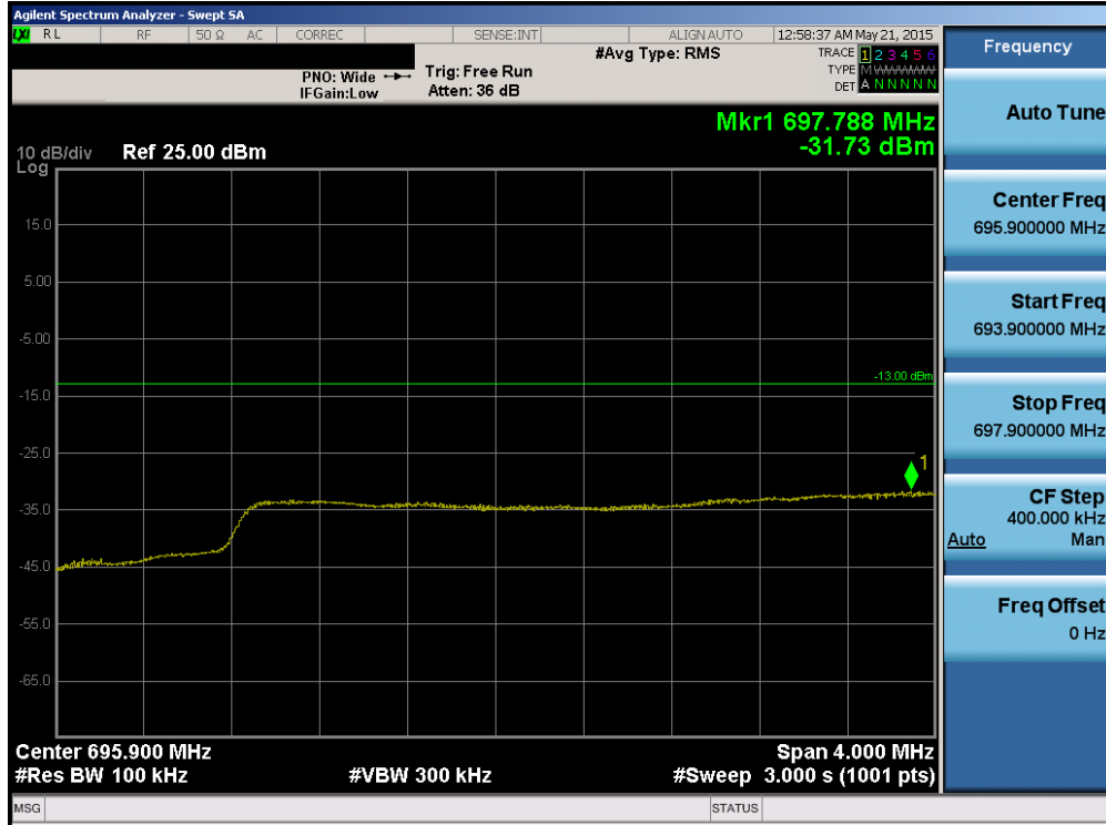
Plot 6-130. Lower Extended Band Edge Plot (Band 12 – 5.0MHz QPSK – RB Size 25)
