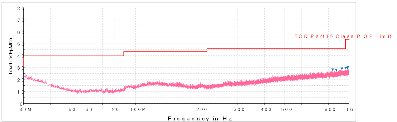
Plot 6-29. Radiated Spurious Plot below 1GHz (Pol. V)
