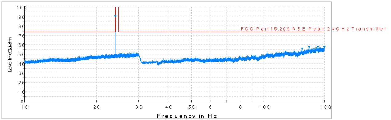
Plot 6-19. Radiated Spurious Plot above 1GHz (BTLE – Ch. 0, Ant. Pol. V)
