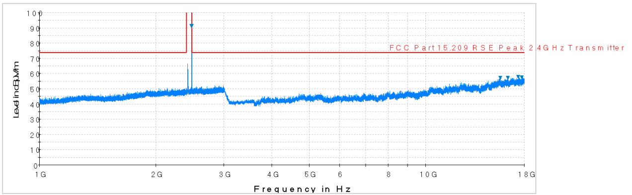
Plot 6-22. Radiated Spurious Plot above 1GHz (BTLE – Ch. 39, Ant. Pol. H)
