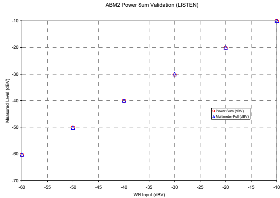
Figure 4-10 ABM2 Power Sum Validation
