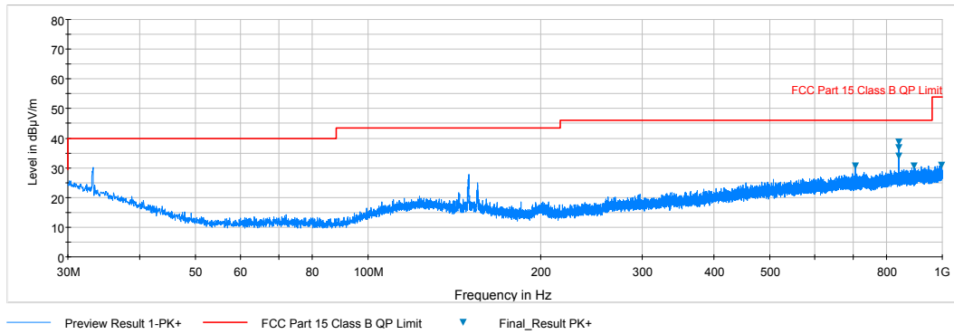
Plot 6-23. Radiated Spurious Plot below 1GHz (Pol. V)
