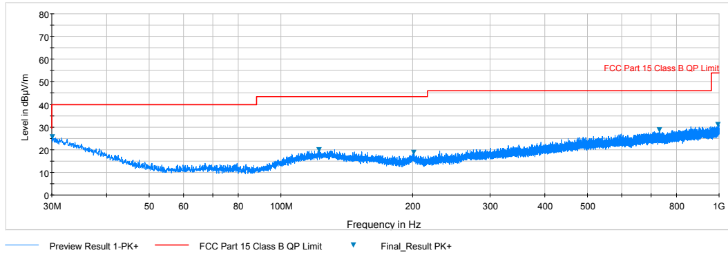
Plot 6-22. Radiated Spurious Plot below 1GHz (Pol. H)
