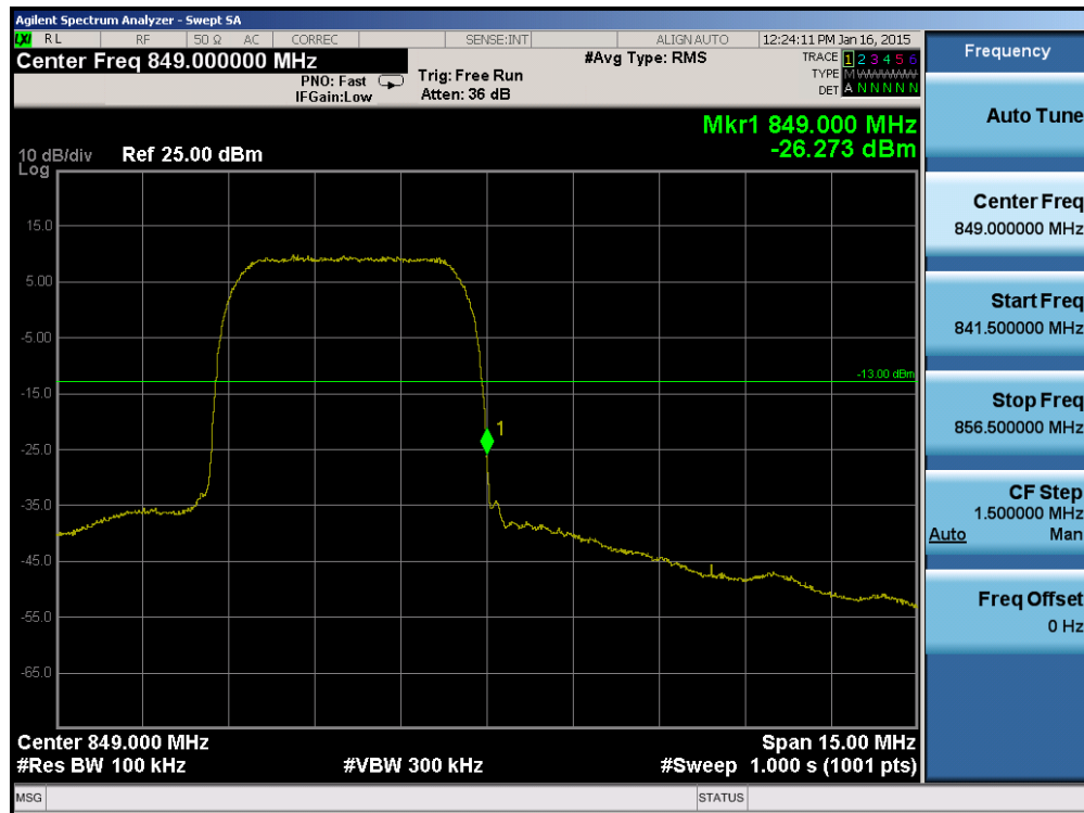
Plot 6-58. Band Edge Plot (Cellular WCDMA Mode – Ch. 4233)
