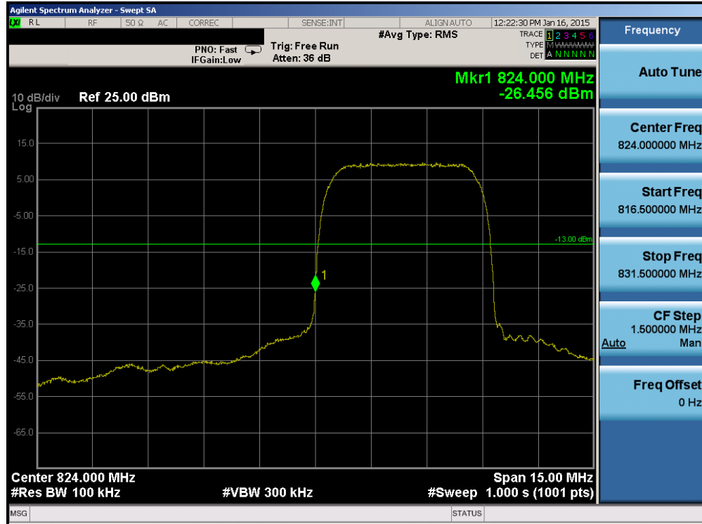
Plot 6-57. Band Edge Plot (Cellular WCDMA Mode – Ch. 4132)
