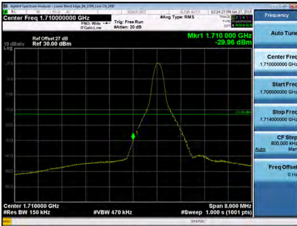
BAND 4. L Lower Band Edge Plot (15M BW Ch.20025 QPSK RB 1, Offset 0) -1
