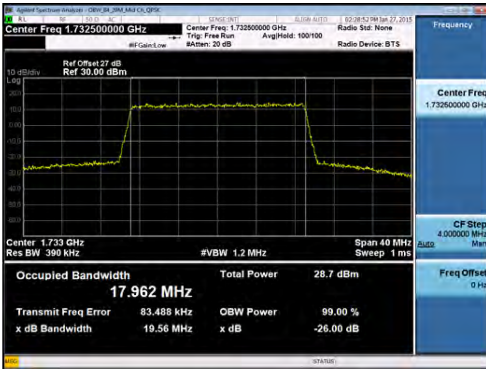
BAND 4. Occupied Bandwidth Plot (20M BW Ch.20175 QPSK RB 100)
