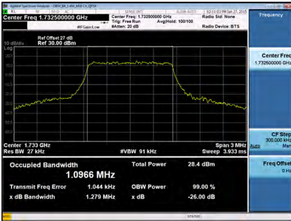
BAND 4. Occupied Bandwidth Plot (1.4M BW Ch.20175 QPSK RB 6)
