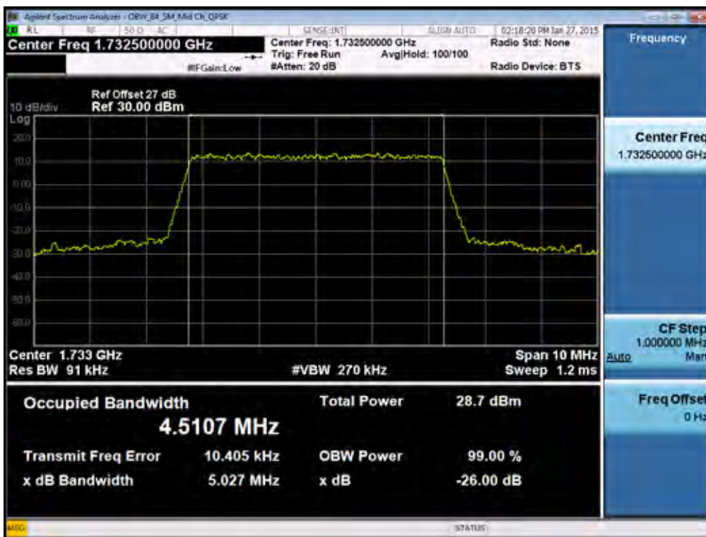
BAND 4. Occupied Bandwidth Plot (5M BW Ch.20175 QPSK RB 25)
