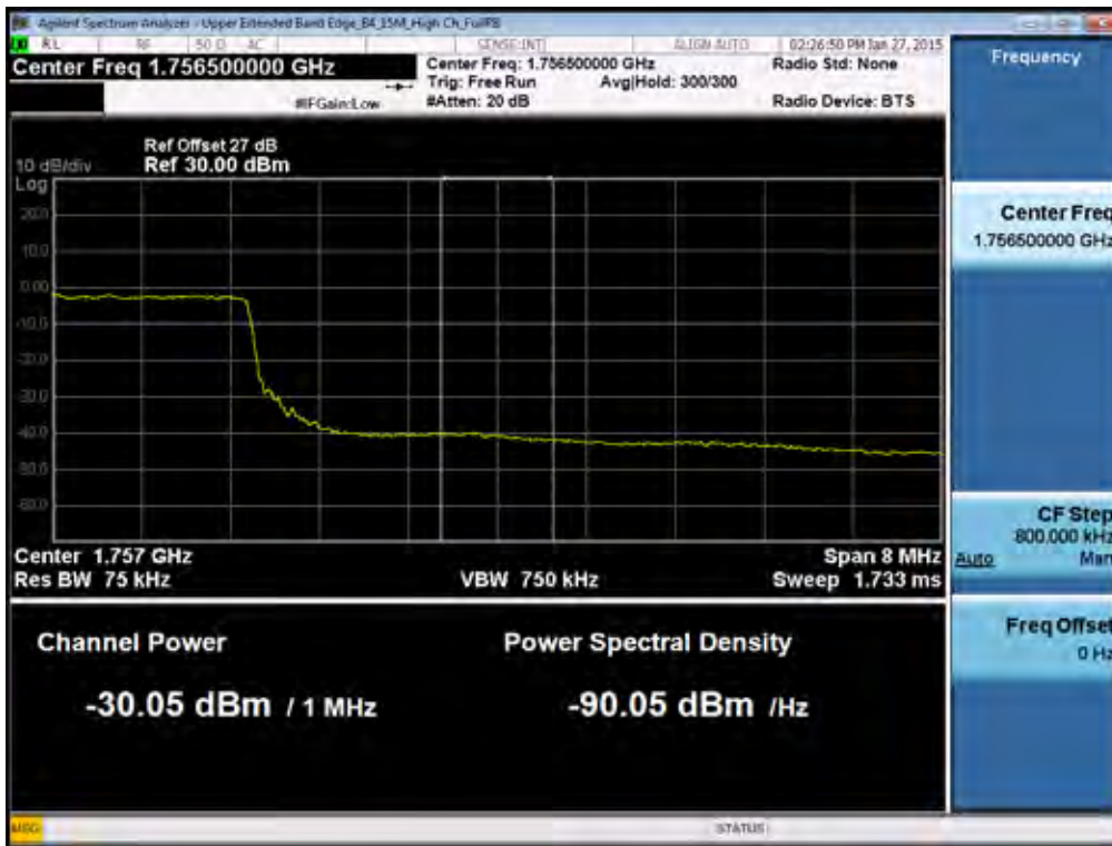
BAND 4. Upper Extended Band Edge Plot (15M BW Ch.20325 QPSK_RB75) -3
