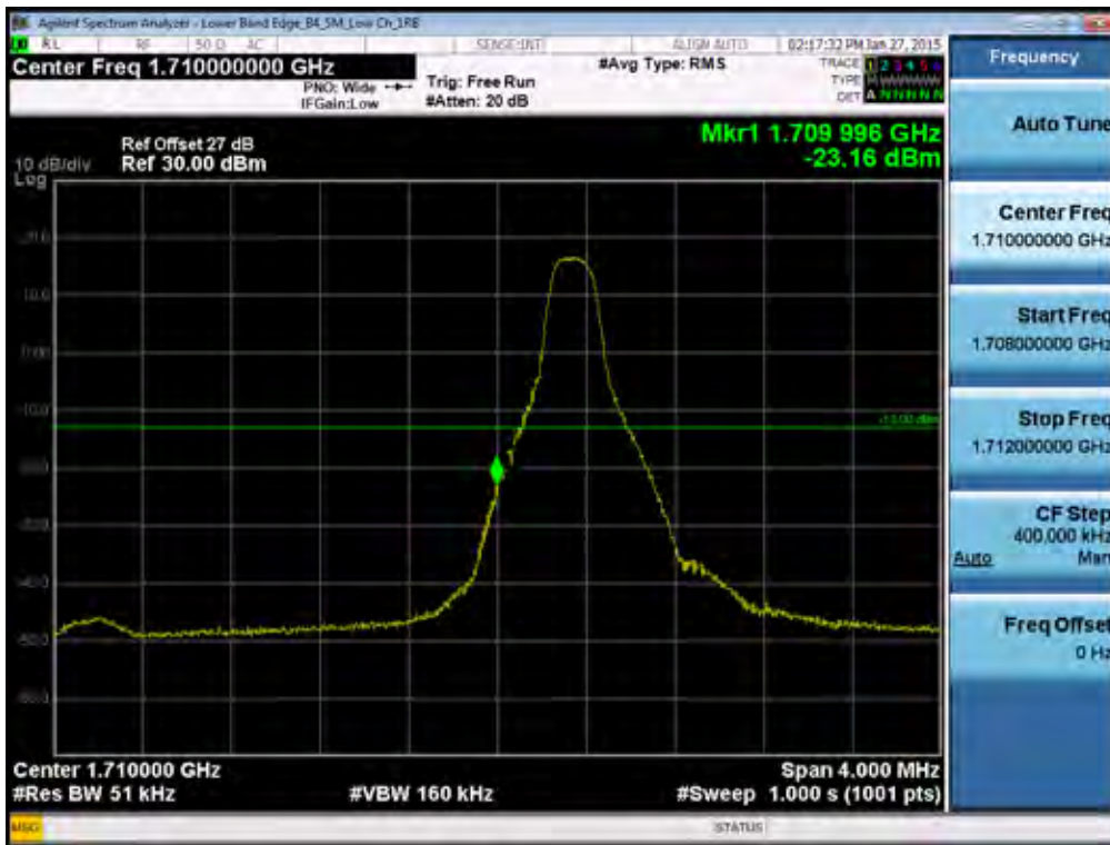
BAND 4. Lower Band Edge Plot (5M BW Ch.19975 QPSK RB 1, Offset 0) -1
