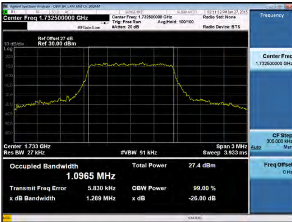
BAND 4. Occupied Bandwidth Plot (1.4M BW Ch.20175 16QAM RB 6)
