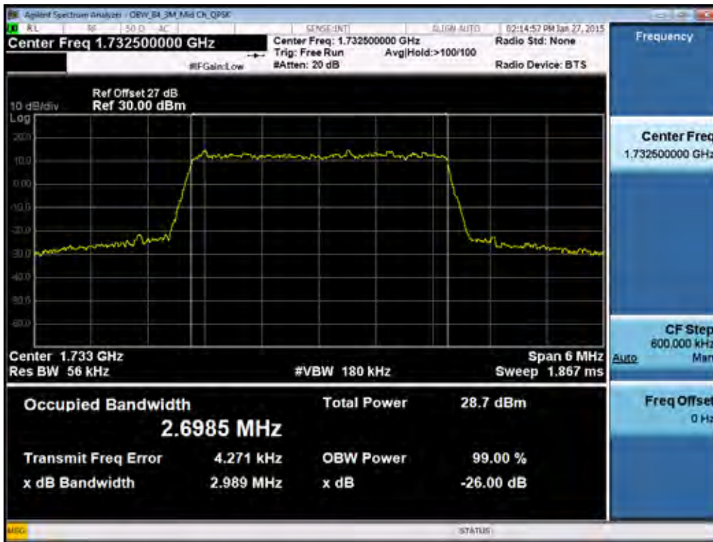
BAND 4. Occupied Bandwidth Plot (3M BW Ch.20175 QPSK RB 15)
