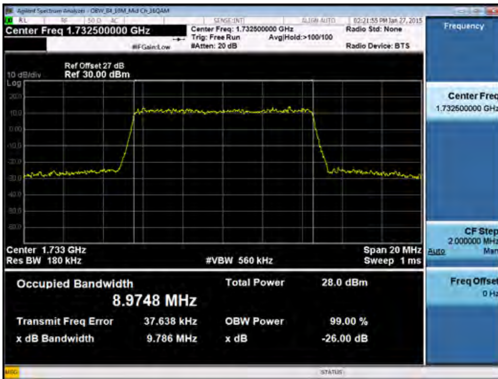
BAND 4. Occupied Bandwidth Plot (10M BW Ch.20175 16QAM RB 50)
