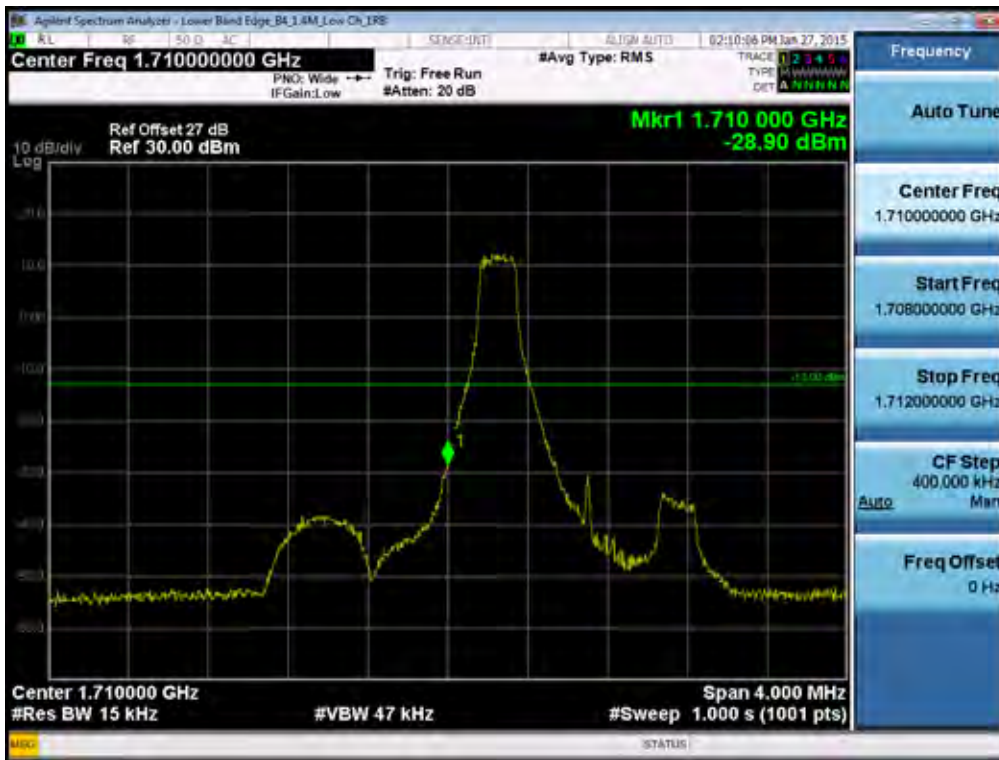
BAND 4. Lower Band Edge Plot (1.4M BW Ch.19957 QPSK RB 1, Offset 0) -1
