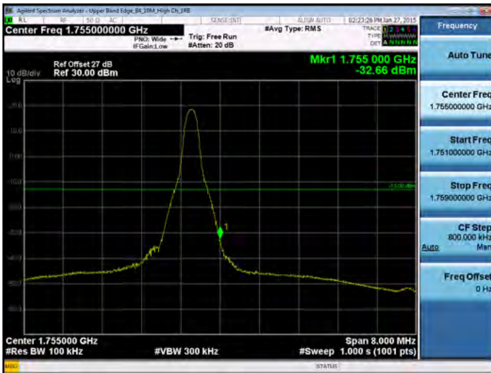
BAND 4. Upper Band Edge Plot (10M BW Ch.20350 QPSK_RB1_Offset 49) -1
