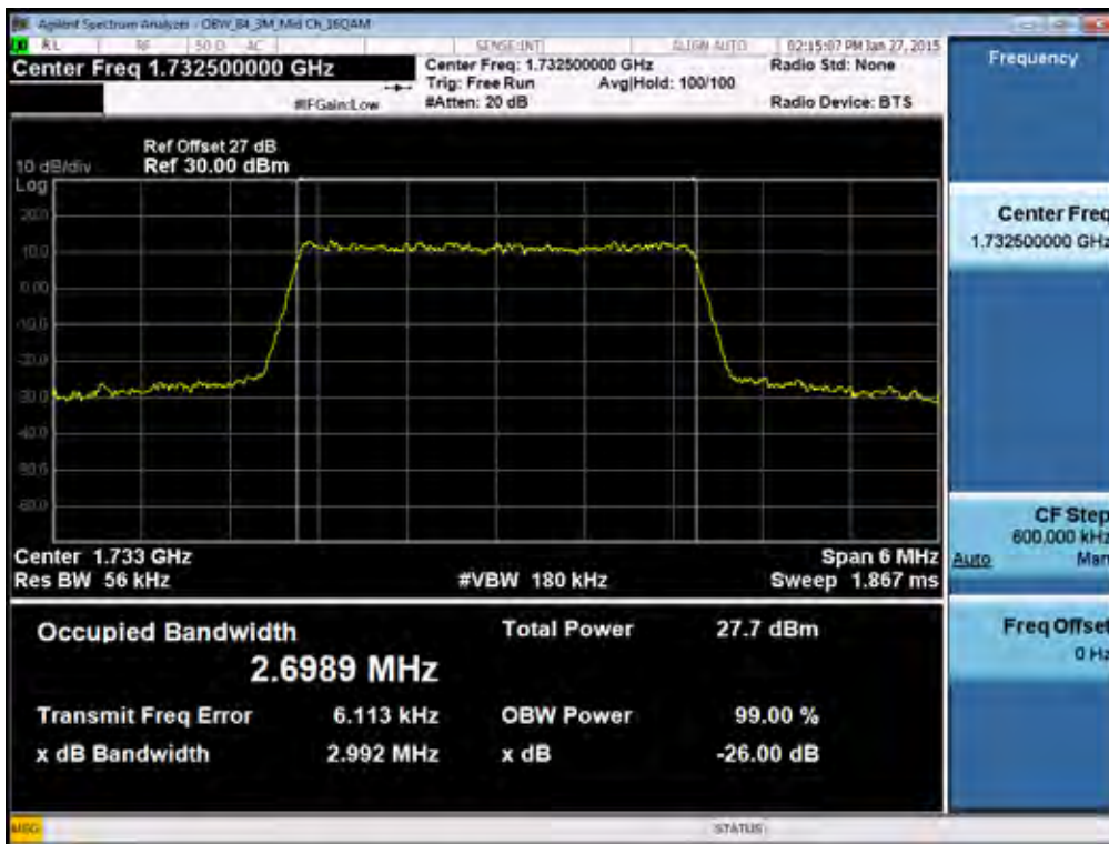
BAND 4. Occupied Bandwidth Plot (3M BW Ch.20175 16QAM RB 15)
