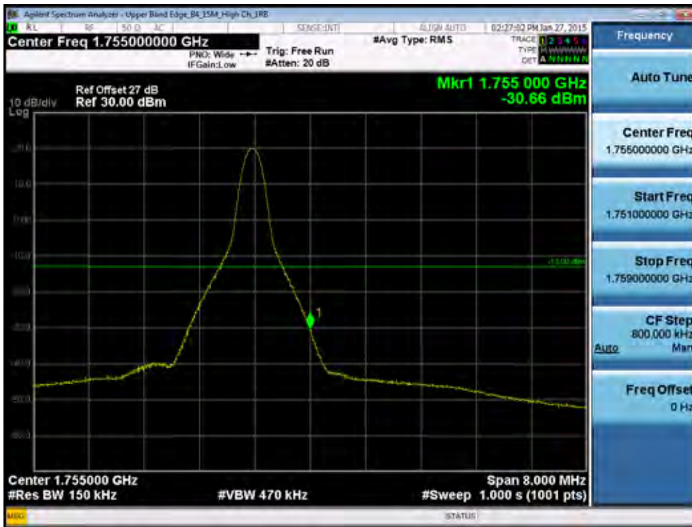
BAND 4. Upper Band Edge Plot (15M BW Ch.20325 QPSK_RB1_Offset 74) -1
