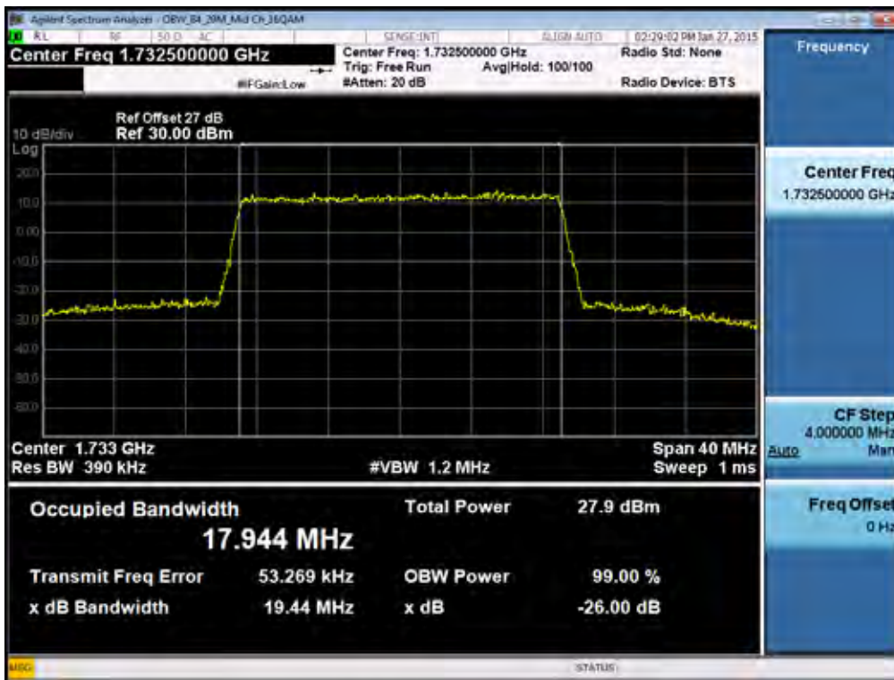
BAND 4. Occupied Bandwidth Plot (20M BW Ch.20175 16QAM RB 100)
