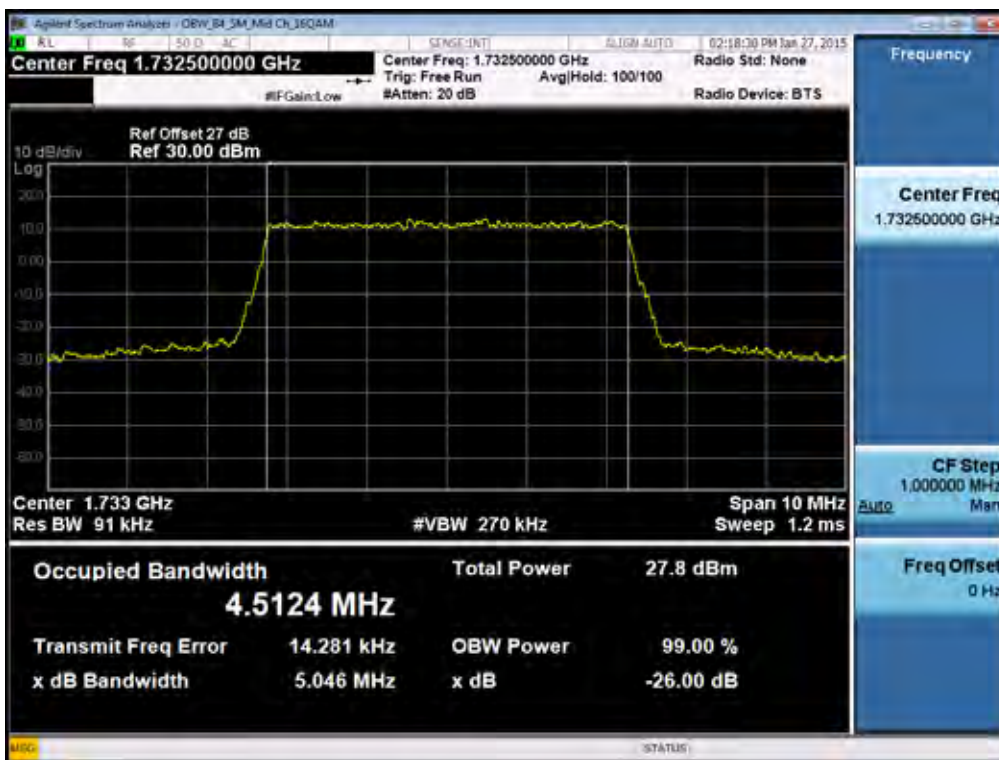
BAND 4. Occupied Bandwidth Plot (5M BW Ch.20175 16QAM RB 25)
