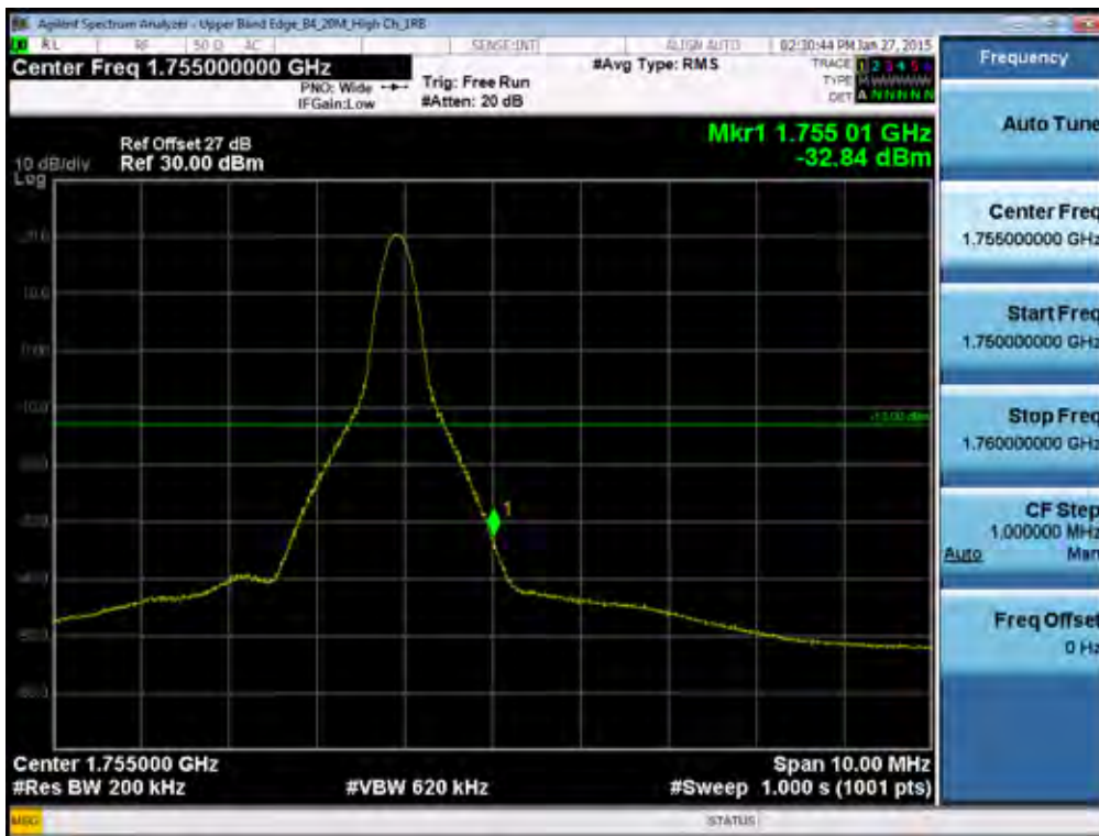
BAND 4. Upper Band Edge Plot (20M BW Ch.20300 QPSK_RB1_Offset 99) -1
