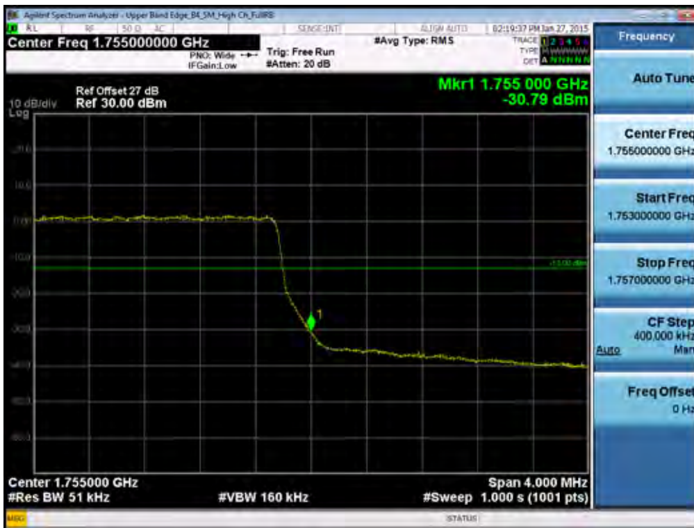
BAND 4. Upper Band Edge Plot (5M BW Ch.20375 QPSK_RB25) -2
