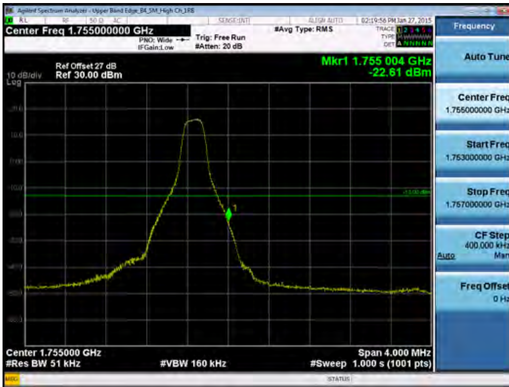
BAND 4. Upper Band Edge Plot (5M BW Ch.20375 QPSK_RB1_Offset 24) -1
