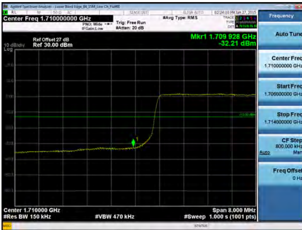
BAND 4. Lower Band Edge Plot (15M BW Ch.20025 QPSK RB 75) -2
