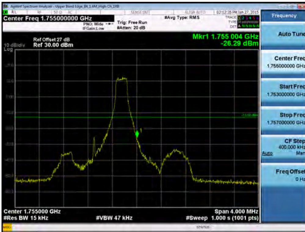
BAND 4. Upper Band Edge Plot (1.4M BW Ch.20393 QPSK_RB1_Offset) -1
