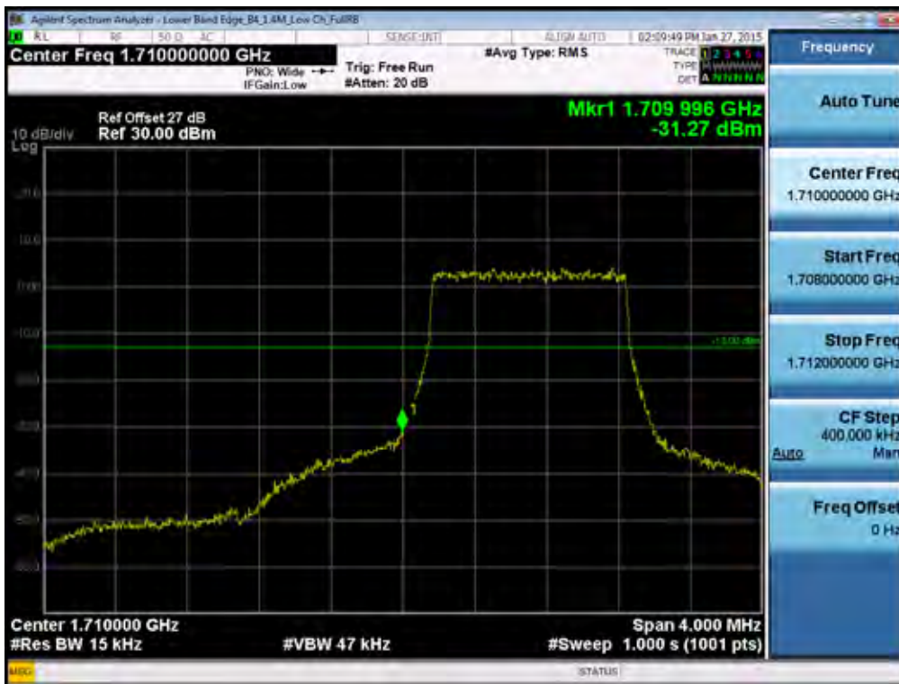
BAND 4. Lower Band Edge Plot (1.4M BW Ch.19957 QPSK RB 6) -2
