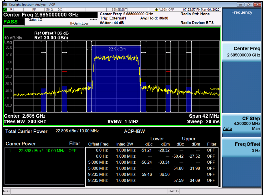
LTE Band 41 / 10MHz / 16QAM - RB Size/Offset (50/0)
