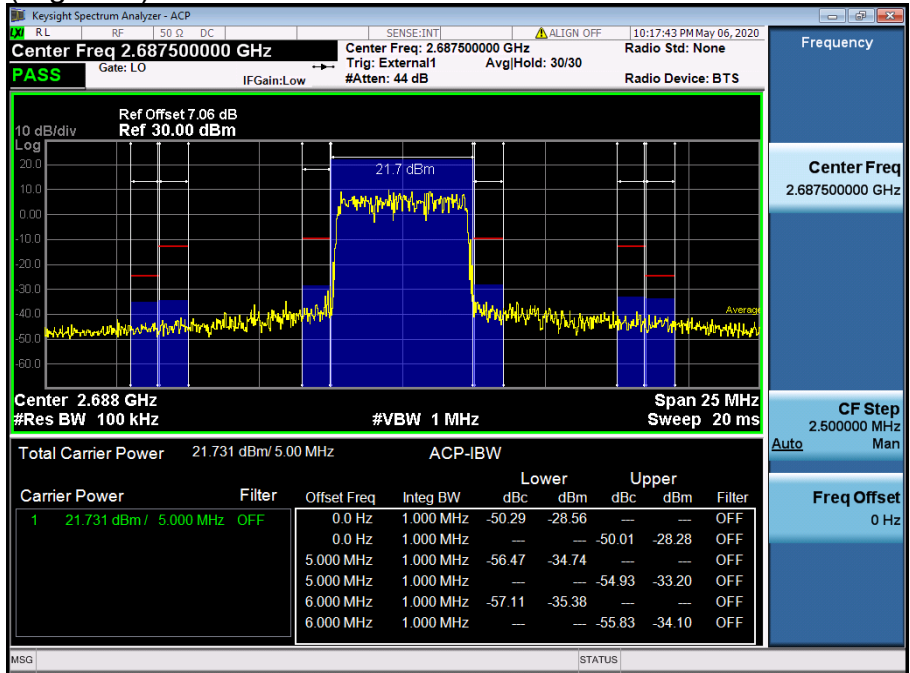
LTE Band 41 / 5MHz / 64QAM - RB Size/Offset (25/0)
