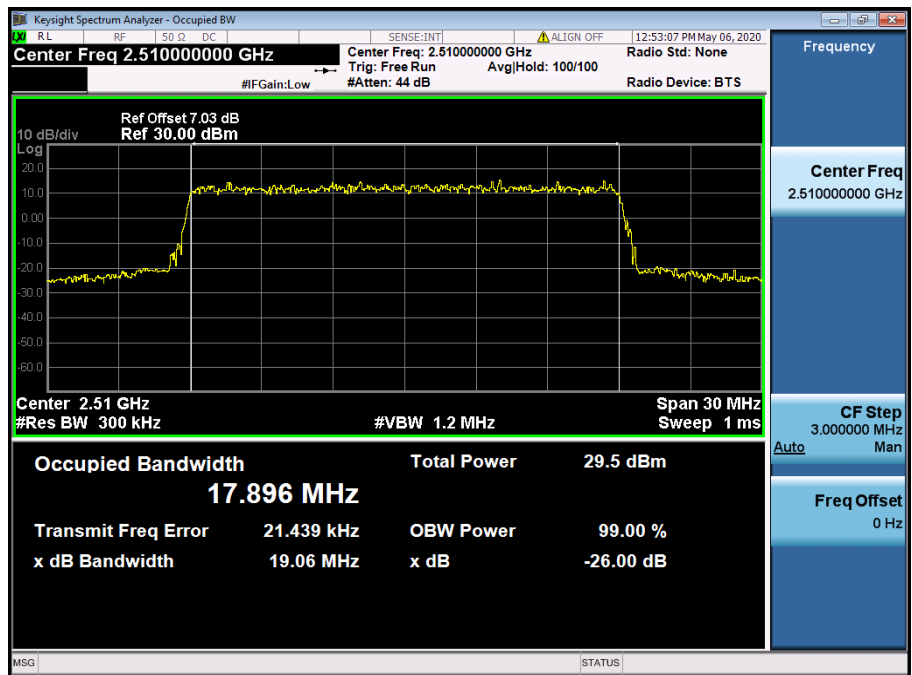
LTE Band 7 / 20 MHz / 64QAM - RB Size 100
