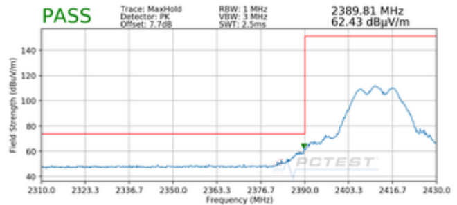
Plot 7-10. Radiated Restricted Lower Band Edge Measurement MIMO (Peak)
