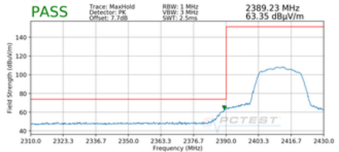
Plot 7-2. Radiated Restricted Lower Band Edge Measurement SISO ANT1 (Peak)
