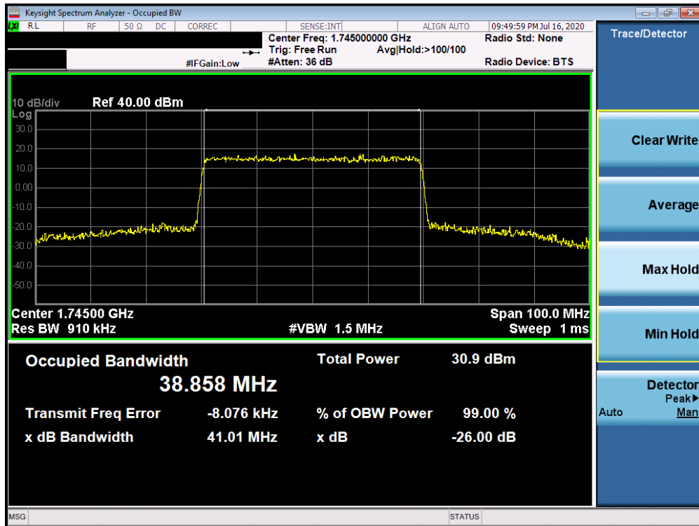
Plot 7-131. Occupied Bandwidth Plot (n66 40MHz 16QAM-CP-OFDM - Full RB Configuration)
