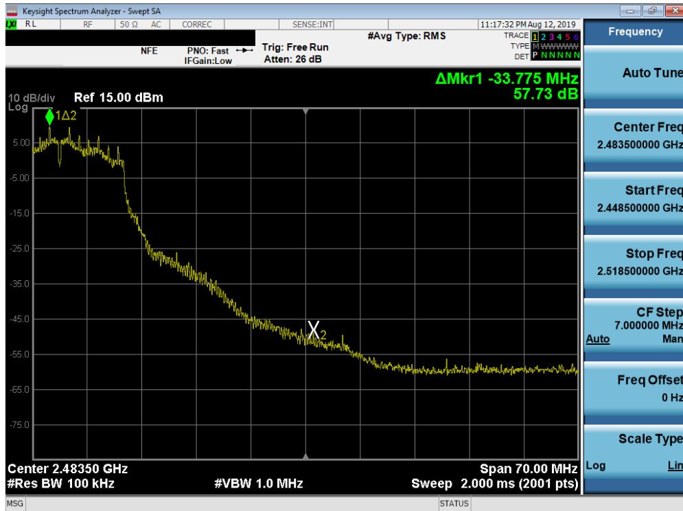
Plot 7-48. Band Edge Plot SISO ANT1 (802.11g- Ch. 9)
