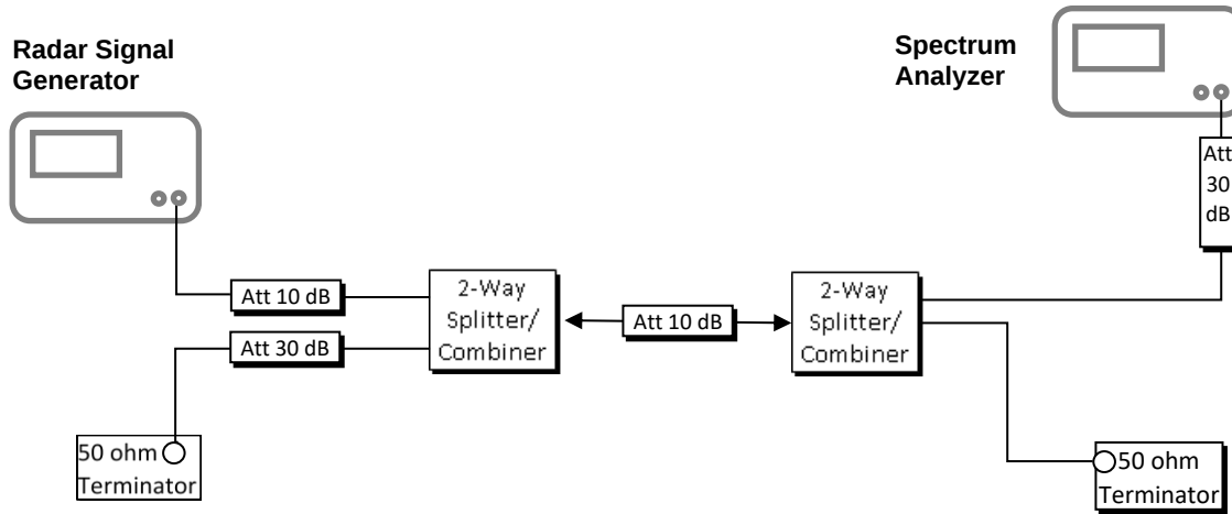
Figure 4-2. Radar Waveform Calibration
