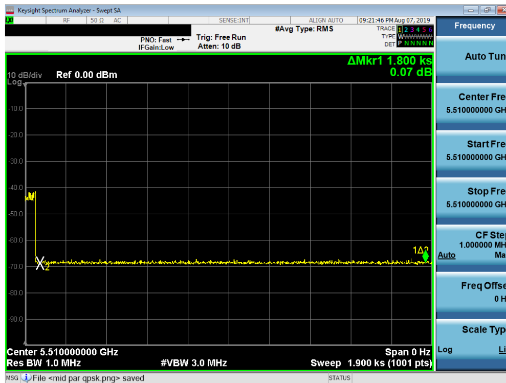
Figure 6-3. Band 2C Client Beacon Test – Monitoring live spectrum – Elapse time 30 minutes
