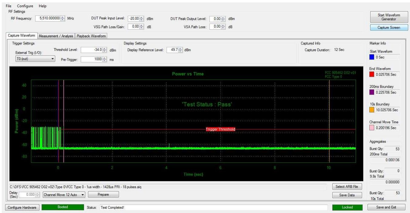
Figure 6-2. Band 2C Move Time and Aggregate Time
