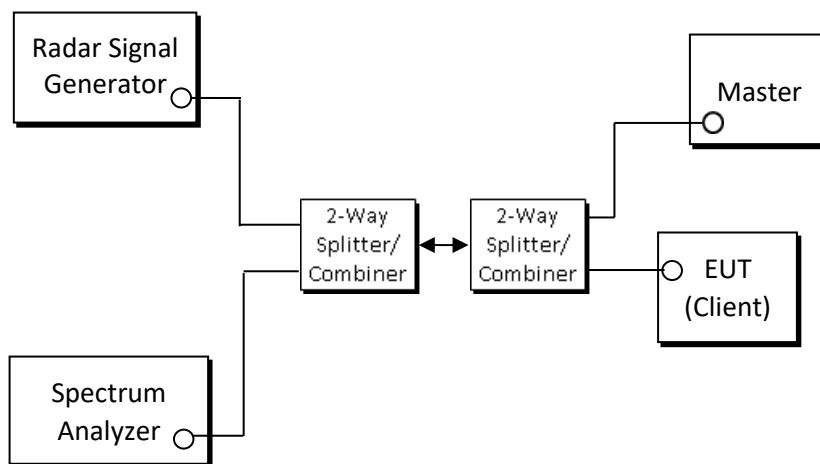
Figure 5-1. Test Setup
