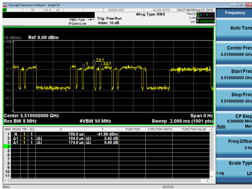
Figure 6-1. Band 2C Period
