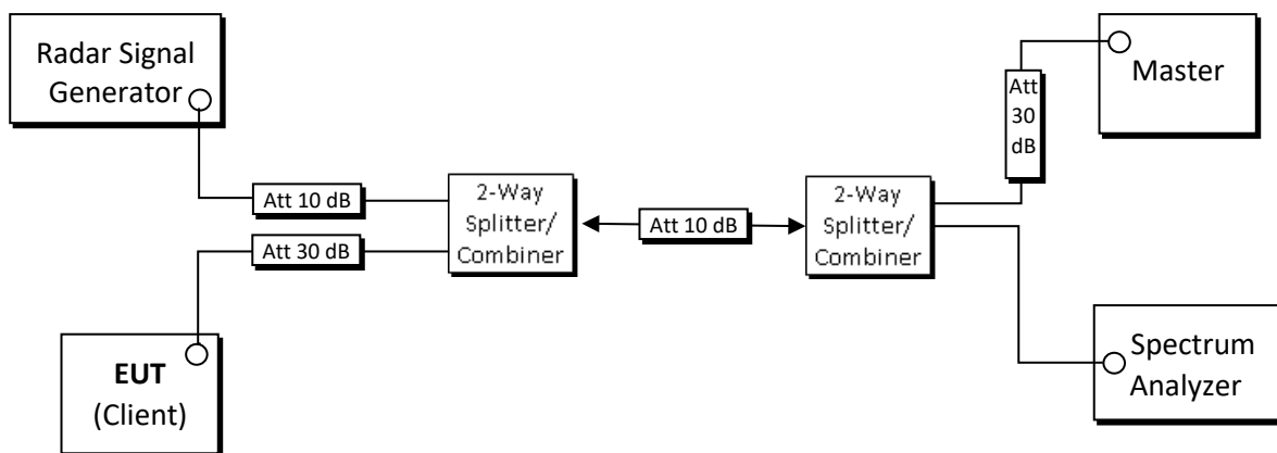
Figure 4-1. Conducted Test Setup for DFS
