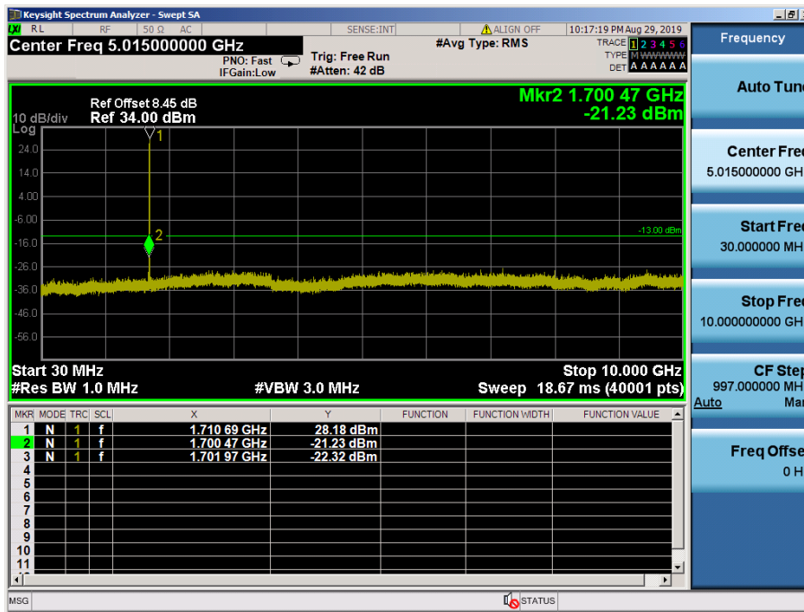
LTE Band 4 / 1.4MHz / QPSK - RB Size/Offset (8/0) – Low Channel
