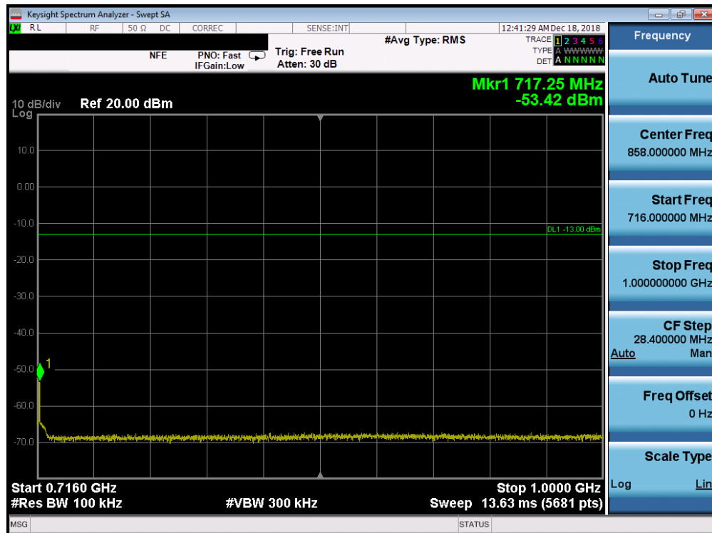
Plot 7-122. Conducted Spurious Plot (Band 12/17 - 10.0MHz QPSK - RB Size 1, RB Offset 0 - Low Channel)
