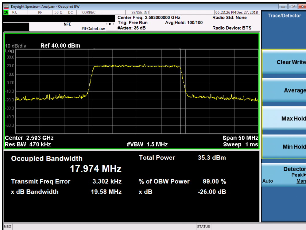
Plot 7-109. Occupied Bandwidth Plot (Band 41 PC2 - 20.0MHz QPSK - Full RB Configuration)
