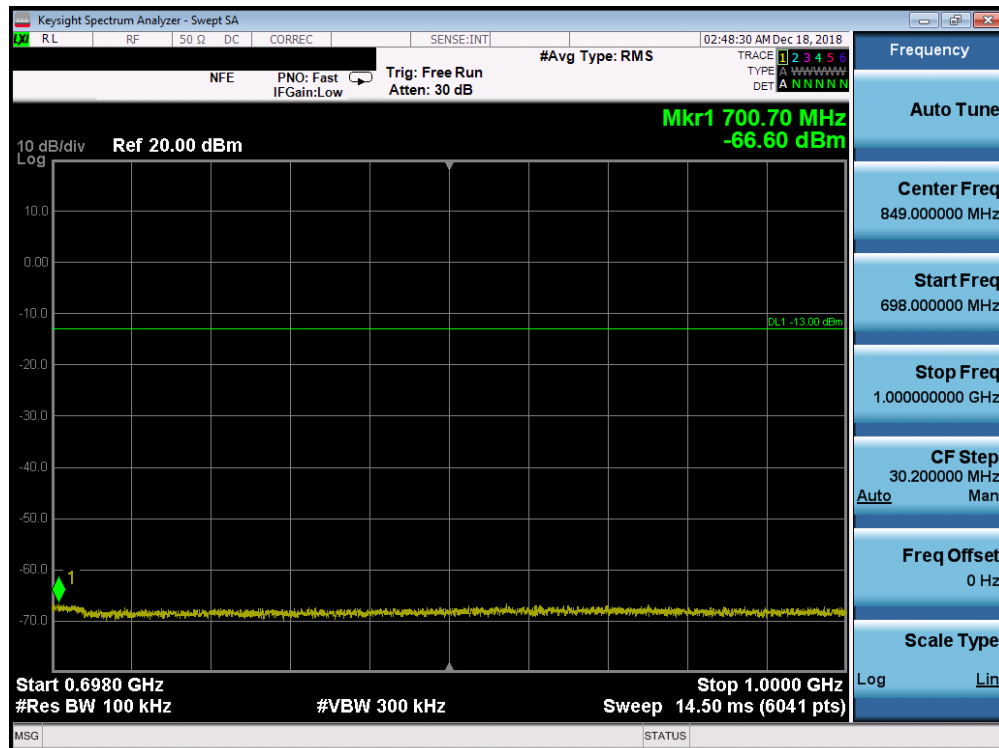
Plot 7-113. Conducted Spurious Plot (Band 71 - 15.0MHz QPSK - RB Size 1, RB Offset 0 - Low Channel)
