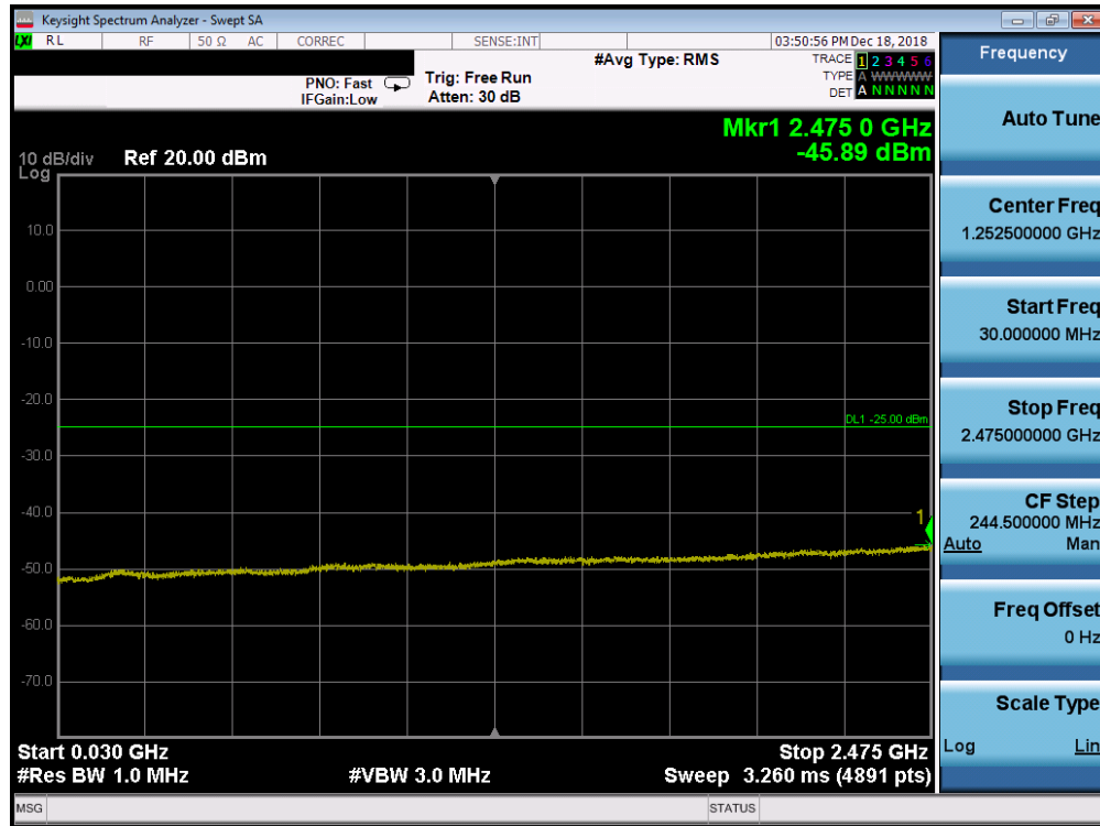
Plot 7-169. Conducted Spurious Plot (Band 7 - 20.0MHz QPSK - RB Size 1, RB Offset 0 - Low Channel)
