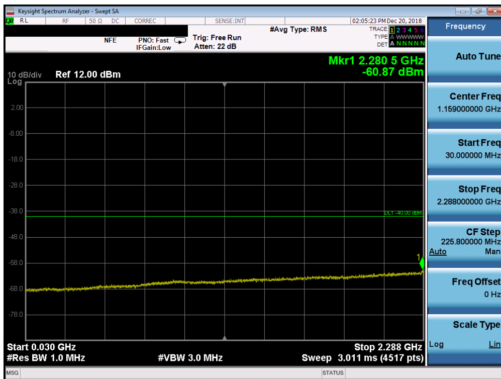
Plot 7-163. Conducted Spurious Plot (Band 30 - 5.0MHz QPSK - RB Size 1, RB Offset 0 - Mid Channel)
