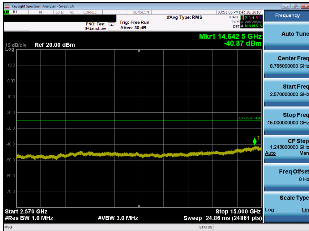
Plot 7-170. Conducted Spurious Plot (Band 7 - 20.0MHz QPSK - RB Size 1, RB Offset 0 - Low Channel)
