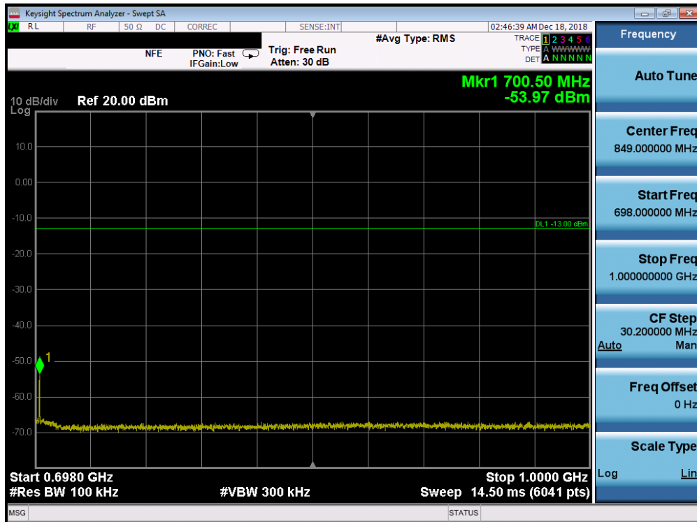
Plot 7-116. Conducted Spurious Plot (Band 71 - 15.0MHz QPSK - RB Size 1, RB Offset 0 - Mid Channel)
