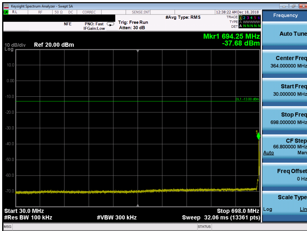
Plot 7-124. Conducted Spurious Plot (Band 12/17 - 10.0MHz QPSK - RB Size 1, RB Offset 0 - Mid Channel)
