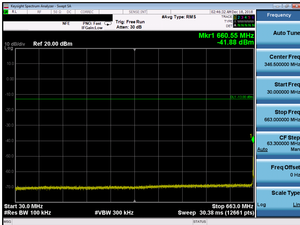
Plot 7-115. Conducted Spurious Plot (Band 71 - 15.0MHz QPSK - RB Size 1, RB Offset 0 - Mid Channel)
