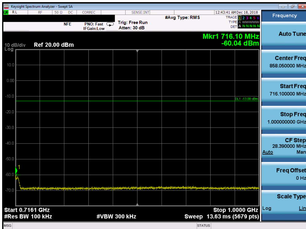
Plot 7-128. Conducted Spurious Plot (Band 12/17 - 10.0MHz QPSK - RB Size 1, RB Offset 0 - High Channel)
