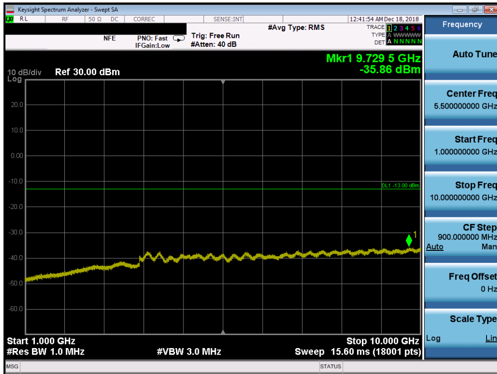
Plot 7-123. Conducted Spurious Plot (Band 12/17 - 10.0MHz QPSK - RB Size 1, RB Offset 0 - Low Channel)
