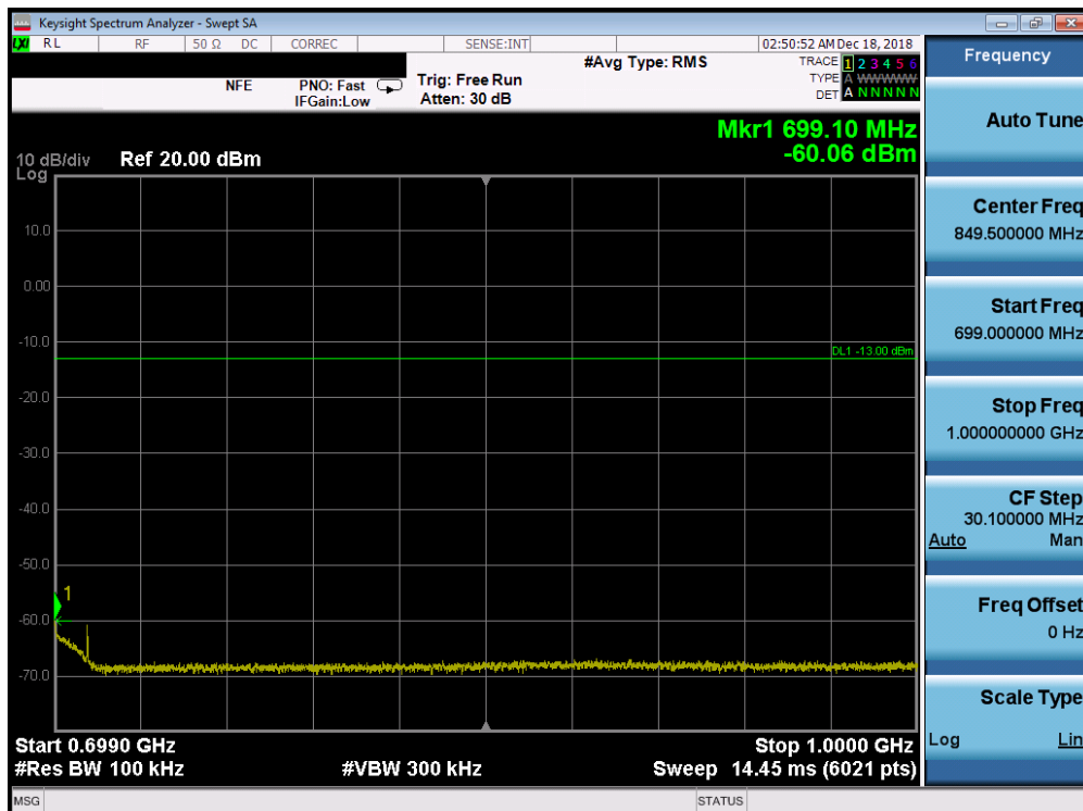
Plot 7-119. Conducted Spurious Plot (Band 71 - 15.0MHz QPSK - RB Size 1, RB Offset 0 - High Channel)
