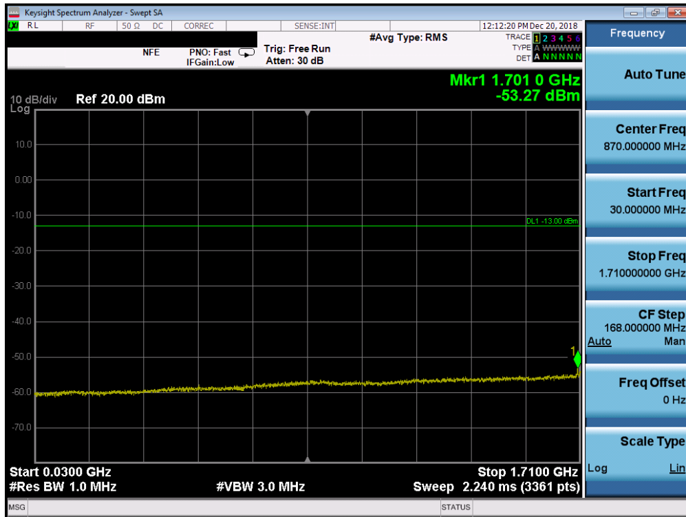
Plot 7-157. Conducted Spurious Plot (Band 25/2 - 20.0MHz QPSK - RB Size 1, RB Offset 0 - High Channel)
