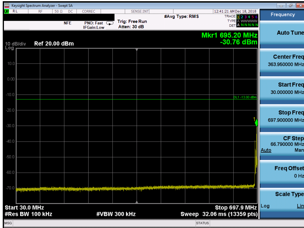
Plot 7-121. Conducted Spurious Plot (Band 12/17 - 10.0MHz QPSK - RB Size 1, RB Offset 0 - Low Channel)
