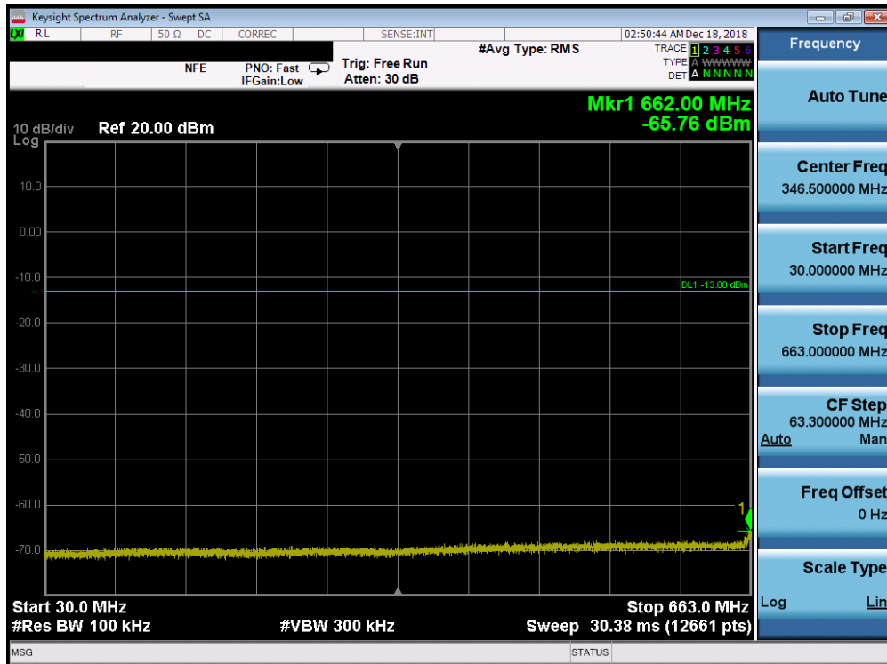
Plot 7-118. Conducted Spurious Plot (Band 71 - 15.0MHz QPSK - RB Size 1, RB Offset 0 - High Channel)
