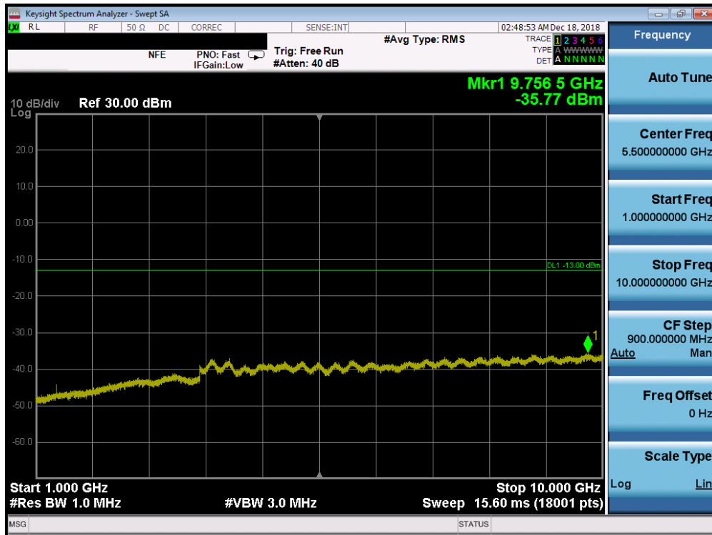
Plot 7-114. Conducted Spurious Plot (Band 71 - 15.0MHz QPSK - RB Size 1, RB Offset 0 - Low Channel)
