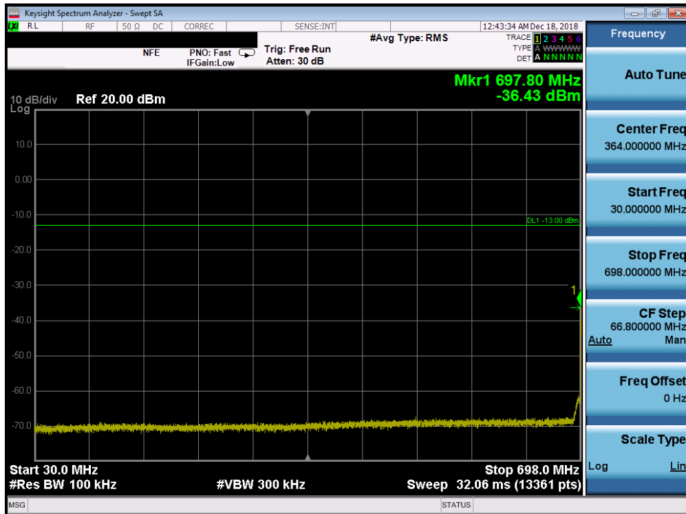
Plot 7-127. Conducted Spurious Plot (Band 12/17 - 10.0MHz QPSK - RB Size 1, RB Offset 0 - High Channel)
