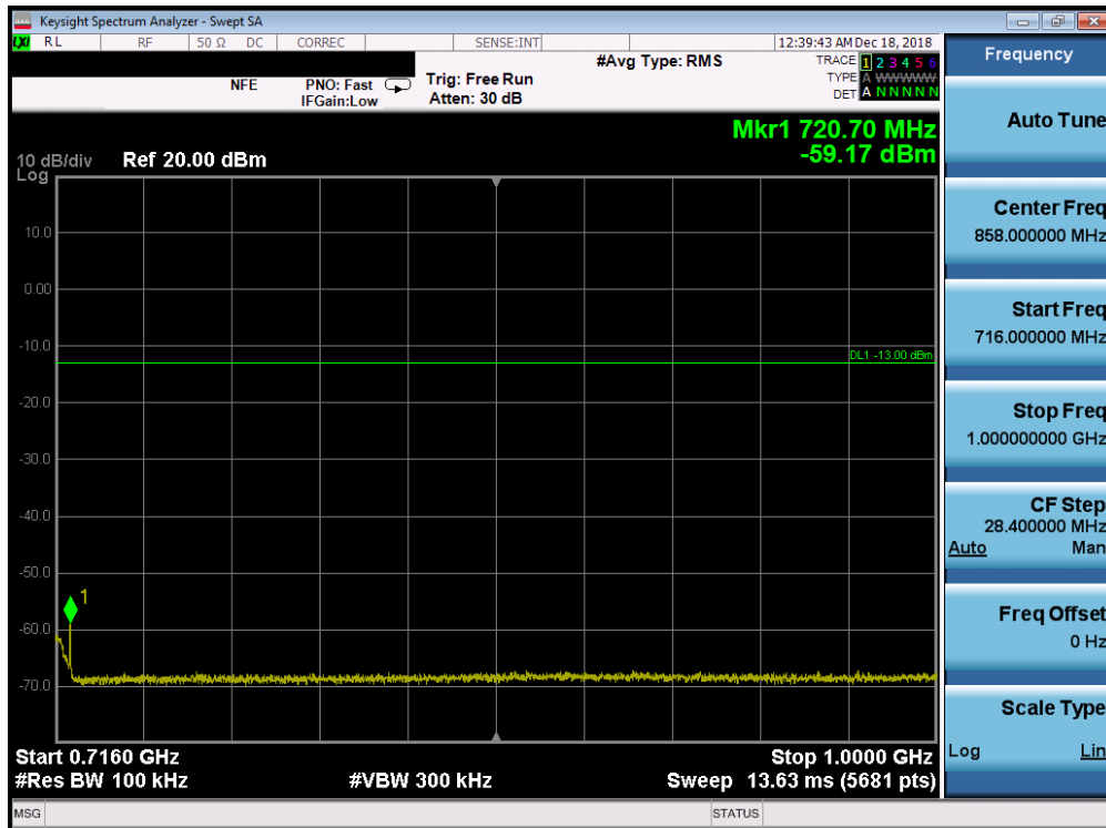
Plot 7-125. Conducted Spurious Plot (Band 12/17 - 10.0MHz QPSK - RB Size 1, RB Offset 0 - Mid Channel)
