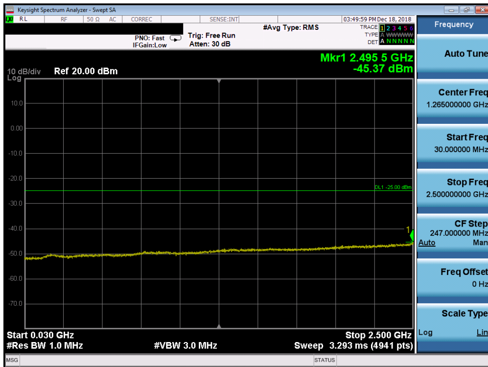
Plot 7-172. Conducted Spurious Plot (Band 7 - 20.0MHz QPSK - RB Size 1, RB Offset 0 - Mid Channel)
