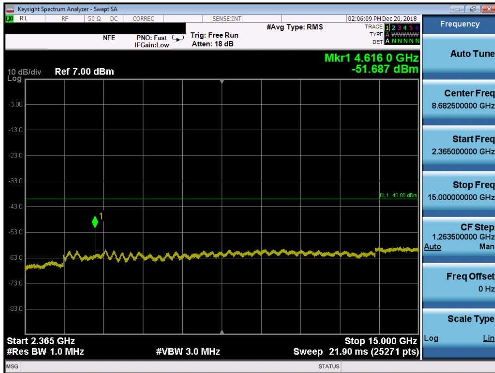
Plot 7-164. Conducted Spurious Plot (Band 30 - 5.0MHz QPSK - RB Size 1, RB Offset 0 - Mid Channel)
