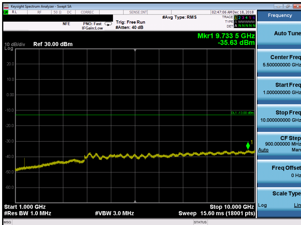
Plot 7-117. Conducted Spurious Plot (Band 71 - 15.0MHz QPSK - RB Size 1, RB Offset 0 - Mid Channel)
