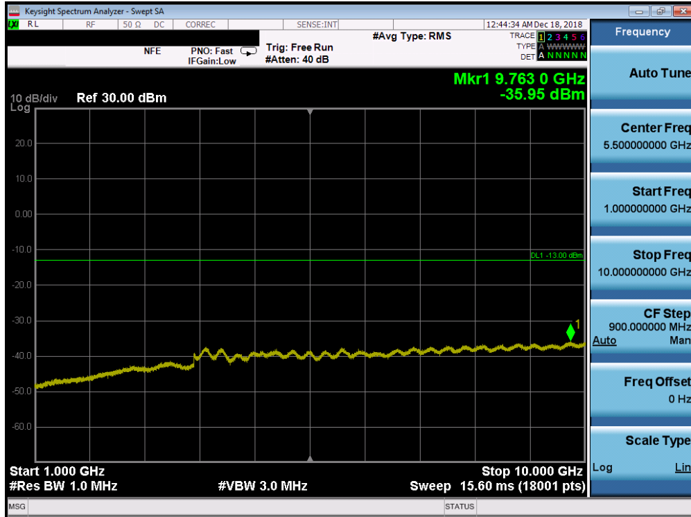
Plot 7-129. Conducted Spurious Plot (Band 12/17 - 10.0MHz QPSK - RB Size 1, RB Offset 0 - High Channel)
