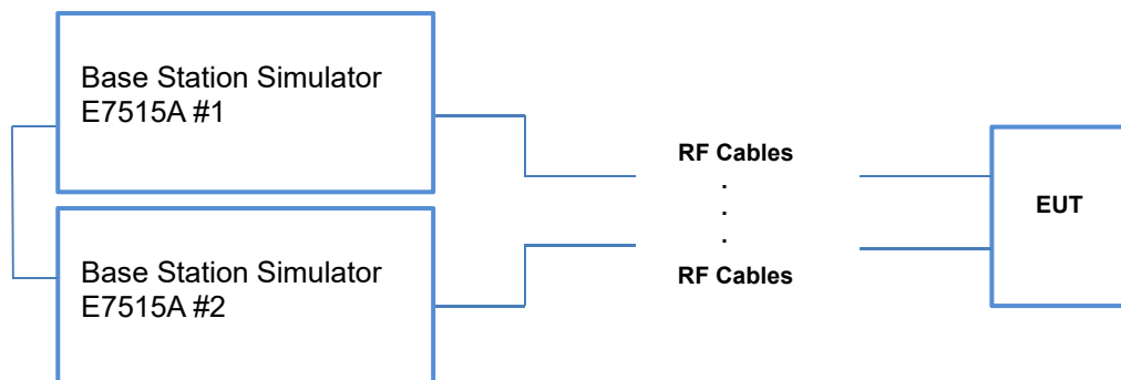
Figure G.3.1 DL 4x4 MIMO, DL 4x4 MIMO with DL 4CA Power Measurement Setup
