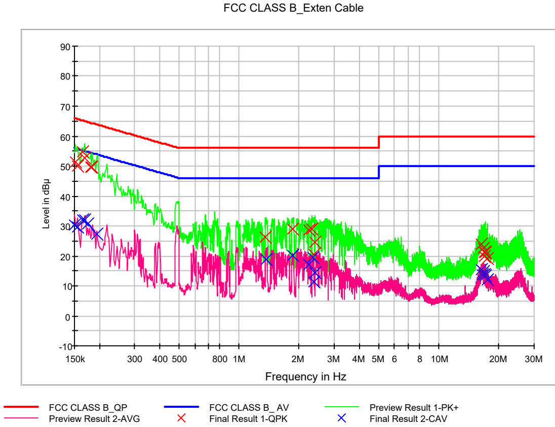
Figure 4: Conducted Emission, AC Main Port, Line (N)
