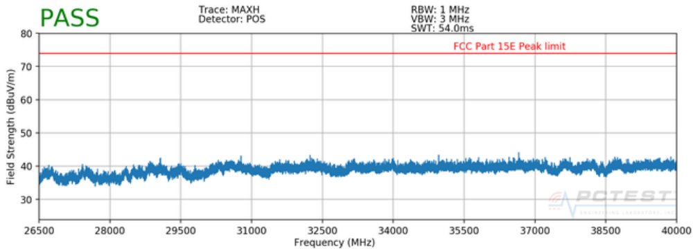
Plot 7-15. Radiated Spurious Plot above 26.5GHz (Simultaneous Transmission Config-1)
