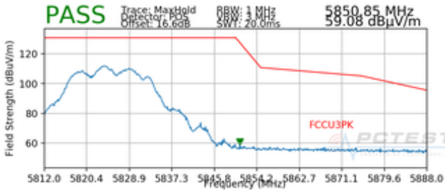
Plot 7-103. Radiated Upper Band Edge Plot MIMO (Peak – UNII Band 3)
