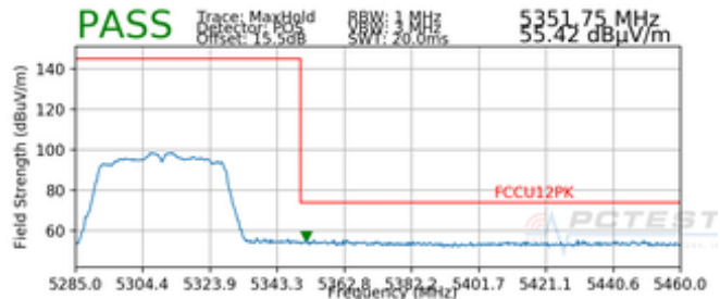
Plot 7-28. Radiated Upper Band Edge Plot SISO ANT1 (Peak – UNII Band 2A)
