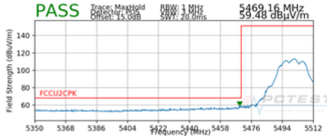
Plot 7-102. Radiated Lower Band Edge Plot MIMO (Peak – UNII Band 2C)
