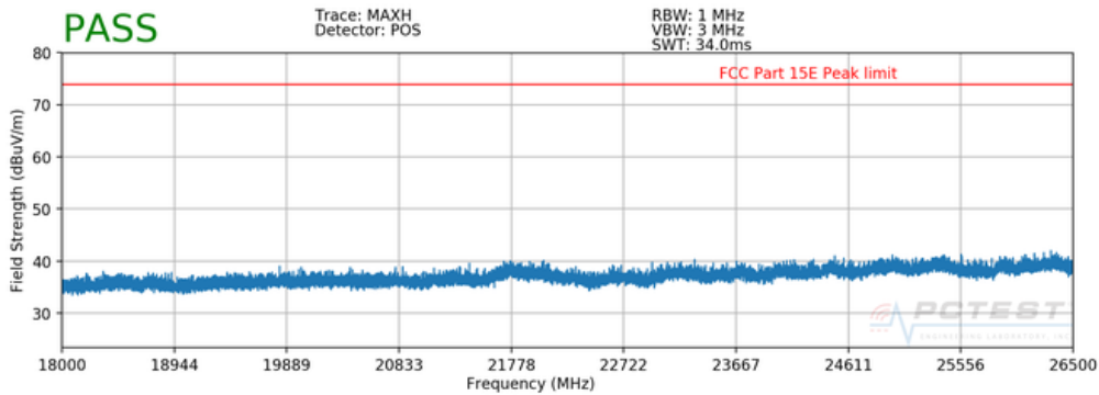
Plot 7-14. Radiated Spurious Plot 18GHz – 26.5GHz (Simultaneous Transmission Config-1)
