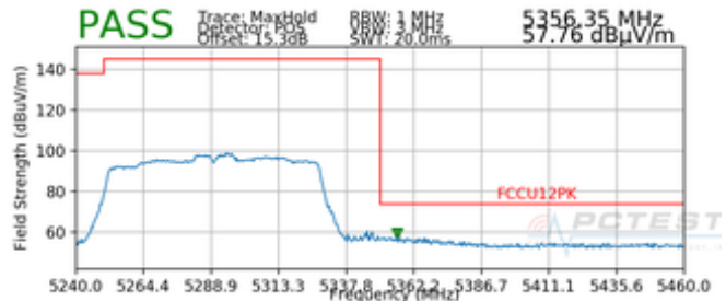
Plot 7-64. Radiated Upper Band Edge Plot SISO ANT2 (Peak – UNII Band 2A)
