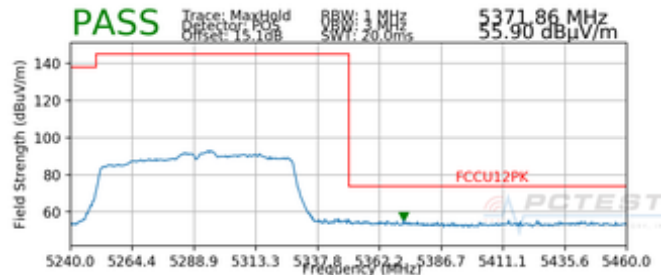
Plot 7-37. Radiated Upper Band Edge Plot SISO ANT1 (Peak – UNII Band 2A)
