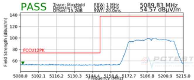
Plot 7-26. Radiated Lower Band Edge Plot SISO ANT1 (Peak – UNII Band 1)
