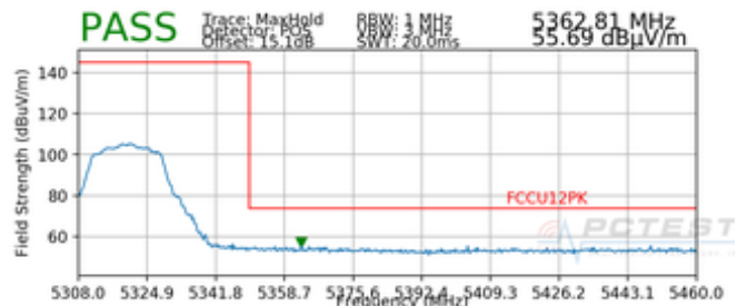
Plot 7-19. Radiated Upper Band Edge Plot SISO ANT1 (Peak – UNII Band 2A)
