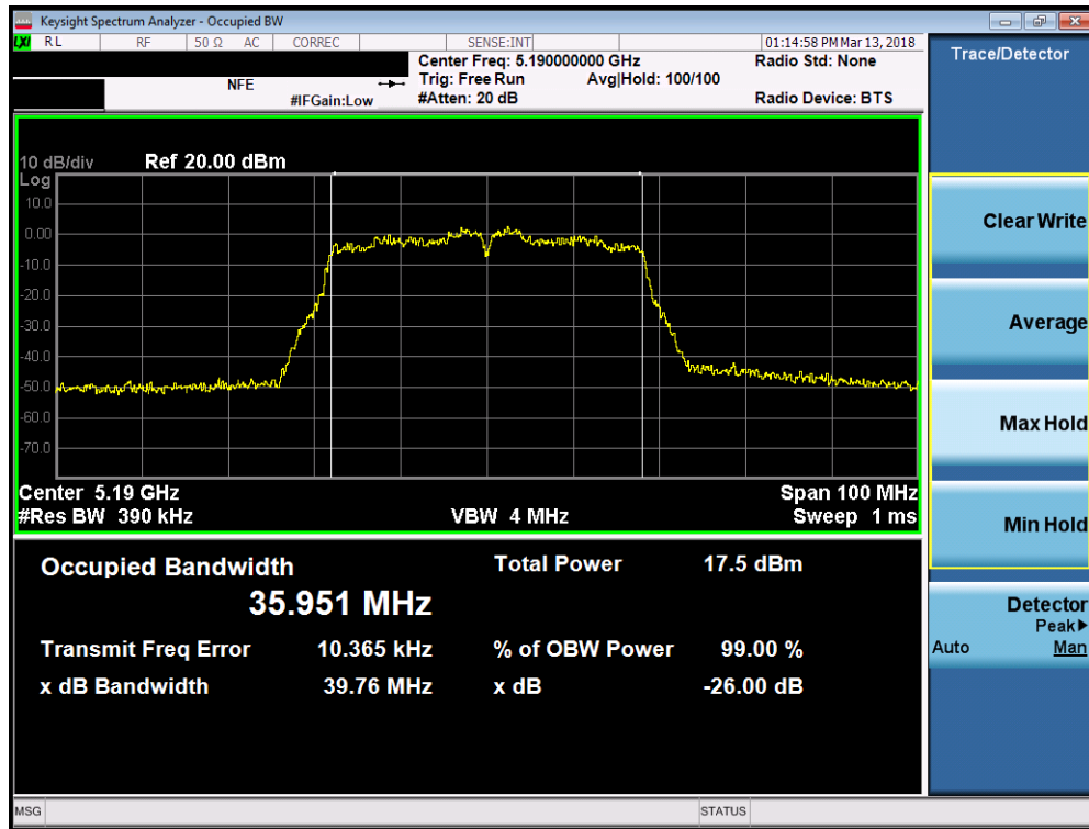
Plot 7-36. 26dB Bandwidth Plot (40MHz BW 802.11n (UNII Band 1) – Ch. 38)
