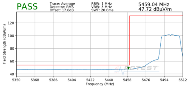
Plot 7-19. Radiated Lower Band Edge Plot MIMO (Average – UNII Band 2C)
