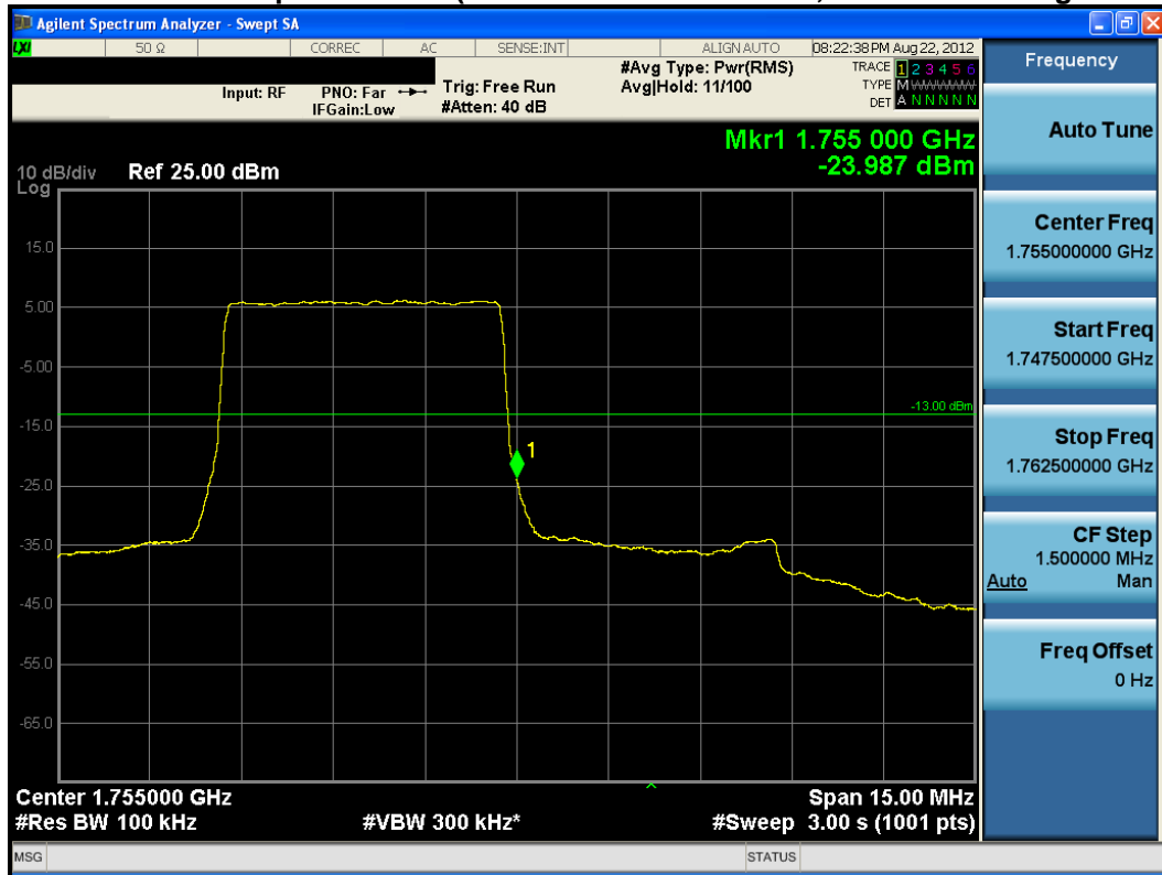
Plot 9-19. Upper Band Edge Plot (5MHz QPSK – RB Size 25)
