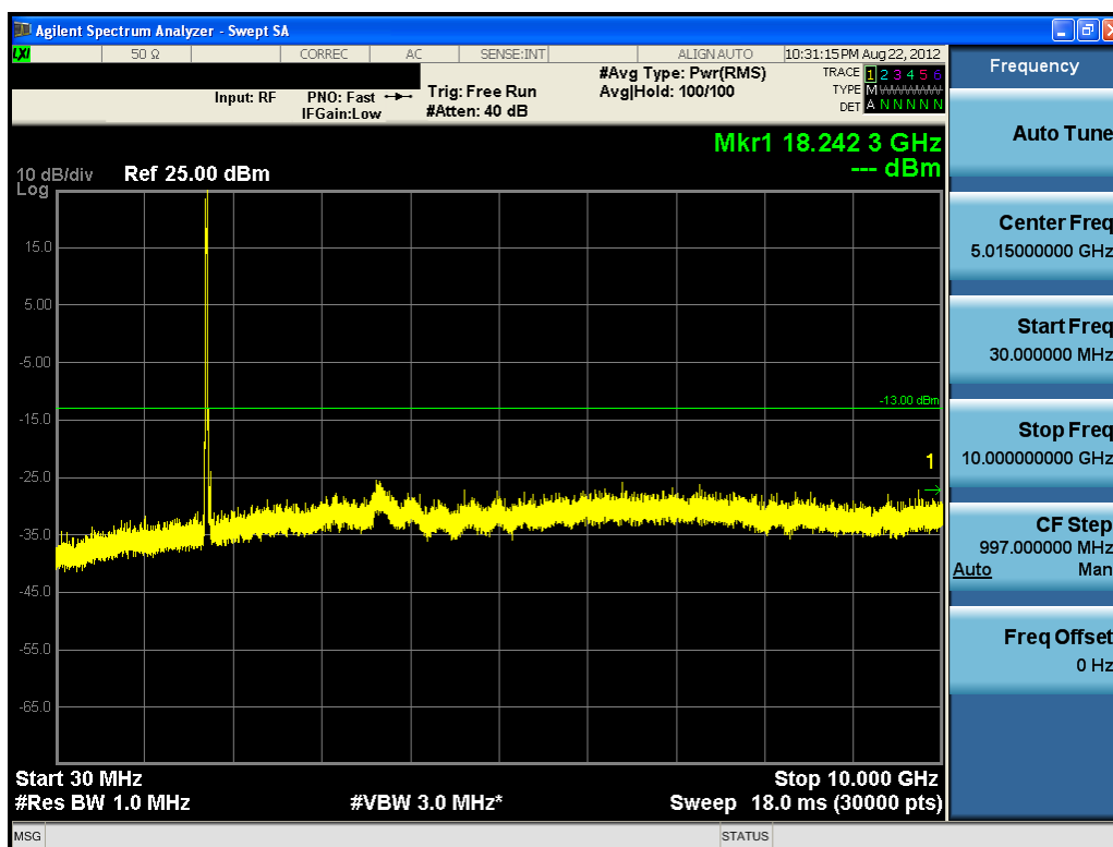
Plot 9-38. Conducted Spurious Plot (QPSK – RB Size 1, RB Offset 0 – Low Channel)
