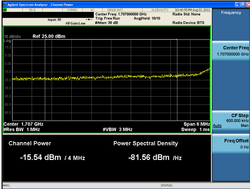
Plot 9-32. Lower Ext. Band Edge Plot (QPSK – RB Size 100)
