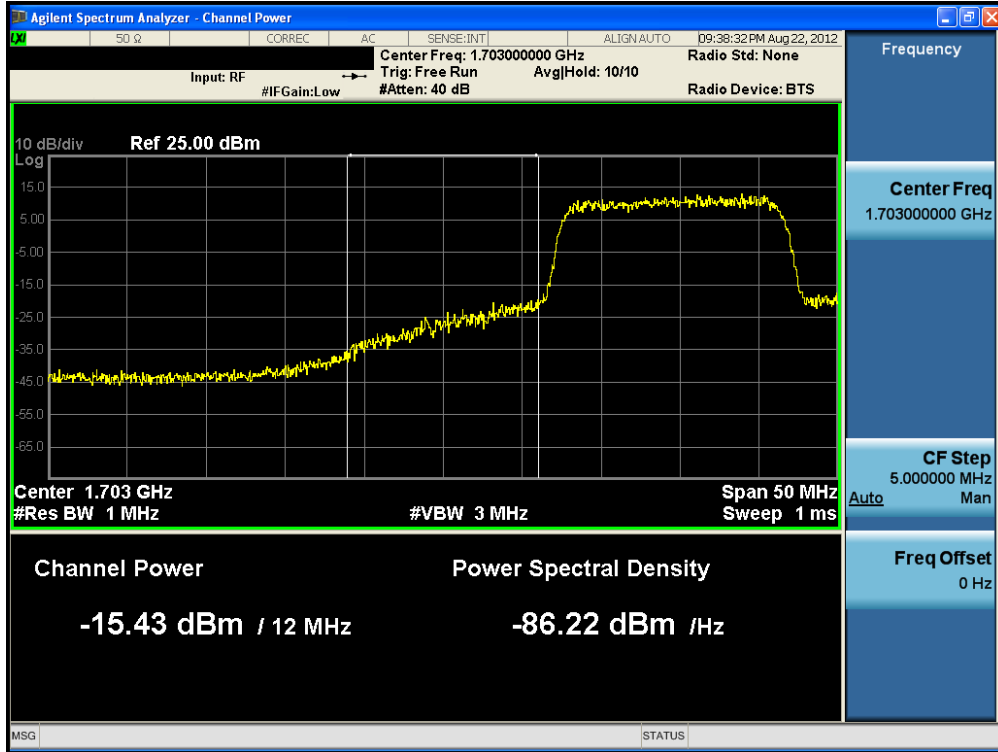
Plot 9-6. Lower Extended Band Edge Plot (15MHz QPSK- RB Size 75)
