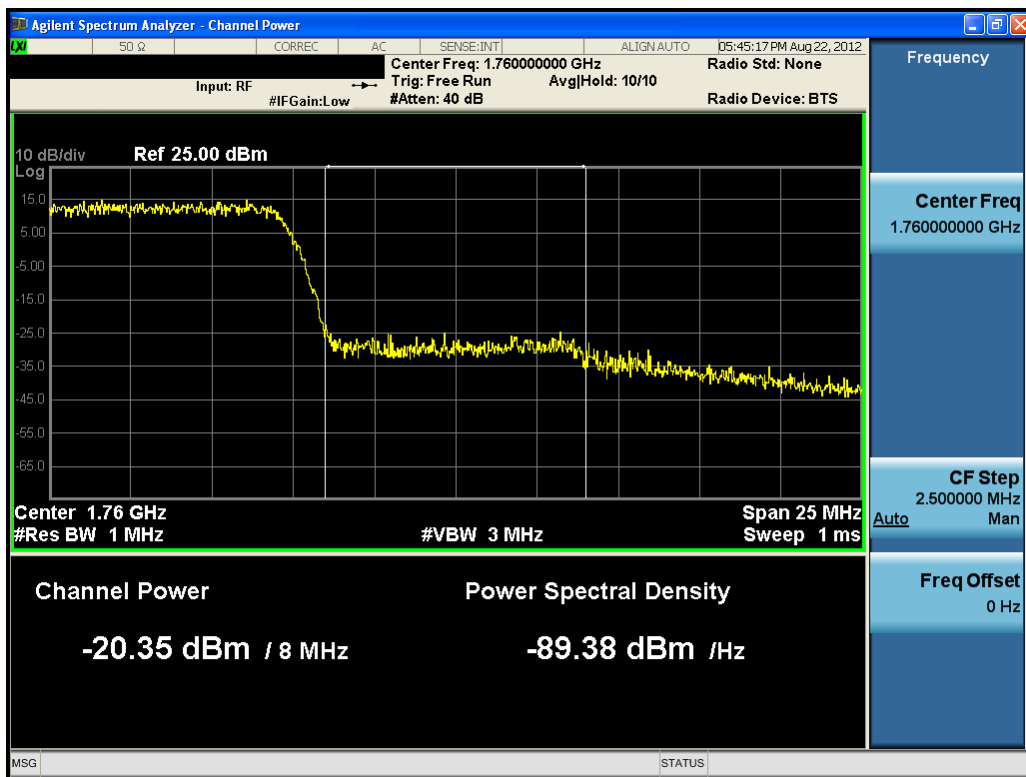
Plot 9-23. Upper Extended Band Edge Plot (10MHz QPSK– RB Size 50)
