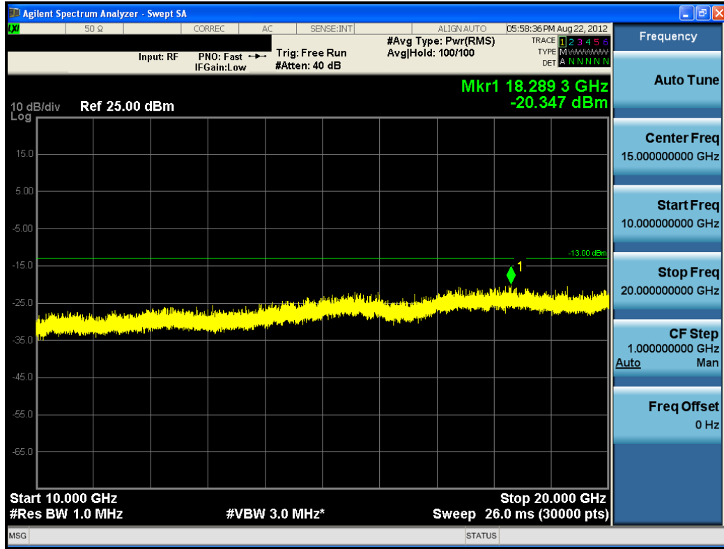
Plot 9-16. Conducted Spurious Plot (10MHz QPSK – RB Size 1, RB Offset 0 – Mid Channel)
