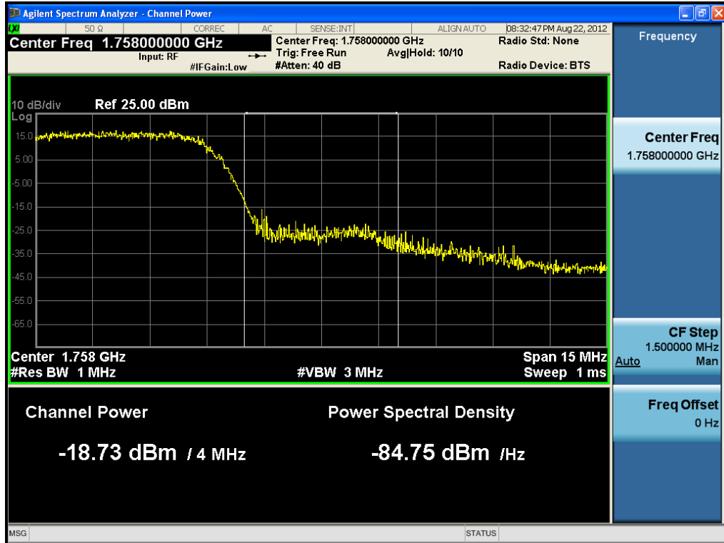
Plot 9-22. Upper Extended Band Edge Plot (5MHz QPSK– RB Size 25)
