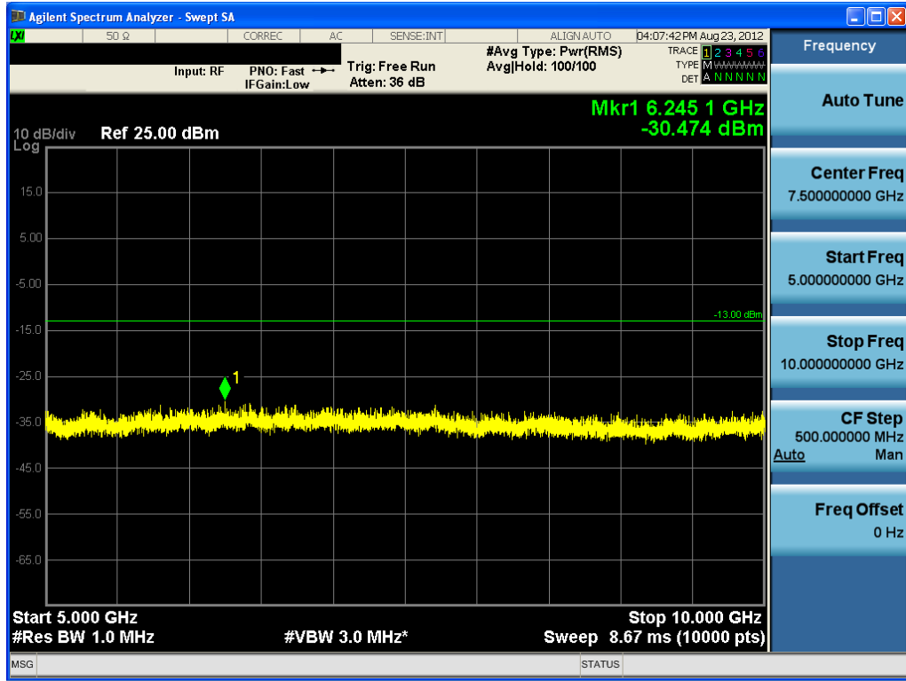
Plot 8-14. Conducted Spurious Plot (50MHz QPSK – RB Size 1, RB Offset 0 – High Channel)
