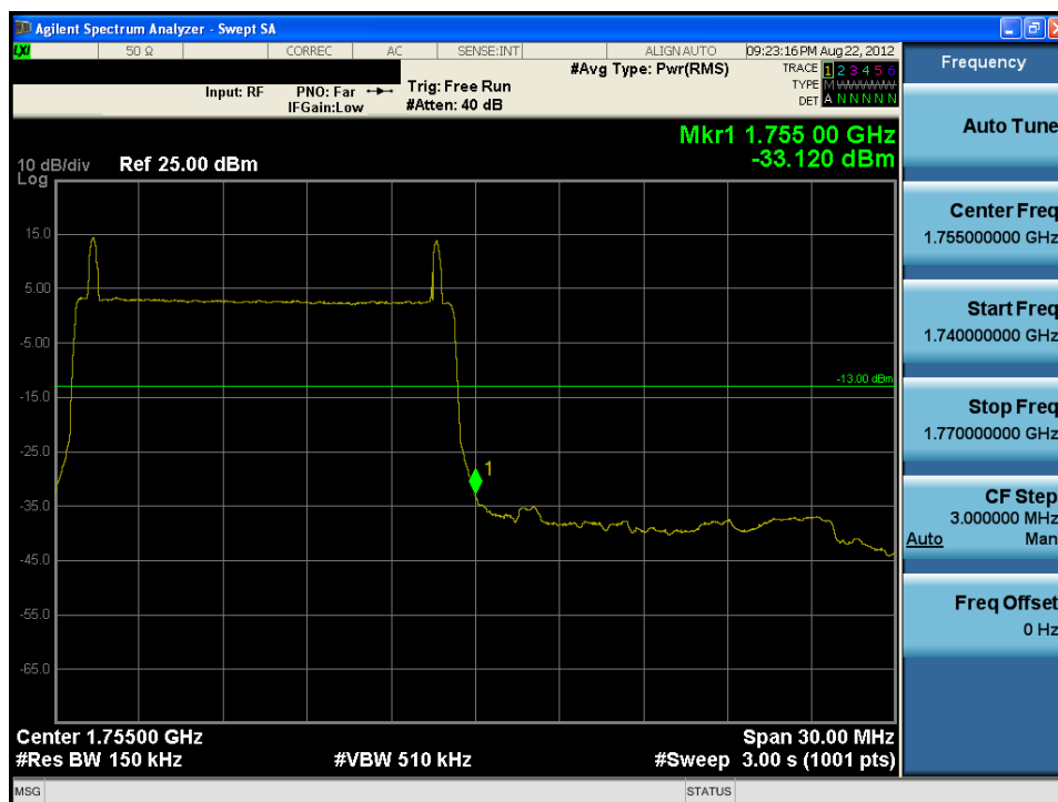
Plot 9-21. Upper Band Edge Plot (15MHz QPSK – RB Size 75)
