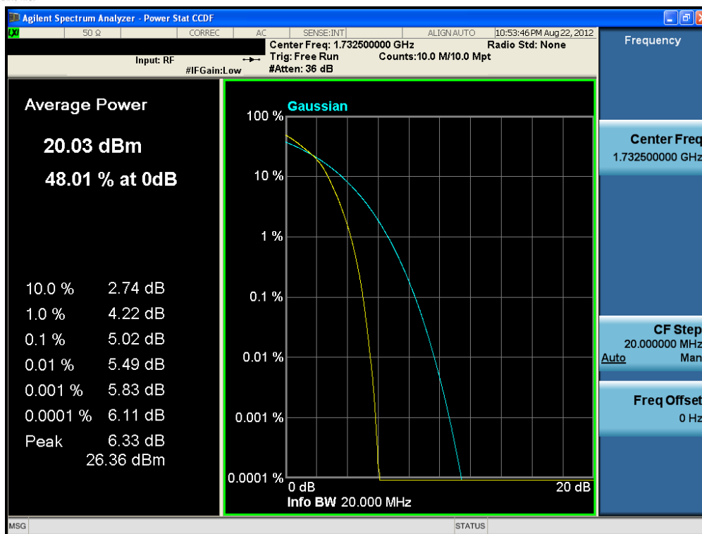
Plot 9-37. Peak to Average Ratio Plot (16QAM – RB Size 100)
