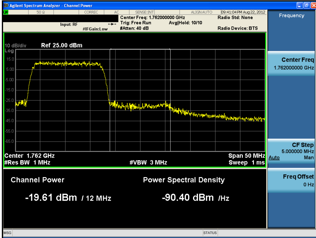
Plot 9-24. Upper Extended Band Edge Plot (15MHz QPSK– RB Size 75, Offset 0)
