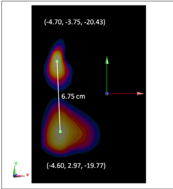
Figure 13-3 Peak SAR Location Plot of LTE Band 4 (AWS) and 2.4 GHz WLAN
